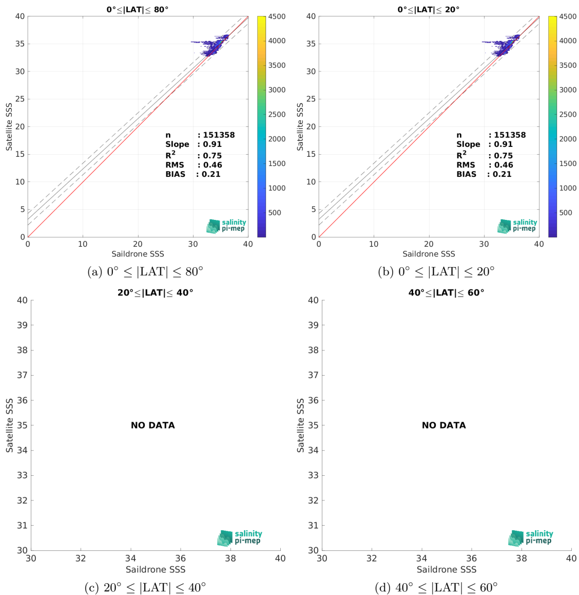
Figure 10: Contour maps of the concentration of SMAP SSS L3 v5.0 - Monthly (JPL) SSS (y-axis) versus Sairdron SSS (x-axis) at match-up pairs for different latitude bands. For each plot, the red line shows x=y . The black thin and dashed lines indicate a linear fit through the data cloud and the \pm 95\% confidence levels, respectively. The number match-up pairs n , the slope and R^2 coefficient of the linear fit, the root mean square (RMS) and the mean bias between satellite and in situ data are indicated for each latitude band in each plots.
