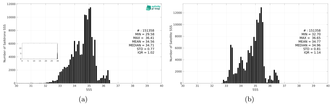
Figure 3: Histograms of SSS from Saildrone (a) and SMAP SSS L3 v5.0 - Monthly (JPL) (b) considering all match-up pairs per bins of 0.1 over the Equatorial Ocean 10N-10S Pi-MEP region and for the full satellite product period.
