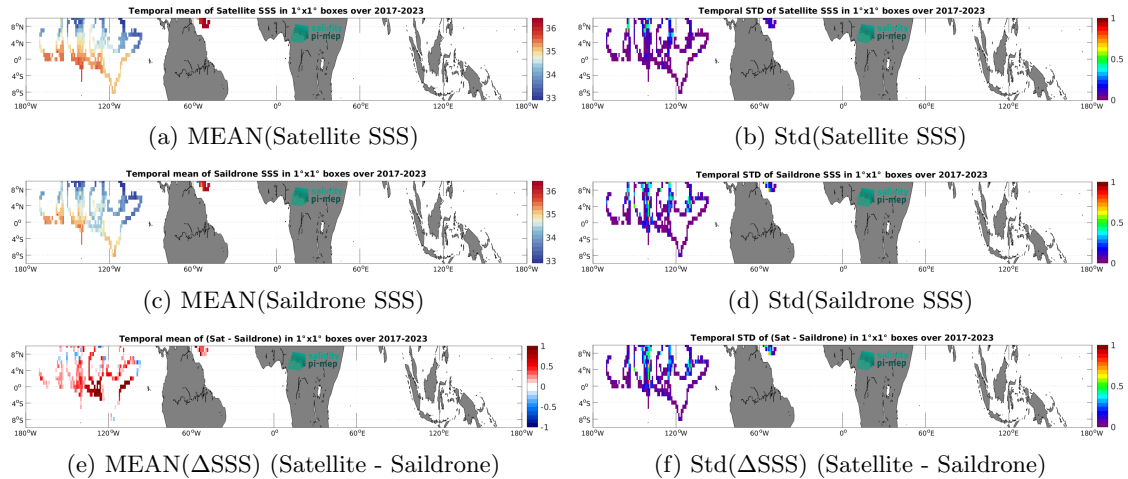
Figure 7: Temporal mean (left) and Std (right) of SSS from SMAP SSS L3 v5.0 - Monthly (JPL) (top), Saildrone (middle), and of \Delta SSS (Satellite - Saildrone). Only match-up pairs are used to generate these maps.
