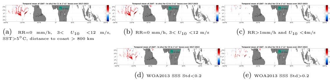
Figure 14: Temporal mean gridded over spatial boxes of size 1^\circ \times 1^\circ of \Delta SSS (SMAP SSS L3 v5.0 - Monthly (JPL) - Saildrone) for 5 different subdatasets corresponding to:RR=0 mm/h, 3 < U_{10} < 12 m/s, SST>5°C, distance to coast > 800 km (a), RR=0 mm/h, 3 < U_{10} < 12 m/s (b), RR>1mm/h and U_{10} < 4 m/s (c), WOA2013 SSS Std<0.2 (d), WOA2013 SSS Std>0.2 (e).
