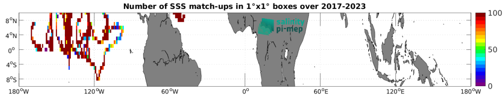
Figure 5: Number of SSS match-ups between Saildrone SSS and the SMAP SSS L3 v5.0 - Monthly (JPL) SSS product for the Equatorial Ocean 10N-10S Pi-MEP region over 1^\circ \times 1^\circ boxes and for the full satellite product period.
