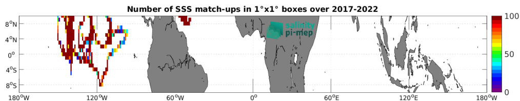
Figure 5: Number of SSS match-ups between Sairdroner SSS and the SMAP SSS L3 v5.0 - Monthly (JPL) SSS product for the Equatorial Ocean 10N-10S Pi-MEP region over 1^\circ \times 1^\circ boxes and for the full satellite product period.
