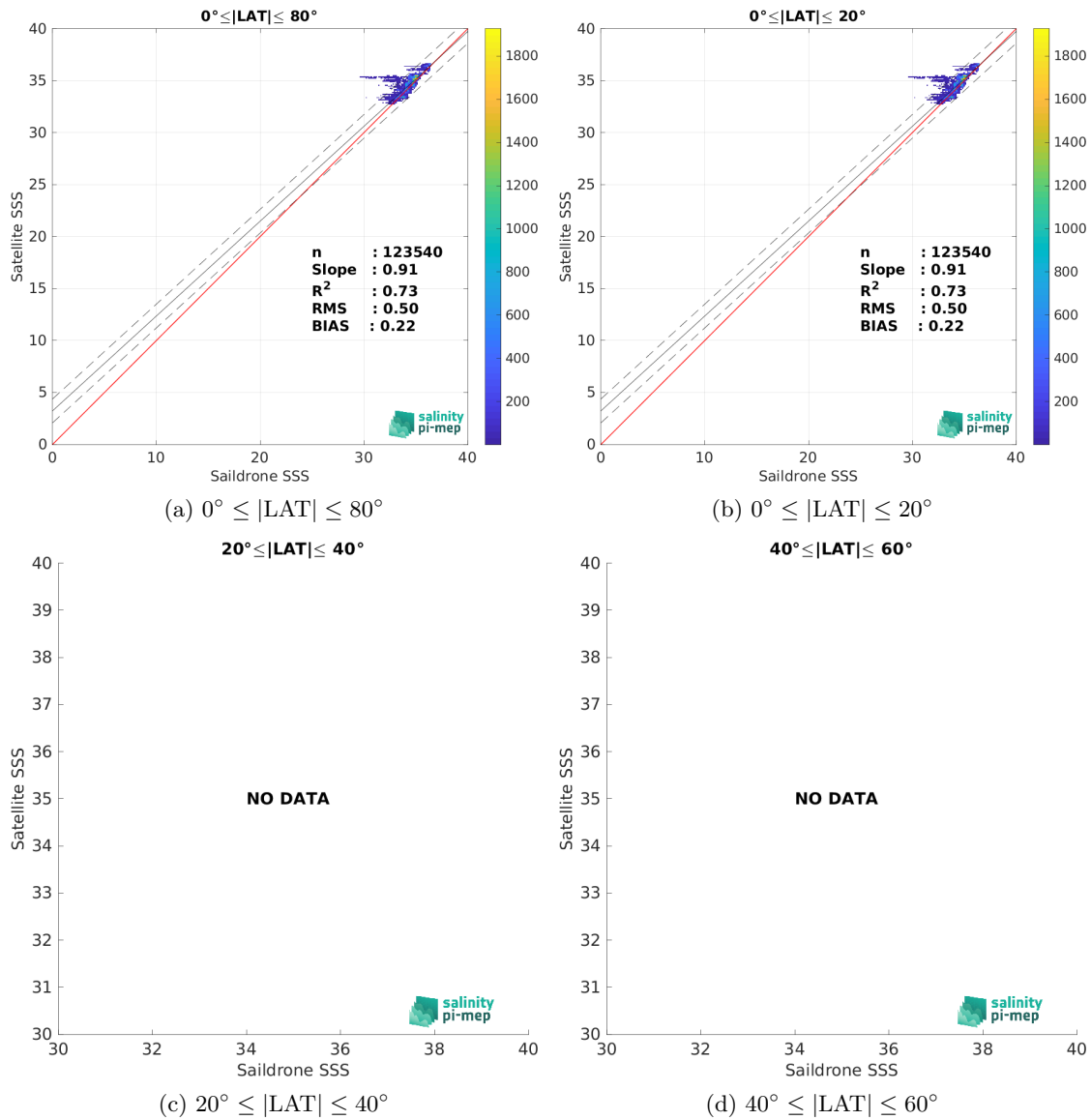
Figure 10: Contour maps of the concentration of SMAP SSS L3 v5.0 - Monthly (JPL) SSS (y-axis) versus Sairdrone SSS (x-axis) at match-up pairs for different latitude bands. For each plot, the red line shows x=y . The black thin and dashed lines indicate a linear fit through the data cloud and the \pm 95\% confidence levels, respectively. The number match-up pairs n , the slope and R^2 coefficient of the linear fit, the root mean square (RMS) and the mean bias between satellite and in situ data are indicated for each latitude band in each plots.
