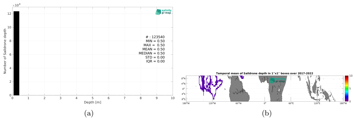
Figure 4: Histograms of the depth of the upper level SSS measurements from Sairdroner in the Match-up DataBase for the Equatorial Ocean 10N-10S Pi-MEP region (a) and temporal mean spatial distribution of pressure of the in situ SSS data over 1^\circ \times 1^\circ boxes and for the full satellite product period (b).
