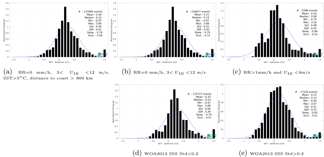
Figure 13: Normalized histogram of \Delta SSS (SMAP SSS L3 v5.0 - Monthly (JPL) - Saildrone) for 5 different subdatasets corresponding to: RR=0 mm/h, 3 < U_{10} < 12 m/s, SST > 5^\circ\text{C} , distance to coast > 800 km (a), RR=0 mm/h, 3 < U_{10} < 12 m/s (b), RR > 1 mm/h and U_{10} < 4 m/s (c), WOA2013 SSS Std < 0.2 (d), WOA2013 SSS Std > 0.2 (e).
