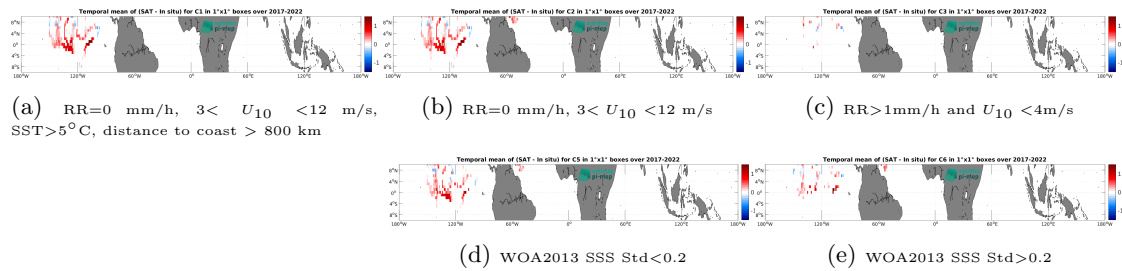
Figure 12: Temporal mean gridded over spatial boxes of size 1^\circ \times 1^\circ of \Delta SSS (SMAP SSS L3 v5.0 - Monthly (JPL) - Saildrone) for 5 different subdatasets corresponding to: RR=0 mm/h, 3 < U_{10} < 12 m/s, SST > 5^\circ\text{C} , distance to coast > 800 km (a), RR=0 mm/h, 3 < U_{10} < 12 m/s (b), RR > 1 mm/h and U_{10} < 4 m/s (c), WOA2013 SSS Std < 0.2 (d), WOA2013 SSS Std > 0.2 (e).
