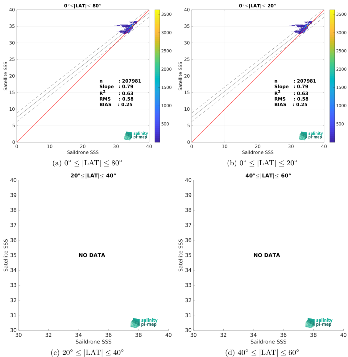
Figure 9: Contour maps of the concentration of SMAP SSS L3 v5.0 - Monthly (JPL) SSS (y-axis) versus Sairdrone SSS (x-axis) at match-up pairs for different latitude bands. For each plot, the red line shows x=y . The black thin and dashed lines indicate a linear fit through the data cloud and the \pm 95\% confidence levels, respectively. The number match-up pairs n , the slope and R^2 coefficient of the linear fit, the root mean square (RMS) and the mean bias between satellite and in situ data are indicated for each latitude band in each plots.
