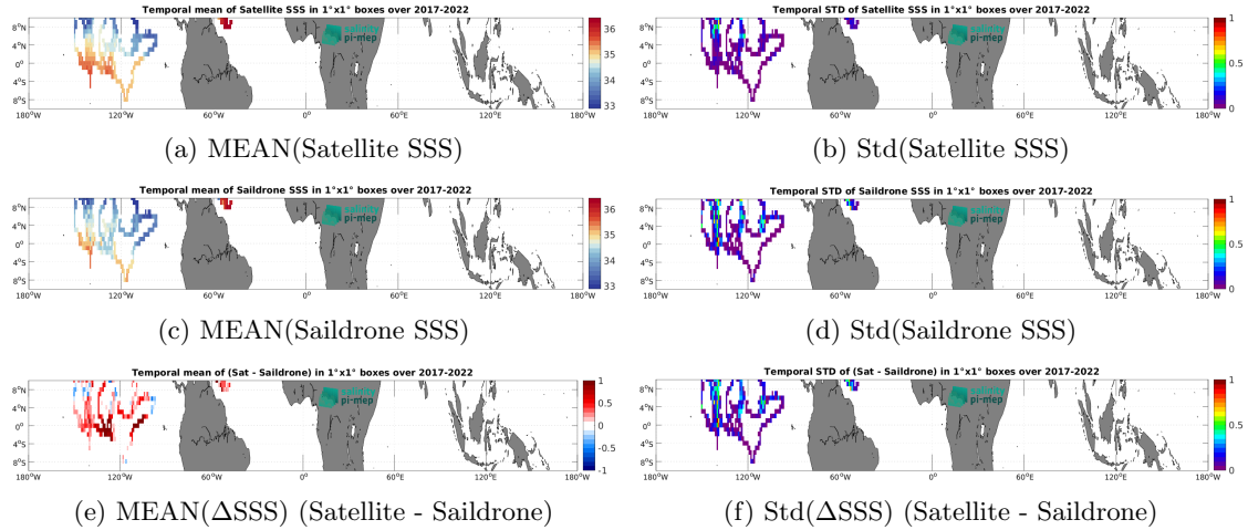
Figure 6: Temporal mean (left) and Std (right) of SSS from SMAP SSS L3 v5.0 - Monthly (JPL) (top), Saildrone (middle), and of \Delta SSS (Satellite - Saildrone). Only match-up pairs are used to generate these maps.
