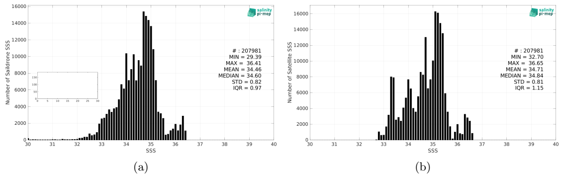
Figure 2: Histograms of SSS from Saildrone (a) and SMAP SSS L3 v5.0 - Monthly (JPL) (b) considering all match-up pairs per bins of 0.1 over the Equatorial Ocean 10N-10S Pi-MEP region and for the full satellite product period.
