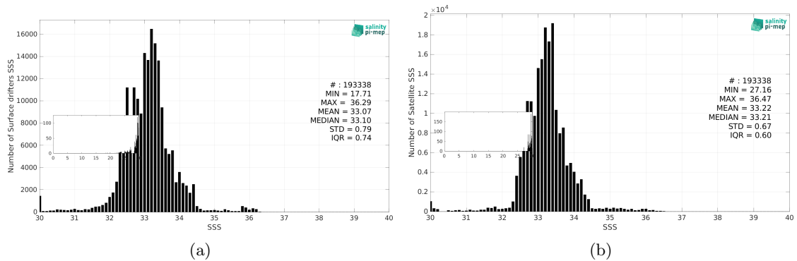
Figure 3: Histograms of SSS from Surface drifters (a) and SMAP SSS L3 v5.0 - Monthly (JPL) (b) considering all match-up pairs per bins of 0.1 over the Equatorial Ocean 10N-10S Pi-MEP region and for the full satellite product period.
