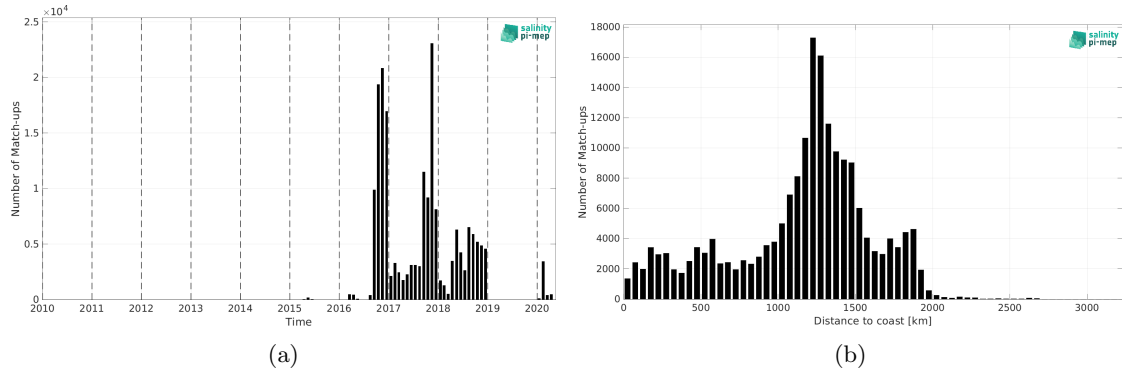
Figure 2: Number of match-ups between Surface drifters and SMAP SSS L3 v5.0 - Monthly (JPL) SSS as a function of time (a) and as function of the distance to coast (b) over the Equatorial Ocean 10N-10S Pi-MEP region and for the full satellite product period.
