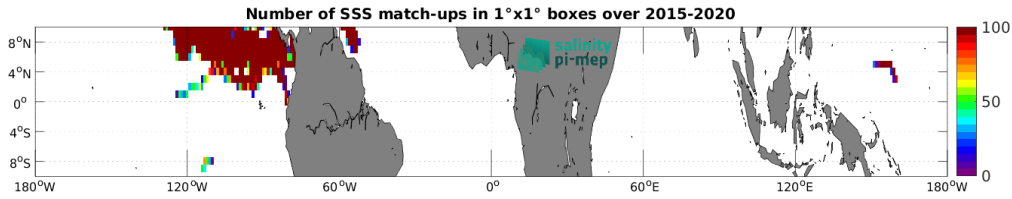
Figure 4: Number of SSS match-ups between Surface drifters SSS and the SMAP SSS L3 v5.0 - Monthly (JPL) SSS product for the Equatorial Ocean 10N-10S Pi-MEP region over 1^\circ \times 1^\circ boxes and for the full satellite product period.
