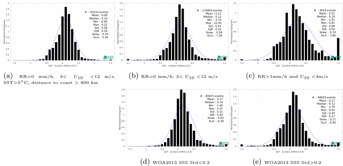
Figure 14: Normalized histogram of \Delta SSS (SMAP SSS L3 v5.0 - Monthly (JPL) - Surface drifters) for 5 different subdatasets corresponding to: RR=0 mm/h, 3 < U_{10} < 12 m/s, SST >5^\circ C, distance to coast > 800 km (a), RR=0 mm/h, 3 < U_{10} < 12 m/s (b), RR >1 mm/h and U_{10} < 4 m/s (c), WOA2013 SSS Std <0.2 (d), WOA2013 SSS Std >0.2 (e).
