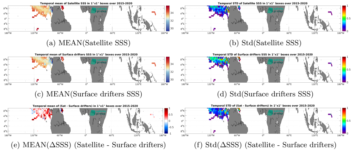
Figure 6: Temporal mean (left) and Std (right) of SSS from SMAP SSS L3 v5.0 - Monthly (JPL) (top), Surface drifters (middle), and of \Delta SSS (Satellite - Surface drifters). Only match-up pairs are used to generate these maps.
