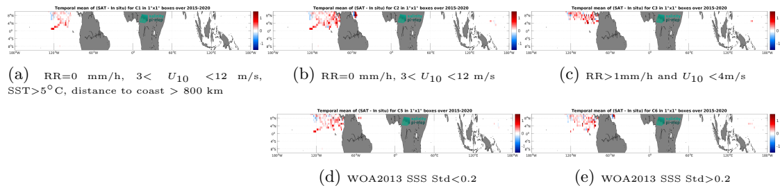
Figure 13: Temporal mean gridded over spatial boxes of size 1^\circ \times 1^\circ of \Delta SSS (SMAP SSS L3 v5.0 - Monthly (JPL) - Surface drifters) for 5 different subdatasets corresponding to:RR=0 mm/h, 3 < U_{10} < 12 m/s, SST >5^\circ C, distance to coast > 800 km (a), RR=0 mm/h, 3 < U_{10} < 12 m/s (b), RR >1 mm/h and U_{10} < 4 m/s (c), WOA2013 SSS Std <0.2 (d), WOA2013 SSS Std >0.2 (e).
