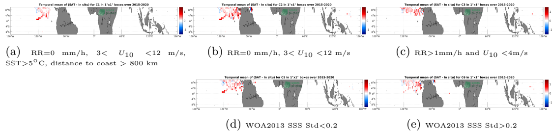
Figure 11: Temporal mean gridded over spatial boxes of size 1^\circ \times 1^\circ of \Delta SSS (SMAP SSS L3 v5.0 - Monthly (JPL) - Surface drifters) for 5 different subdatasets corresponding to:RR=0 mm/h, 3 < U_{10} < 12 m/s, SST > 5^\circ C , distance to coast > 800 km (a), RR=0 mm/h, 3 < U_{10} < 12 m/s (b), RR>1mm/h and U_{10} < 4 m/s (c), WOA2013 SSS Std<0.2 (d), WOA2013 SSS Std>0.2 (e).
