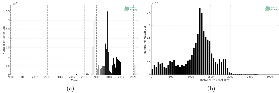
Figure 1: Number of match-ups between Surface drifters and SMAP SSS L3 v5.0 - Monthly (JPL) SSS as a function of time (a) and as function of the distance to coast (b) over the Equatorial Ocean 10N-10S Pi-MEP region and for the full satellite product period.
