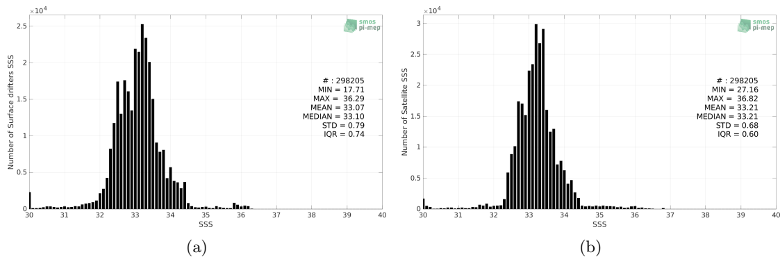
Figure 2: Histograms of SSS from Surface drifters (a) and SMAP SSS L3 v5.0 - Monthly (JPL) (b) considering all match-up pairs per bins of 0.1 over the Equatorial Ocean 10N-10S Pi-MEP region and for the full satellite product period.
