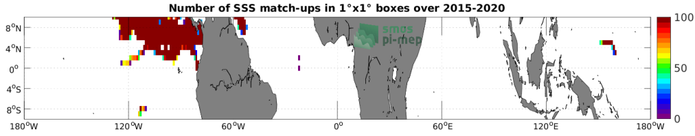
Figure 3: Number of SSS match-ups between Surface drifters SSS and the SMAP SSS L3 v5.0 - Monthly (JPL) SSS product for the Equatorial Ocean 10N-10S Pi-MEP region over 1^\circ \times 1^\circ boxes and for the full satellite product period.
