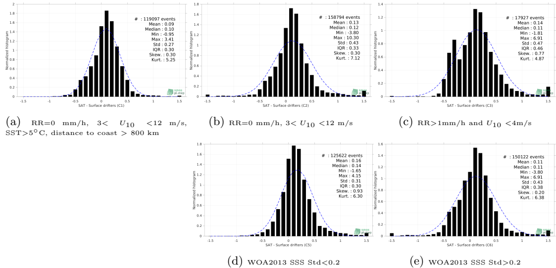
Figure 12: Normalized histogram of \Delta SSS (SMAP SSS L3 v5.0 - Monthly (JPL) - Surface drifters) for 5 different subdatasets corresponding to: RR=0 mm/h, 3 < U_{10} < 12 m/s, SST > 5^\circ C , distance to coast > 800 km (a), RR=0 mm/h, 3 < U_{10} < 12 m/s (b), RR>1mm/h and U_{10} < 4 m/s (c), WOA2013 SSS Std<0.2 (d), WOA2013 SSS Std>0.2 (e).
