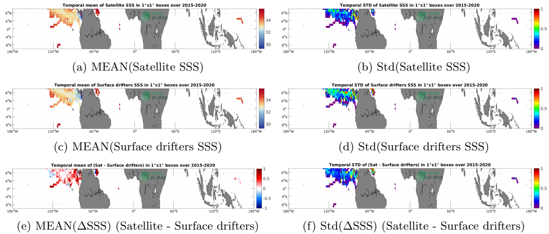
Figure 5: Temporal mean (left) and Std (right) of SSS from SMAP SSS L3 v5.0 - Monthly (JPL) (top), Surface drifters (middle), and of \Delta SSS (Satellite - Surface drifters). Only match-up pairs are used to generate these maps.
