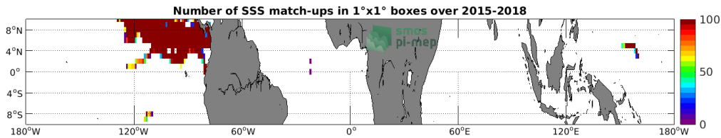
Figure 3: Number of SSS match-ups between Surface drifters SSS and the SMAP SSS L3 v5.0 - Monthly (JPL) SSS product for the Equatorial Ocean 10N-10S Pi-MEP region over 1°x1° boxes and for the full satellite product period.
