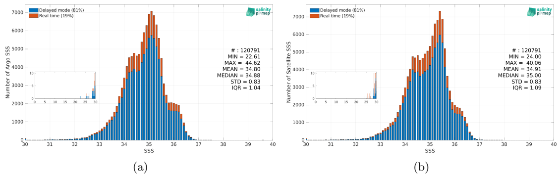
Figure 3: Histograms of SSS from Argo (a) and SMAP SSS L3 v5.0 - Monthly (JPL) (b) considering all match-up pairs per bins of 0.1 over the Equatorial Ocean 10N-10S Pi-MEP region and for the full satellite product period.
