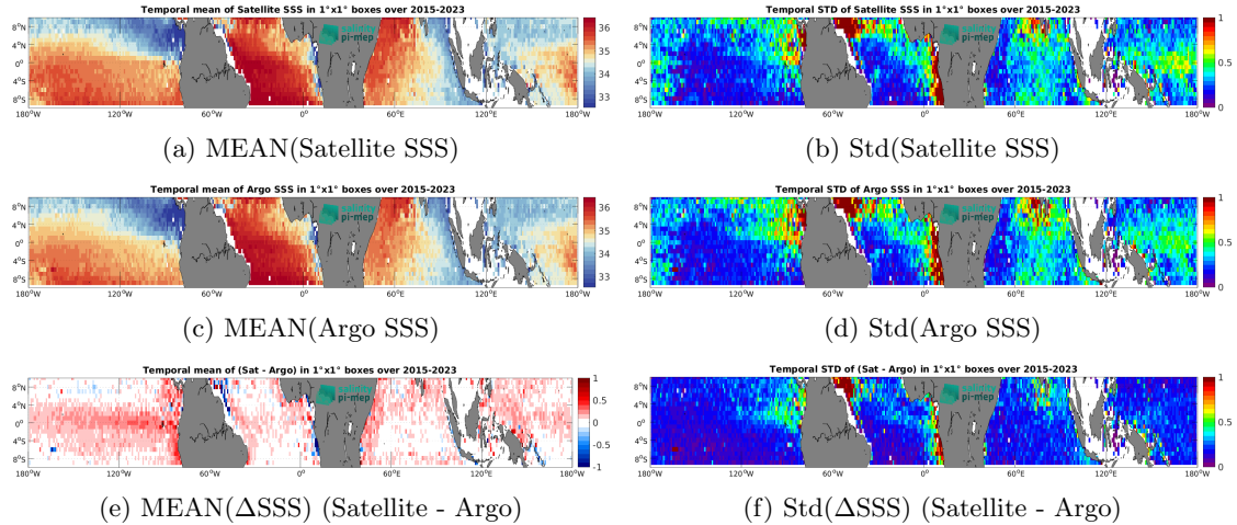
Figure 7: Temporal mean (left) and Std (right) of SSS from SMAP SSS L3 v5.0 - Monthly (JPL) (top), Argo (middle), and of \Delta SSS (Satellite - Argo). Only match-up pairs are used to generate these maps.
