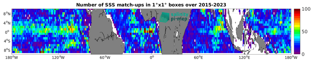
Figure 5: Number of SSS match-ups between Argo SSS and the SMAP SSS L3 v5.0 - Monthly (JPL) SSS product for the Equatorial Ocean 10N-10S Pi-MEP region over 1^\circ \times 1^\circ boxes and for the full satellite product period.
