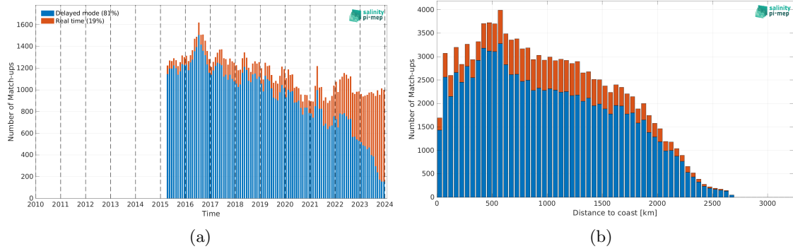
Figure 2: Number of match-ups between Argo and SMAP SSS L3 v5.0 - Monthly (JPL) SSS as a function of time (a) and as function of the distance to coast (b) over the Equatorial Ocean 10N-10S Pi-MEP region and for the full satellite product period.
