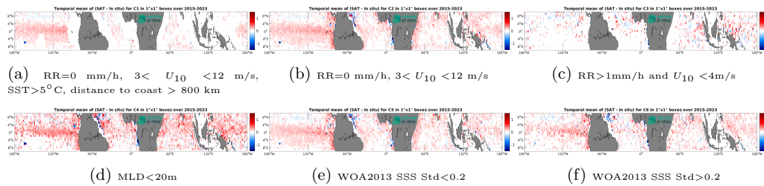
Figure 14: Temporal mean gridded over spatial boxes of size 1^\circ \times 1^\circ of \Delta SSS (SMAP SSS L3 v5.0 - Monthly (JPL) - Argo) for 6 different subdatasets corresponding to:RR=0 mm/h, 3 < U_{10} < 12 m/s, SST >5^\circ\text{C} , distance to coast > 800 km (a), RR=0 mm/h, 3 < U_{10} < 12 m/s (b), RR >1 mm/h and U_{10} < 4 m/s (c),MLD <20 m (d),WOA2013 SSS Std <0.2 (e),WOA2013 SSS Std >0.2 (f).
