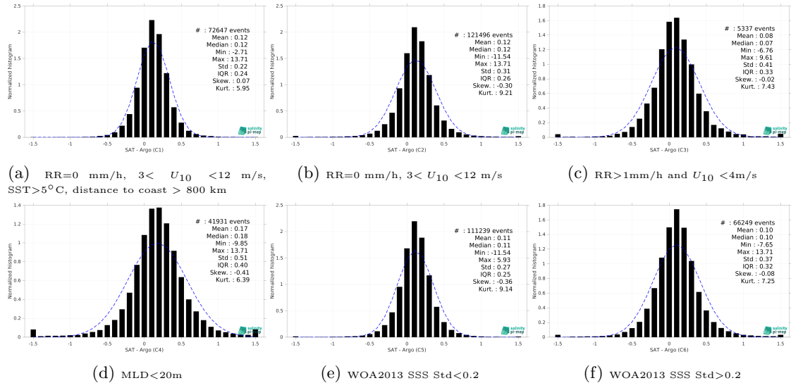
Figure 13: Normalized histogram of \Delta SSS (SMAP SSS L3 v5.0 - Monthly (JPL) - Argo) for 6 different subdatasets corresponding to: RR=0 mm/h, 3 < U_{10} < 12 m/s, SST >5^\circ C, distance to coast > 800 km (a), RR=0 mm/h, 3 < U_{10} < 12 m/s (b), RR >1 mm/h and U_{10} < 4 m/s (c), MLD <20 m (d), WOA2013 SSS Std <0.2 (e), WOA2013 SSS Std >0.2 (f).
