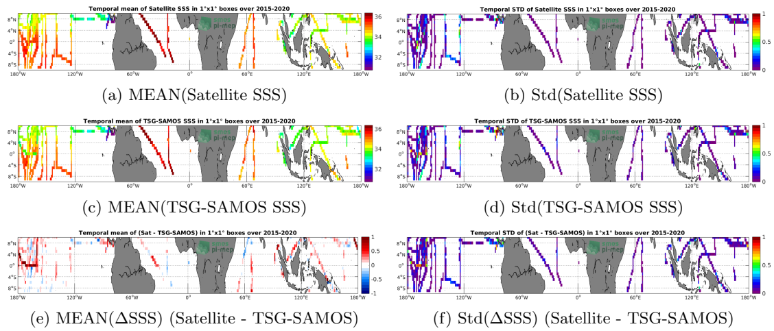
Figure 6: Temporal mean (left) and Std (right) of SSS from SMAP-L3-JPL-V4.3-MONTHLY-60KM (top), TSG-SAMOS (middle), and of \Delta SSS (Satellite - TSG-SAMOS). Only match-up pairs are used to generate these maps.
