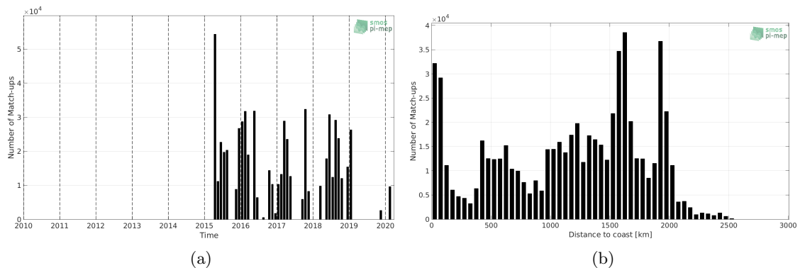
Figure 1: Number of match-ups between TSG-SAMOS and SMAP-L3-JPL-V4.3-MONTHLY-60KM SSS as a function of time (a) and as function of the distance to coast (b) over the Equatorial Ocean 10N-10S Pi-MEP region and for the full satellite product period.
