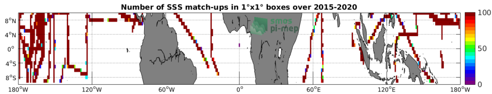
Figure 4: Number of SSS match-ups between TSG-SAMOS SSS and the SMAP-L3-JPL-V4.3-MONTHLY-60KM SSS product for the Equatorial Ocean 10N-10S Pi-MEP region over 1^\circ \times 1^\circ boxes and for the full satellite product period.
