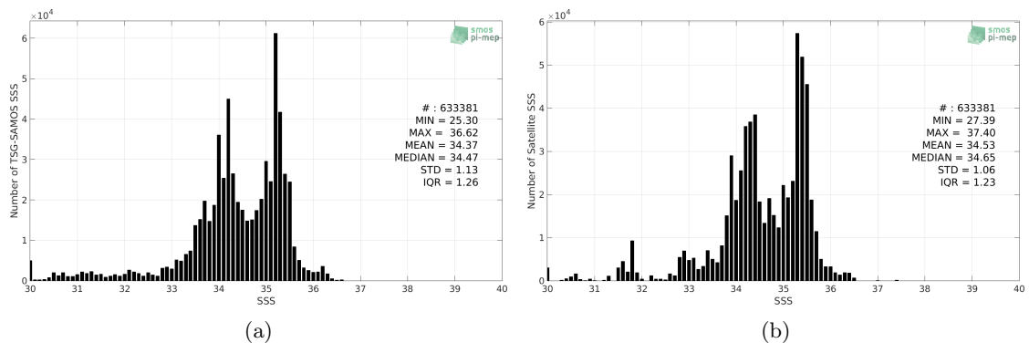
Figure 2: Histograms of SSS from TSG-SAMOS (a) and SMAP-L3-JPL-V4.3-MONTHLY-60KM (b) considering all match-up pairs per bins of 0.1 over the Equatorial Ocean 10N-10S Pi-MEP region and for the full satellite product period.
