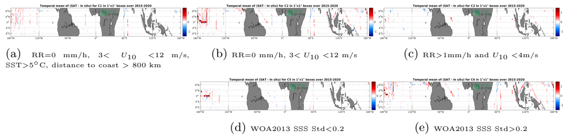
Figure 12: Temporal mean gridded over spatial boxes of size 1^\circ \times 1^\circ of \Delta SSS (SMAP-L3-JPL-V4.3-MONTHLY-60KM - TSG-SAMOS) for 5 different subdatasets corresponding to:RR=0 mm/h, 3 < U_{10} < 12 m/s, SST >5^\circ\text{C} , distance to coast > 800 km (a), RR=0 mm/h, 3 < U_{10} < 12 m/s (b), RR >1 mm/h and U_{10} < 4 m/s (c), WOA2013 SSS Std <0.2 (d), WOA2013 SSS Std >0.2 (e).
