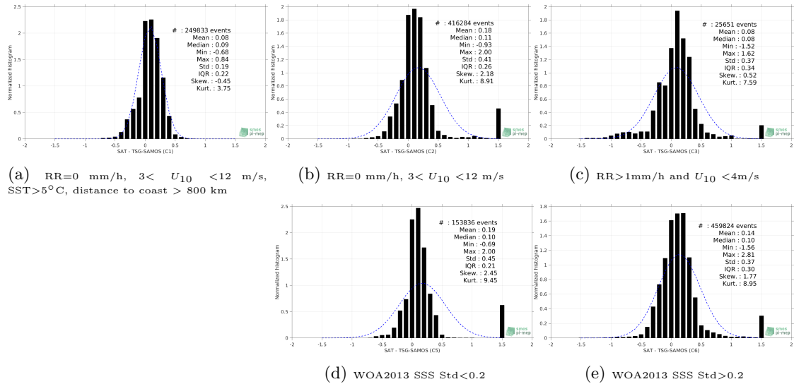
Figure 13: Normalized histogram of \Delta SSS (SMAP-L3-JPL-V4.3-MONTHLY-60KM - TSG-SAMOS) for 5 different subdatasets corresponding to: RR=0 mm/h, 3 < U_{10} < 12 m/s, SST >5^\circ\text{C} , distance to coast > 800 km (a), RR=0 mm/h, 3 < U_{10} < 12 m/s (b), RR >1 mm/h and U_{10} < 4 m/s (c), WOA2013 SSS Std <0.2 (d), WOA2013 SSS Std >0.2 (e).
