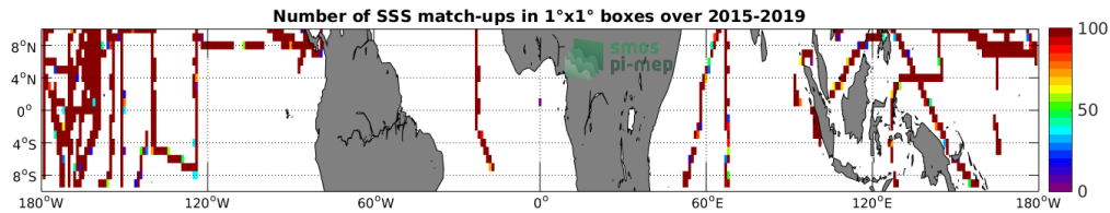
Figure 4: Number of SSS match-ups between TSG-SAMOS SSS and the SMAP-L3-JPL-V4.3-MONTHLY-60KM SSS product for the Equatorial Ocean 10N-10S Pi-MEP region over 1°x1° boxes and for the full satellite product period.
