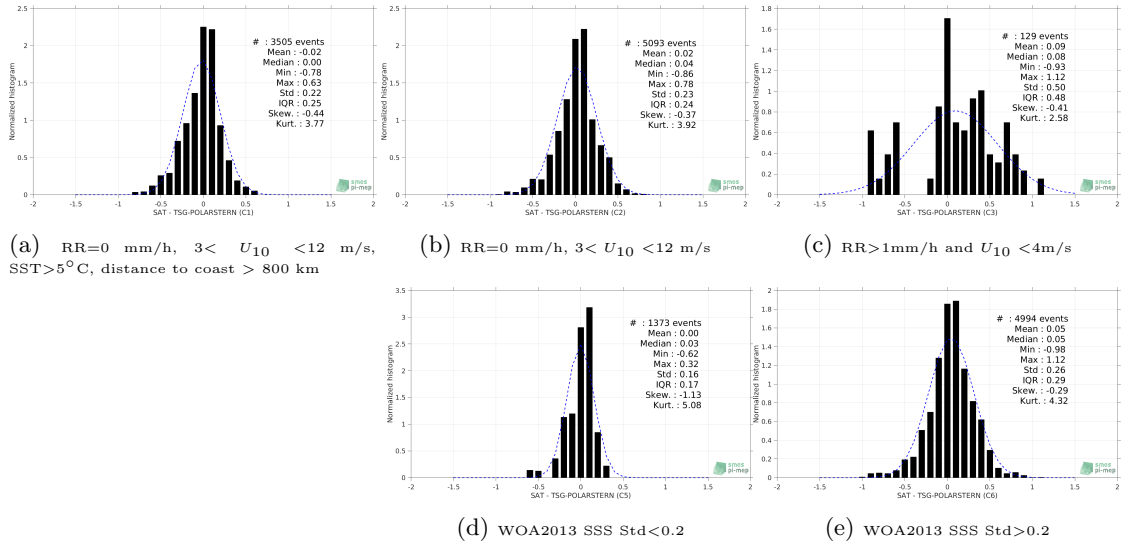
Figure 13: Normalized histogram of ΔSSS (SMAP-L3-JPL-V4.3-MONTHLY-60KM - TSG-POLARSTERN) for 5 different subdatasets corresponding to: RR=0 mm/h, 3 < U_{10} < 12 m/s, SST>5°C, distance to coast > 800 km (a), RR=0 mm/h, 3 < U_{10} < 12 m/s (b), RR>1mm/h and U_{10} < 4 m/s (c), WOA2013 SSS Std<0.2 (d), WOA2013 SSS Std>0.2 (e).
