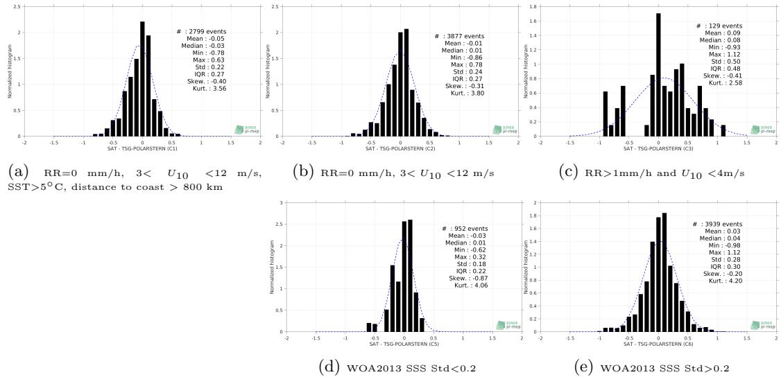
Figure 13: Normalized histogram of \Delta SSS (SMAP-L3-JPL-V4.3-MONTHLY-60KM - TSG-POLARSTERN) for 5 different subdatasets corresponding to: RR=0 mm/h, 3 < U_{10} < 12 m/s, SST >5^\circ C, distance to coast > 800 km (a), RR=0 mm/h, 3 < U_{10} < 12 m/s (b), RR >1 mm/h and U_{10} < 4 m/s (c), WOA2013 SSS Std <0.2 (d), WOA2013 SSS Std >0.2 (e).
