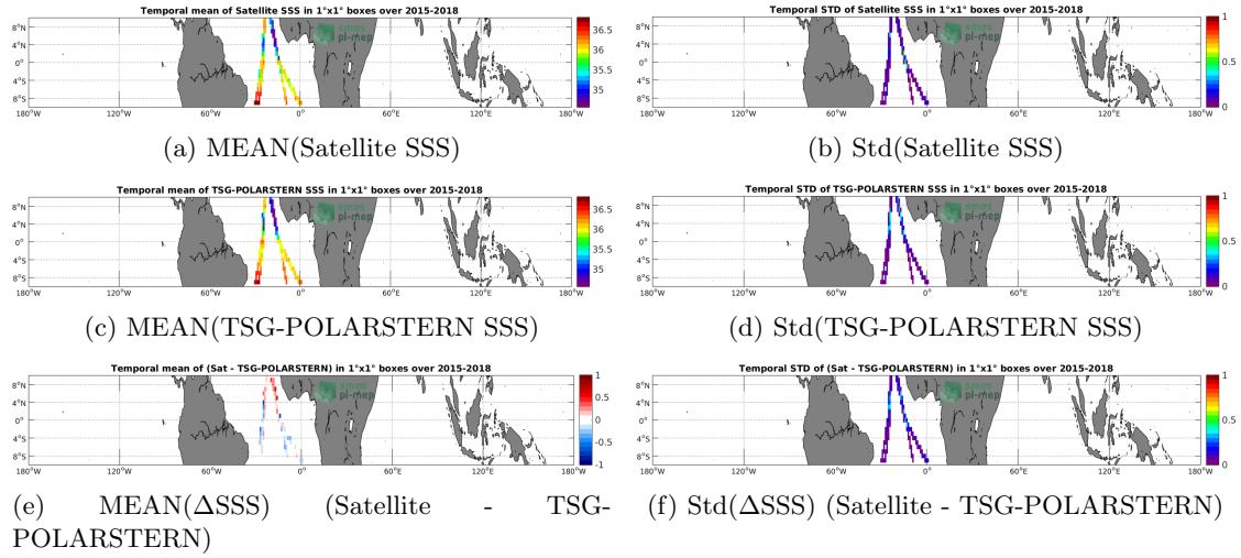
Figure 6: Temporal mean (left) and Std (right) of SSS from SMAP-L3-JPL-V4.3-MONTHLY-60KM (top), TSG-POLARSTERN (middle), and of \Delta SSS (Satellite - TSG-POLARSTERN). Only match-up pairs are used to generate these maps.
