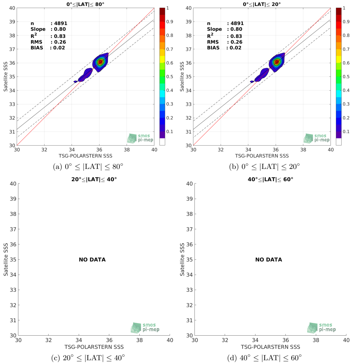
Figure 9: Contour maps of the concentration of SMAP-L3-JPL-V4.3-MONTHLY-60KM SSS (y-axis) versus TSG-POLARSTERN SSS (x-axis) at match-up pairs for different latitude bands. For each plot, the red line shows x=y . The black thin and dashed lines indicate a linear fit through the data cloud and the \pm 95\% confidence levels, respectively. The number match-up pairs n , the slope and R^2 coefficient of the linear fit, the root mean square (RMS) and the mean bias between satellite and in situ data are indicated for each latitude band in each plots.
