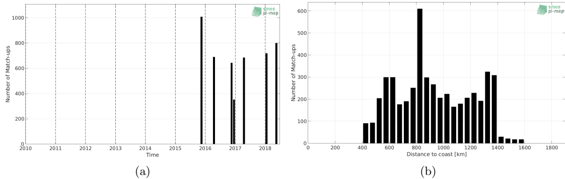
Figure 1: Number of match-ups between TSG-POLARSTERN and SMAP-L3-JPL-V4.3-MONTHLY-60KM SSS as a function of time (a) and as function of the distance to coast (b) over the Equatorial Ocean 10N-10S Pi-MEP region and for the full satellite product period.
