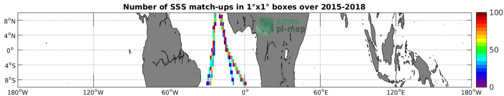
Figure 4: Number of SSS match-ups between TSG-POLARSTERN SSS and the SMAP-L3-JPL-V4.3-MONTHLY-60KM SSS product for the Equatorial Ocean 10N-10S Pi-MEP region over 1°x1° boxes and for the full satellite product period.
