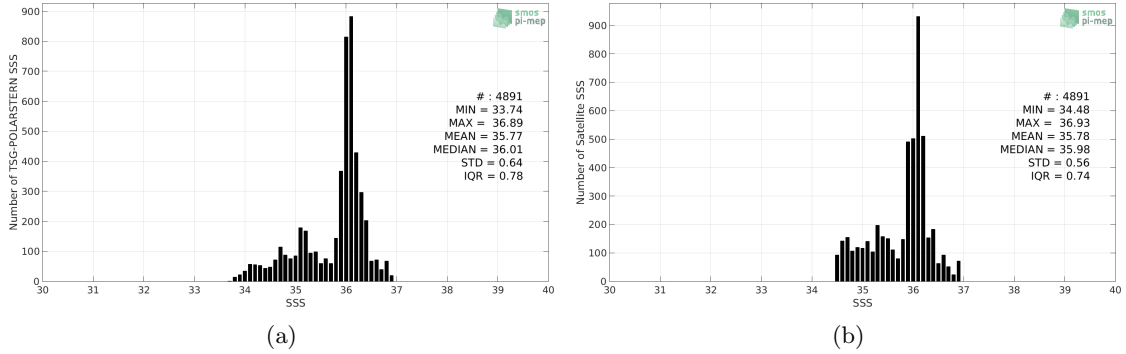
Figure 2: Histograms of SSS from TSG-POLARSTERN (a) and SMAP-L3-JPL-V4.3-MONTHLY-60KM (b) considering all match-up pairs per bins of 0.1 over the Equatorial Ocean 10N-10S Pi-MEP region and for the full satellite product period.
