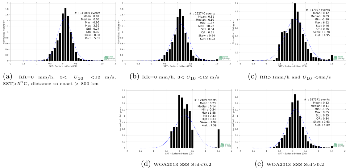
Figure 12: Normalized histogram of ΔSSS (SMAP-L3-JPL-V4.3-MONTHLY-60KM - Surface drifters) for 5 different subdatasets corresponding to: RR=0 mm/h, 3 < U 10 < 12 m/s, SST > 5°C, distance to coast > 800 km (a), RR=0 mm/h, 3 < U 10 < 12 m/s (b), RR > 1mm/h and U 10 < 4m/s (c), WOA2013 SSS Std < 0.2 (d), WOA2013 SSS Std > 0.2 (e).
