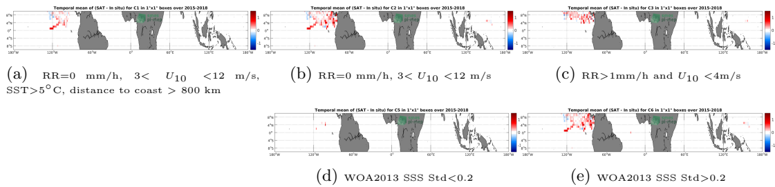
Figure 11: Temporal mean gridded over spatial boxes of size 1°x1° of ΔSSS (SMAP-L3-JPL-V4.3-MONTHLY-60KM - Surface drifters) for 5 different subdatasets corresponding to:RR=0 mm/h, 3 < U 10 < 12 m/s, SST > 5°C, distance to coast > 800 km (a), RR=0 mm/h, 3 < U 10 < 12 m/s (b), RR > 1mm/h and U 10 < 4m/s (c), WOA2013 SSS Std < 0.2 (d), WOA2013 SSS Std > 0.2 (e).
