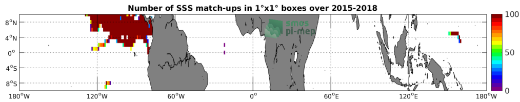
Figure 3: Number of SSS match-ups between Surface drifters SSS and the SMAP-L3-JPL-V4.3-MONTHLY-60KM SSS product for the Equatorial Ocean 10N-10S Pi-MEP region over 1°x1° boxes and for the full satellite product period.
