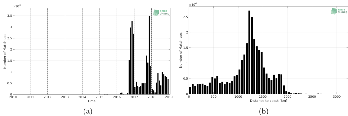
Figure 1: Number of match-ups between Surface drifters and SMAP-L3-JPL-V4.3-MONTHLY-60KM SSS as a function of time (a) and as function of the distance to coast (b) over the Equatorial Ocean 10N-10S Pi-MEP region and for the full satellite product period.
