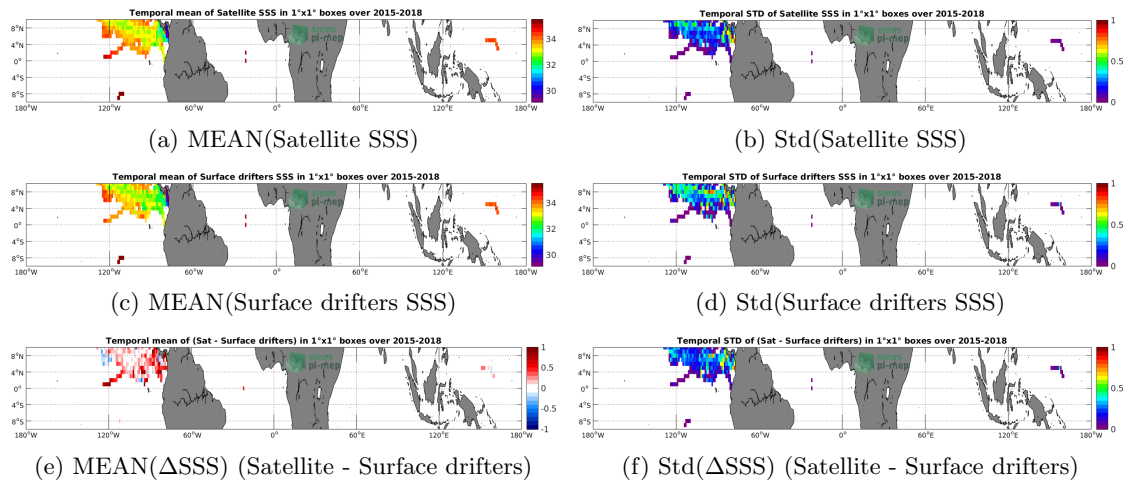
Figure 5: Temporal mean (left) and Std (right) of SSS from SMAP-L3-JPL-V4.3-MONTHLY-60KM (top), Surface drifters (middle), and of \Delta SSS (Satellite - Surface drifters). Only match-up pairs are used to generate these maps.
