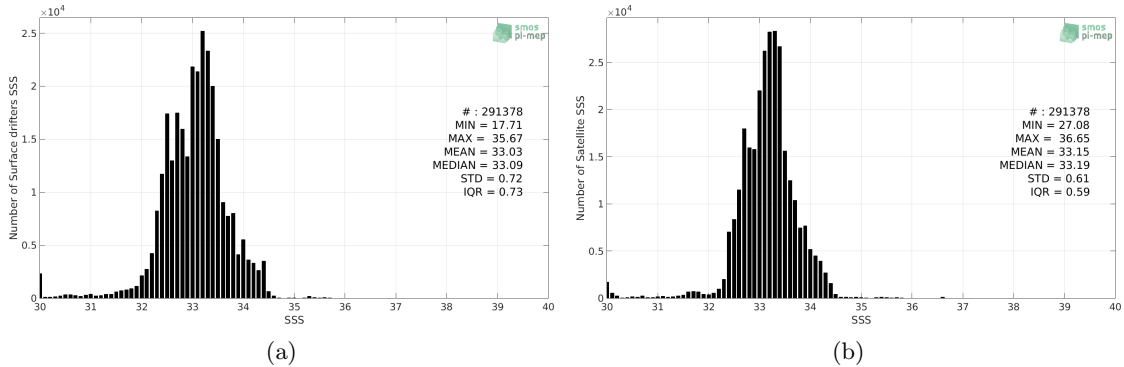
Figure 2: Histograms of SSS from Surface drifters (a) and SMAP-L3-JPL-V4.3-MONTHLY-60KM (b) considering all match-up pairs per bins of 0.1 over the Equatorial Ocean 10N-10S Pi-MEP region and for the full satellite product period.
