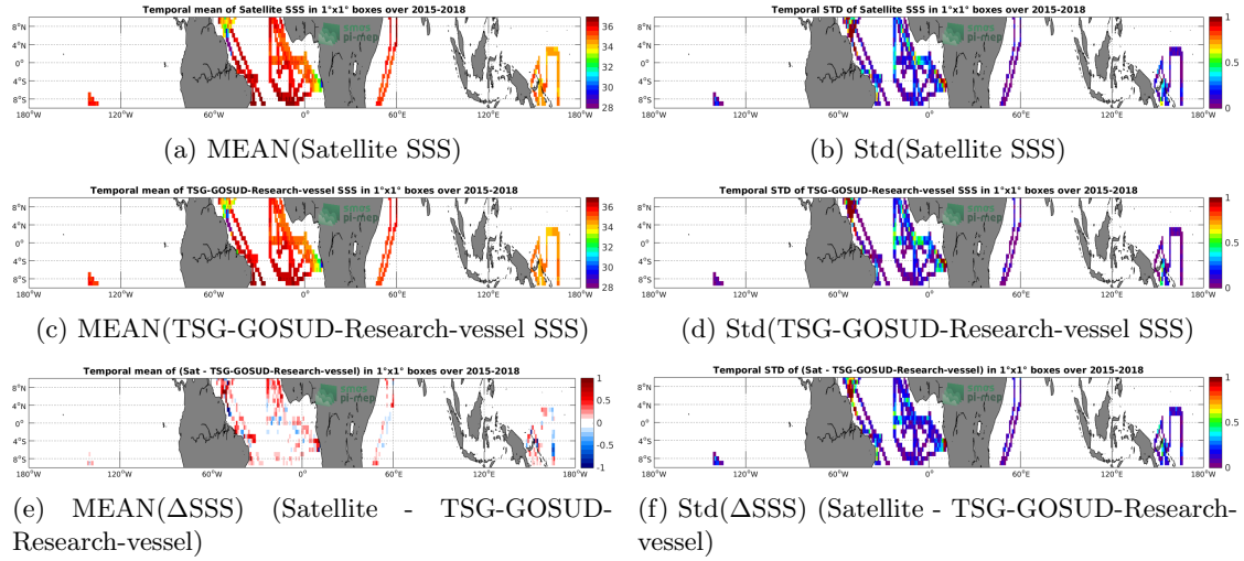
Figure 6: Temporal mean (left) and Std (right) of SSS from SMAP-L3-JPL-V4.2-8DAY-RUNNING-60KM (top), TSG-GOSUD-Research-vessel (middle), and of \Delta SSS (Satellite - TSG-GOSUD-Research-vessel). Only match-up pairs are used to generate these maps.
