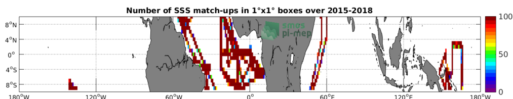
Figure 4: Number of SSS match-ups between TSG-GOSUD-Research-vessel SSS and the SMAP-L3-JPL-V4.2-8DAY-RUNNING-60KM SSS product for the Equatorial Ocean 10N-10S Pi-MEP region over 1^\circ \times 1^\circ boxes and for the full satellite product period.
