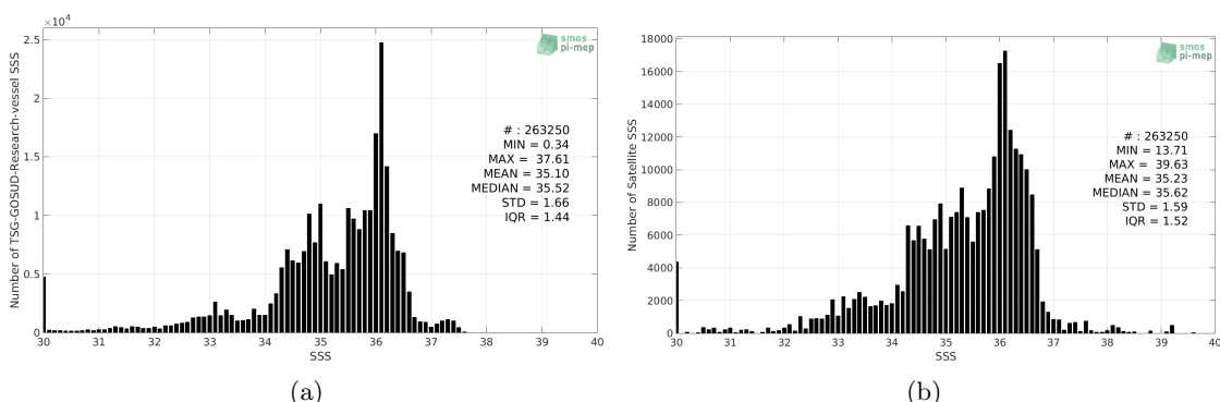
Figure 2: Histograms of SSS from TSG-GOSUD-Research-vessel (a) and SMAP-L3-JPL-V4.2-8DAY-RUNNING-60KM (b) considering all match-up pairs per bins of 0.1 over the Equatorial Ocean 10N-10S Pi-MEP region and for the full satellite product period.
