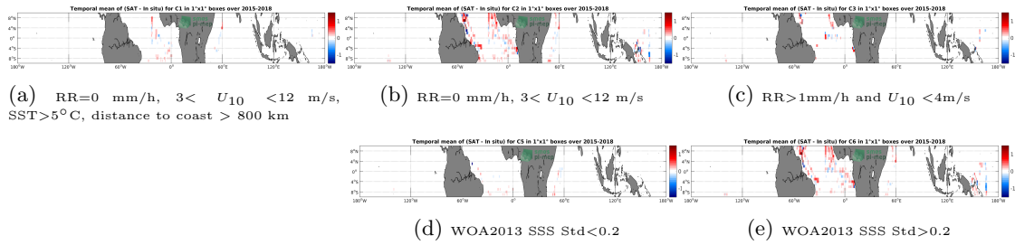
Figure 12: Temporal mean gridded over spatial boxes of size 1^\circ \times 1^\circ of \Delta SSS (SMAP-L3-JPL-V4.2-8DAY-RUNNING-60KM - TSG-GOSUD-Research-vessel) for 5 different subdatasets corresponding to: RR=0 mm/h, 3 < U_{10} < 12 m/s, SST>5°C, distance to coast > 800 km (a), RR=0 mm/h, 3 < U_{10} < 12 m/s (b), RR>1mm/h and U_{10} < 4 m/s (c), WOA2013 SSS Std<0.2 (d), WOA2013 SSS Std>0.2 (e).
