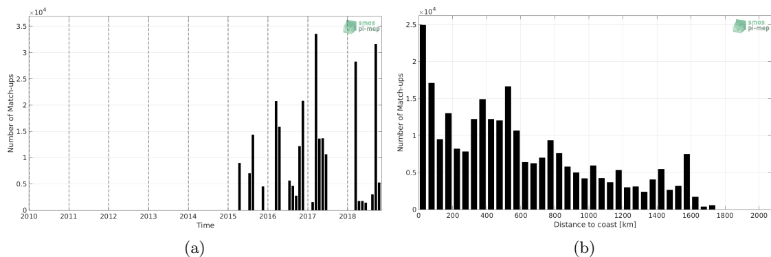
Figure 1: Number of match-ups between TSG-GOSUD-Research-vessel and SMAP-L3-JPL-V4.2-8DAY-RUNNING-60KM SSS as a function of time (a) and as function of the distance to coast (b) over the Equatorial Ocean 10N-10S Pi-MEP region and for the full satellite product period.
