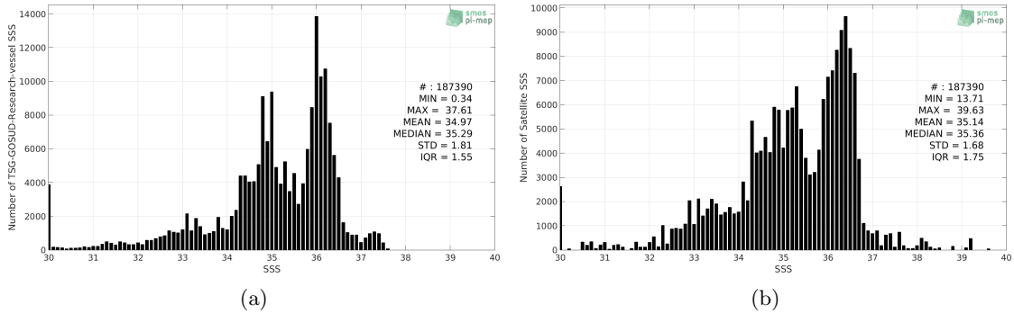
Figure 2: Histograms of SSS from TSG-GOSUD-Research-vessel (a) and SMAP-L3-JPL-V4.2-8DAY-RUNNING-60KM (b) considering all match-up pairs per bins of 0.1 over the Equatorial Ocean 10N-10S Pi-MEP region and for the full satellite product period.
