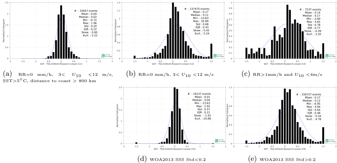
Figure 13: Normalized histogram of \Delta SSS (SMAP-L3-JPL-V4.2-8DAY-RUNNING-60KM - TSG-GOSUD-Research-vessel) for 5 different subdatasets corresponding to: RR=0 mm/h, 3 < U_{10} < 12 m/s, SST >5^\circ\text{C} , distance to coast > 800 km (a), RR=0 mm/h, 3 < U_{10} < 12 m/s (b), RR >1 mm/h and U_{10} < 4 m/s (c), WOA2013 SSS Std <0.2 (d), WOA2013 SSS Std >0.2 (e).
