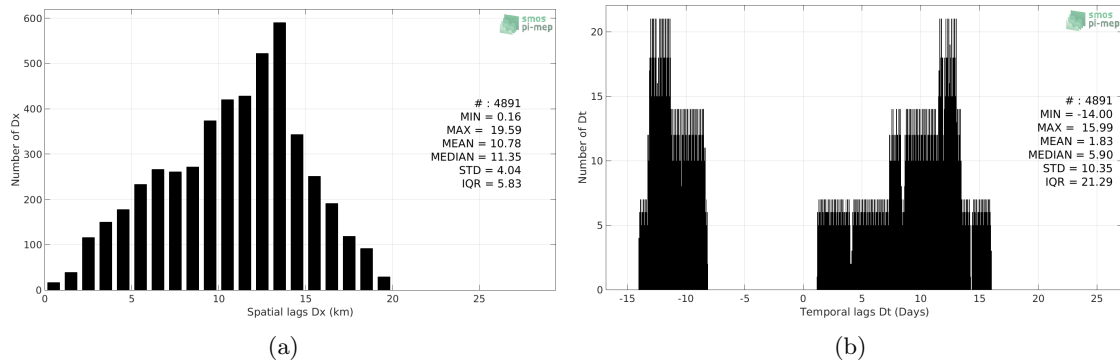
Figure 5: Histograms of the spatial (a) and temporal (b) lags between the time of the TSG-POLARSTERN measurements and the date of the corresponding SMAP-L3-JPL-V4.2-MONTHLY-60KM SSS product.
