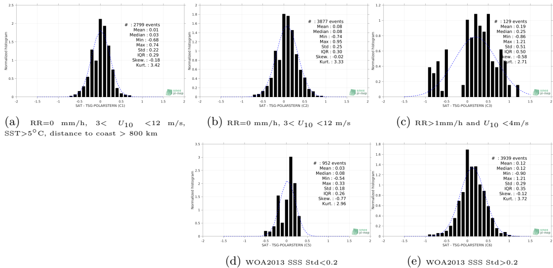
Figure 13: Normalized histogram of \Delta SSS (SMAP-L3-JPL-V4.2-MONTHLY-60KM - TSG-POLARSTERN) for 5 different subdatasets corresponding to: RR=0 mm/h, 3 < U_{10} < 12 m/s, SST >5^\circ C, distance to coast > 800 km (a), RR=0 mm/h, 3 < U_{10} < 12 m/s (b), RR >1 mm/h and U_{10} < 4 m/s (c), WOA2013 SSS Std <0.2 (d), WOA2013 SSS Std >0.2 (e).
