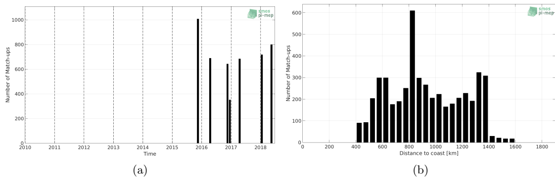
Figure 1: Number of match-ups between TSG-POLARSTERN and SMAP-L3-JPL-V4.2-MONTHLY-60KM SSS as a function of time (a) and as function of the distance to coast (b) over the Equatorial Ocean 10N-10S Pi-MEP region and for the full satellite product period.
