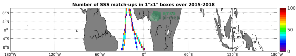
Figure 4: Number of SSS match-ups between TSG-POLARSTERN SSS and the SMAP-L3-JPL-V4.2-MONTHLY-60KM SSS product for the Equatorial Ocean 10N-10S Pi-MEP region over 1^\circ \times 1^\circ boxes and for the full satellite product period.
