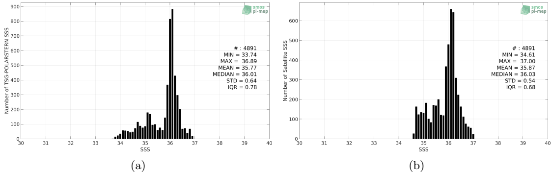
Figure 2: Histograms of SSS from TSG-POLARSTERN (a) and SMAP-L3-JPL-V4.2-MONTHLY-60KM (b) considering all match-up pairs per bins of 0.1 over the Equatorial Ocean 10N-10S Pi-MEP region and for the full satellite product period.
