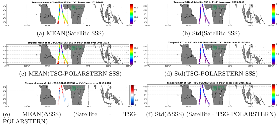
Figure 6: Temporal mean (left) and Std (right) of SSS from SMAP-L3-JPL-V4.2-MONTHLY-60KM (top), TSG-POLARSTERN (middle), and of \Delta SSS (Satellite - TSG-POLARSTERN). Only match-up pairs are used to generate these maps.
