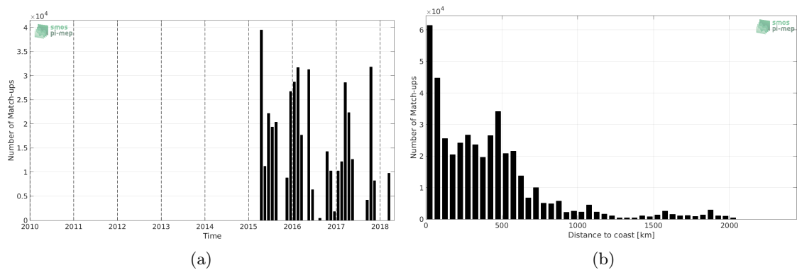
Figure 1: Number of match-ups between TSG-SAMOS and SMAP-L3-JPL-V4-8DAY-RUNNING-60KM SSS as a function of time (a) and as function of the distance to coast (b) over the Equatorial Ocean 10N-10S Pi-MEP region and for the full satellite product period.
