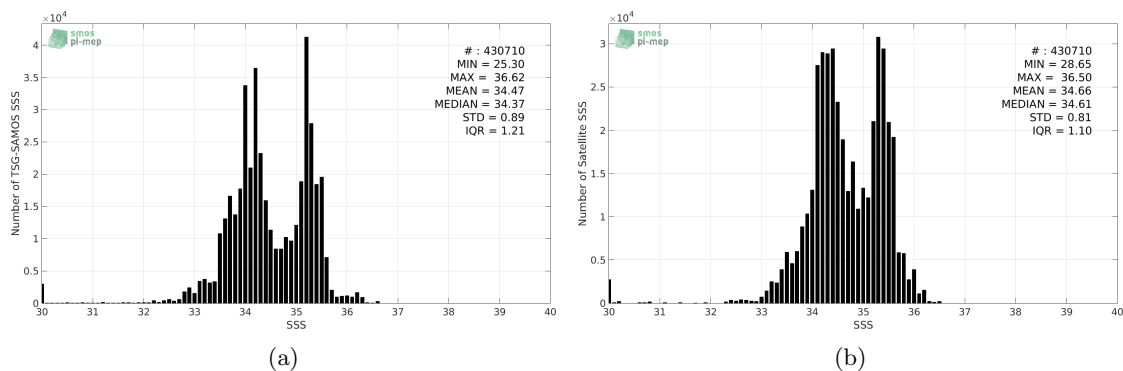
Figure 2: Histograms of SSS from TSG-SAMOS (a) and SMAP-L3-JPL-V4-8DAY-RUNNING-60KM (b) considering all match-up pairs per bins of 0.1 over the Equatorial Ocean 10N-10S Pi-MEP region and for the full satellite product period.
