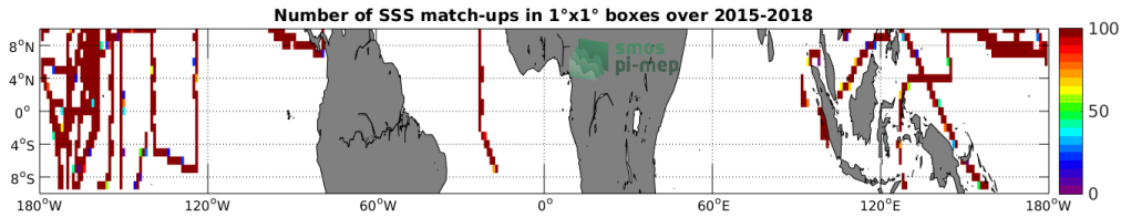
Figure 4: Number of SSS match-ups between TSG-SAMOS SSS and the SMAP-L3-JPL-V4-8DAY-RUNNING-60KM SSS product for the Equatorial Ocean 10N-10S Pi-MEP region over 1°x1° boxes and for the full satellite product period.
