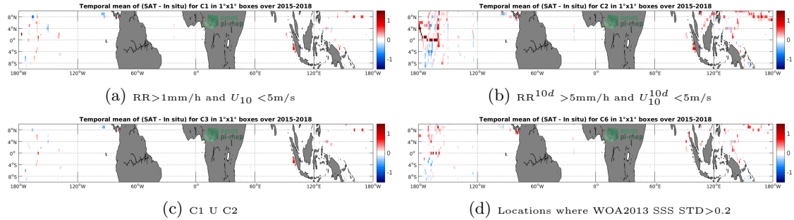
Figure 12: Temporal mean gridded over spatial boxes of size 1^\circ \times 1^\circ of \Delta SSS (SMAP-L3-JPL-V4-8DAY-RUNNING-60KM - TSG-SAMOS) for 4 different subdatasets corresponding to: RR > 1\text{mm/h} and U_{10} < 5\text{m/s} (a), RR^{10d} > 5\text{mm/h} and U_{10}^{10d} < 5\text{m/s} (b), C1 U C2 (c), Locations where WOA2013 SSS STD > 0.2 (d).
