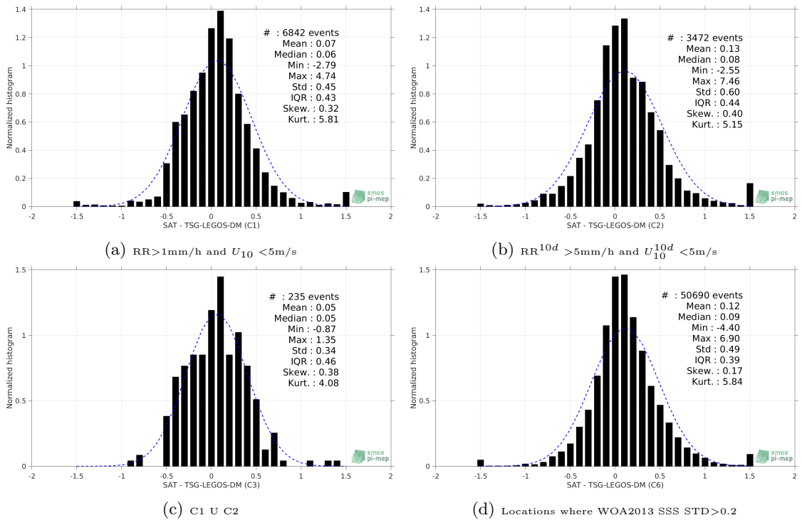
Figure 13: Normalized histogram of \Delta SSS (SMAP-L3-JPL-V4-8DAY-RUNNING-60KM - TSG-LEGOS-DM) for 6 different subdatasets corresponding to: RR > 1\text{mm/h} and U_{10} < 5\text{m/s} (a), RR^{10d} > 5\text{mm/h} and U_{10}^{10d} < 5\text{m/s} (b), C1 U C2 (c), Locations where WOA2013 SSS STD > 0.2 (d).
