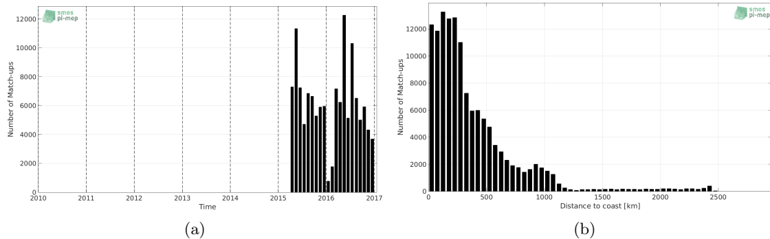
Figure 1: Number of match-ups between TSG-LEGOS-DM and SMAP-L3-JPL-V4-8DAY-RUNNING-60KM SSS as a function of time (a) and as function of the distance to coast (b) over the Equatorial Ocean 10N-10S Pi-MEP region and for the full satellite product period.
