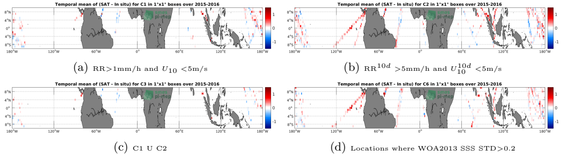
Figure 12: Temporal mean gridded over spatial boxes of size 1^\circ \times 1^\circ of \Delta SSS (SMAP-L3-JPL-V4-8DAY-RUNNING-60KM - TSG-LEGOS-DM) for 4 different subdatasets corresponding to: RR > 1\text{mm/h} and U_{10} < 5\text{m/s} (a), RR^{10d} > 5\text{mm/h} and U_{10}^{10d} < 5\text{m/s} (b), C1 U C2 (c), Locations where WOA2013 SSS STD > 0.2 (d).
