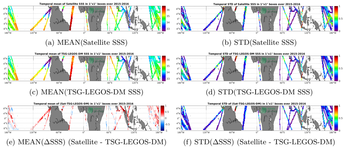
Figure 6: Temporal mean (left) and STD (right) of SSS from SMAP-L3-JPL-V4-8DAY-RUNNING-60KM (top), TSG-LEGOS-DM (middle), and of \Delta SSS (Satellite - TSG-LEGOS-DM). Only match-up pairs are used to generate these maps.
