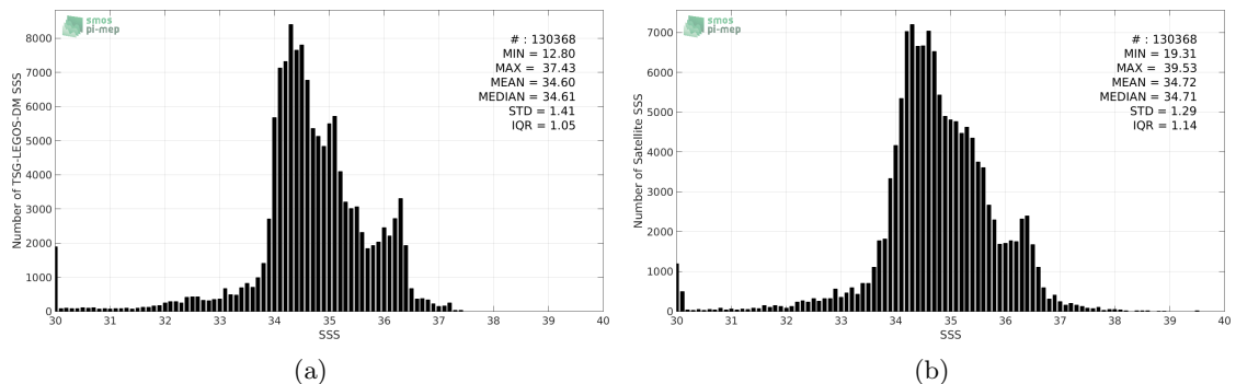
Figure 2: Histograms of SSS from TSG-LEGOS-DM (a) and SMAP-L3-JPL-V4-8DAY-RUNNING-60KM (b) considering all match-up pairs per bins of 0.1 over the Equatorial Ocean 10N-10S Pi-MEP region and for the full satellite product period.
