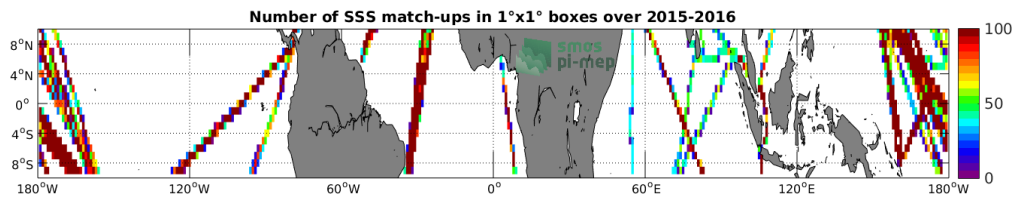
Figure 4: Number of SSS match-ups between TSG-LEGOS-DM SSS and the SMAP-L3-JPL-V4-8DAY-RUNNING-60KM SSS product for the Equatorial Ocean 10N-10S Pi-MEP region over 1^\circ \times 1^\circ boxes and for the full satellite product period.
