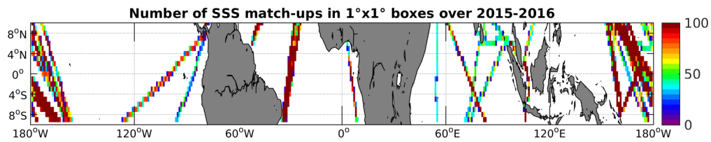
Figure 4: Number of SSS match-ups between TSG-LEGOS-DM SSS and the SMAP-L3-JPL-V4-8DAY-RUNNING-60KM SSS product for the Equatorial Ocean 10N-10S Pi-MEP region over 1^\circ \times 1^\circ boxes and for the full satellite product period.
