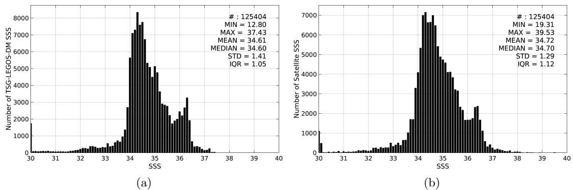
Figure 2: Histograms of SSS from TSG-LEGOS-DM (a) and SMAP-L3-JPL-V4-8DAY-RUNNING-60KM (b) considering all match-up pairs per bins of 0.1 over the Equatorial Ocean 10N-10S Pi-MEP region and for the full satellite product period.
