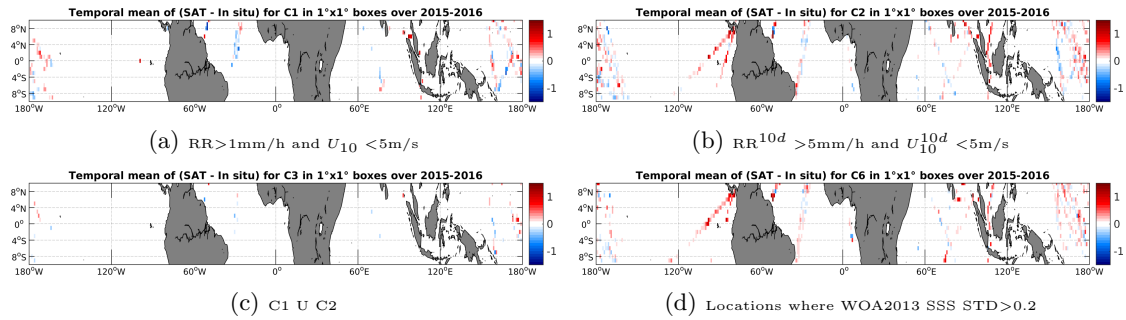
Figure 12: Temporal mean gridded over spatial boxes of size 1^\circ \times 1^\circ of \Delta SSS (SMAP-L3-JPL-V4-8DAY-RUNNING-60KM - TSG-LEGOS-DM) for 4 different subdatasets corresponding to: RR > 1\text{mm/h} and U_{10} < 5\text{m/s} (a), RR^{10d} > 5\text{mm/h} and U_{10}^{10d} < 5\text{m/s} (b), C1 U C2 (c), Locations where WOA2013 SSS STD > 0.2 (d).
