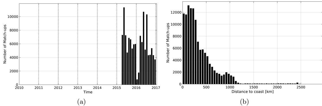
Figure 1: Number of match-ups between TSG-LEGOS-DM and SMAP-L3-JPL-V4-8DAY-RUNNING-60KM SSS as a function of time (a) and as function of the distance to coast (b) over the Equatorial Ocean 10N-10S Pi-MEP region and for the full satellite product period.
