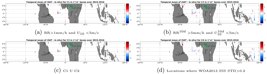
Figure 12: Temporal mean gridded over spatial boxes of size 1^\circ \times 1^\circ of \Delta SSS (SMAP-L3-JPL-V4-8DAY-RUNNING-60KM - TSG-GOSUD-Research-vessel) for 4 different subdatasets corresponding to: RR > 1\text{mm/h} and U_{10} < 5\text{m/s} (a), RR^{10d} > 5\text{mm/h} and U_{10}^{10d} < 5\text{m/s} (b), C1 U C2 (c), Locations where WOA2013 SSS STD > 0.2 (d).
