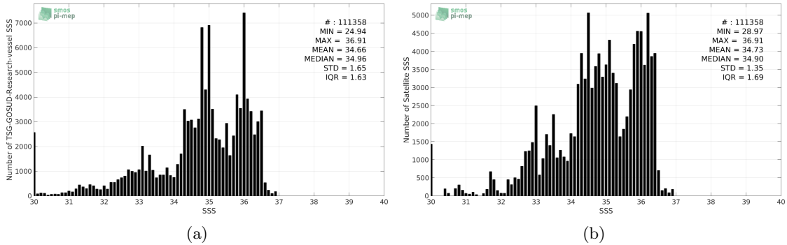
Figure 2: Histograms of SSS from TSG-GOSUD-Research-vessel (a) and SMAP-L3-JPL-V4-8DAY-RUNNING-60KM (b) considering all match-up pairs per bins of 0.1 over the Equatorial Ocean 10N-10S Pi-MEP region and for the full satellite product period.
