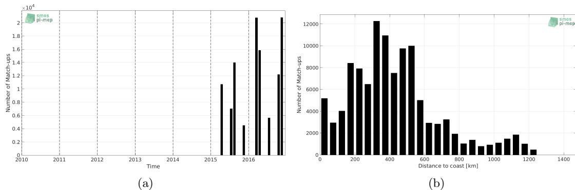
Figure 1: Number of match-ups between TSG-GOSUD-Research-vessel and SMAP-L3-JPL-V4-8DAY-RUNNING-60KM SSS as a function of time (a) and as function of the distance to coast (b) over the Equatorial Ocean 10N-10S Pi-MEP region and for the full satellite product period.
