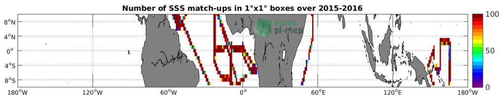
Figure 4: Number of SSS match-ups between TSG-GOSUD-Research-vessel SSS and the SMAP-L3-JPL-V4-8DAY-RUNNING-60KM SSS product for the Equatorial Ocean 10N-10S Pi-MEP region over 1^{\circ} \times 1^{\circ} boxes and for the full satellite product period.
