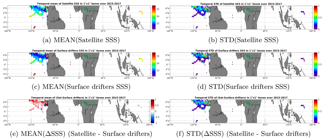
Figure 5: Temporal mean (left) and STD (right) of SSS from SMAP-L3-JPL-V4-8DAY-RUNNING-60KM (top), Surface drifters (middle), and of \Delta SSS (Satellite - Surface drifters). Only match-up pairs are used to generate these maps.
