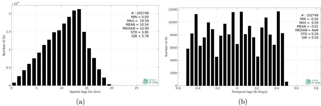
Figure 4: Histograms of the spatial (a) and temporal (b) lags between the time of the Surface drifters measurements and the date of the corresponding SMAP-L3-JPL-V4-8DAY-RUNNING-60KM SSS product.
