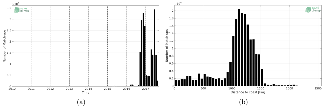
Figure 1: Number of match-ups between Surface drifters and SMAP-L3-JPL-V4-8DAY-RUNNING-60KM SSS as a function of time (a) and as function of the distance to coast (b) over the Equatorial Ocean 10N-10S Pi-MEP region and for the full satellite product period.
