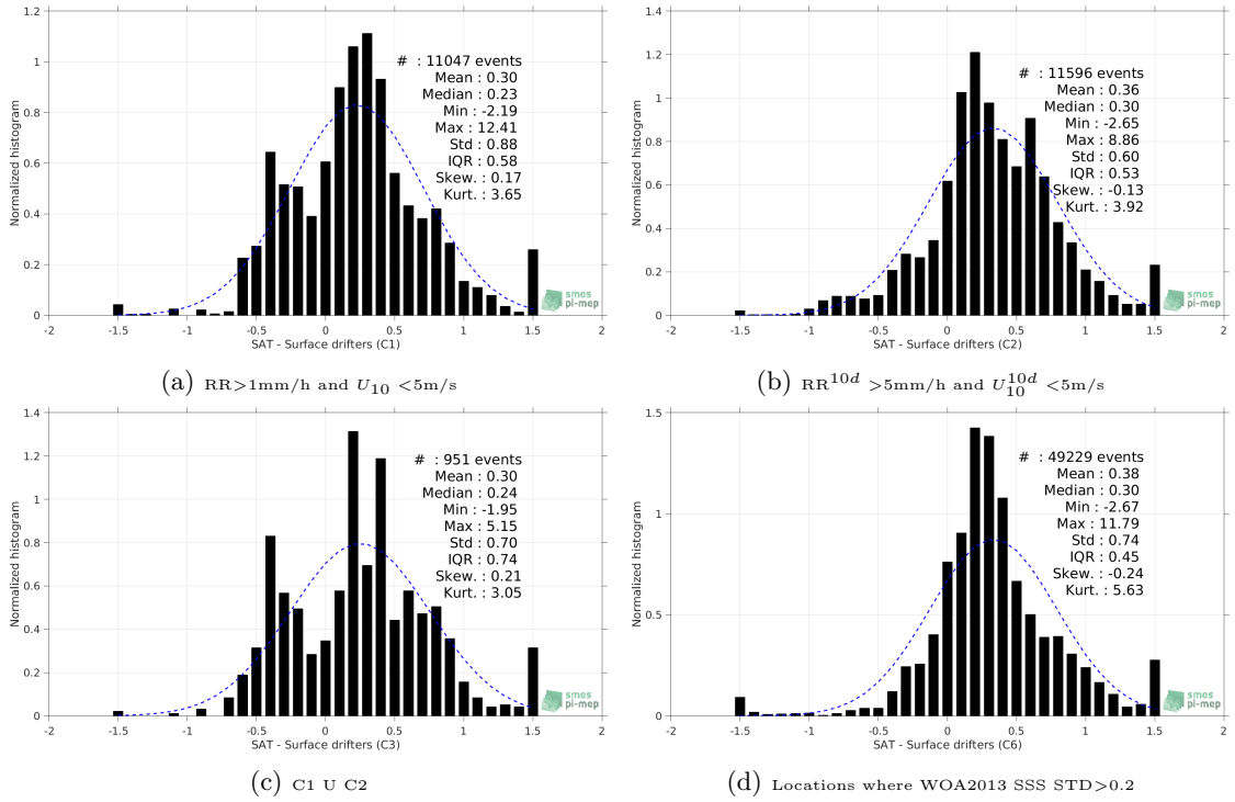
Figure 12: Normalized histogram of \Delta SSS (SMAP-L3-JPL-V4-8DAY-RUNNING-60KM - Surface drifters) for 6 different subdatasets corresponding to: RR > 1\text{mm/h} and U_{10} < 5\text{m/s} (a), RR^{10d} > 5\text{mm/h} and U_{10}^{10d} < 5\text{m/s} (b), C1 U C2 (c), Locations where WOA2013 SSS STD > 0.2 (d).
