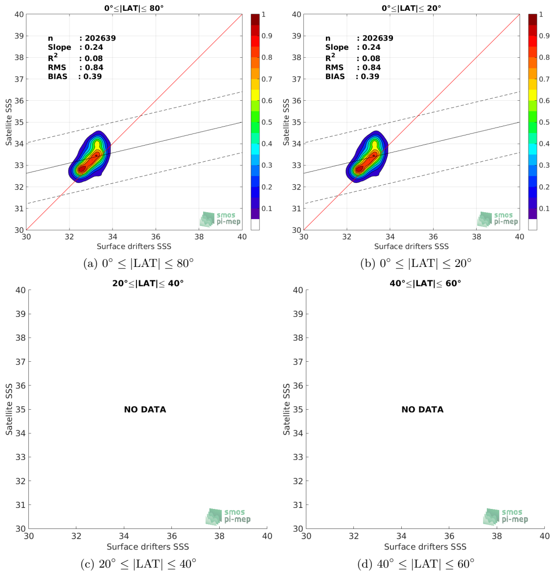
Figure 8: Contour maps of the concentration of SMAP-L3-JPL-V4-8DAY-RUNNING-60KM SSS (y-axis) versus Surface drifters SSS (x-axis) at match-up pairs for different latitude bands. For each plot, the red line shows x=y . The black thin and dashed lines indicate a linear fit through the data cloud and the \pm 95\% confidence levels, respectively. The number match-up pairs n , the slope and R^2 coefficient of the linear fit, the root mean square (RMS) and the mean bias between satellite and in situ data are indicated for each latitude band in each plots.
