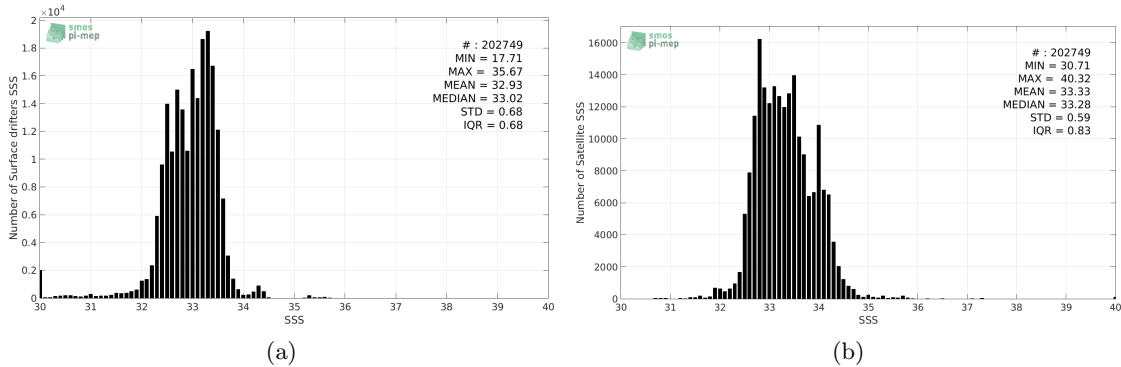
Figure 2: Histograms of SSS from Surface drifters (a) and SMAP-L3-JPL-V4-8DAY-RUNNING-60KM (b) considering all match-up pairs per bins of 0.1 over the Equatorial Ocean 10N-10S Pi-MEP region and for the full satellite product period.
