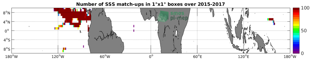
Figure 3: Number of SSS match-ups between Surface drifters SSS and the SMAP-L3-JPL-V4-8DAY-RUNNING-60KM SSS product for the Equatorial Ocean 10N-10S Pi-MEP region over 1°x1° boxes and for the full satellite product period.
