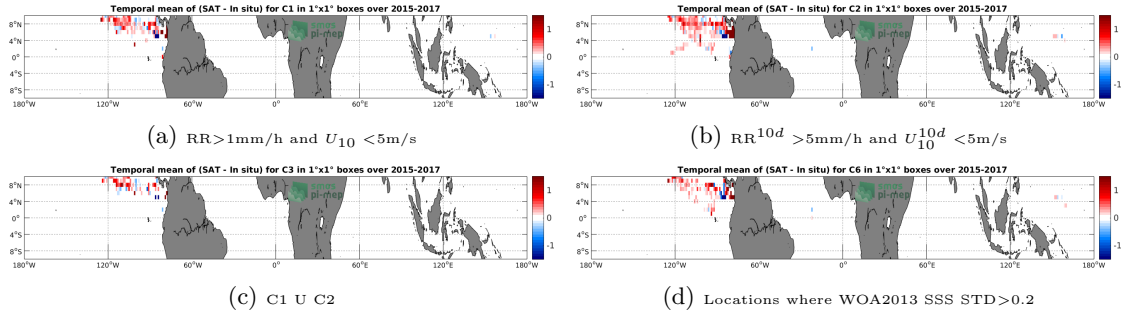
Figure 11: Temporal mean gridded over spatial boxes of size 1^\circ \times 1^\circ of \Delta SSS (SMAP-L3-JPL-V4-8DAY-RUNNING-60KM - Surface drifters) for 4 different subdatasets corresponding to: RR > 1\text{mm/h} and U_{10} < 5\text{m/s} (a), RR^{10d} > 5\text{mm/h} and U_{10}^{10d} < 5\text{m/s} (b), C1 U C2 (c), Locations where WOA2013 SSS STD > 0.2 (d).
