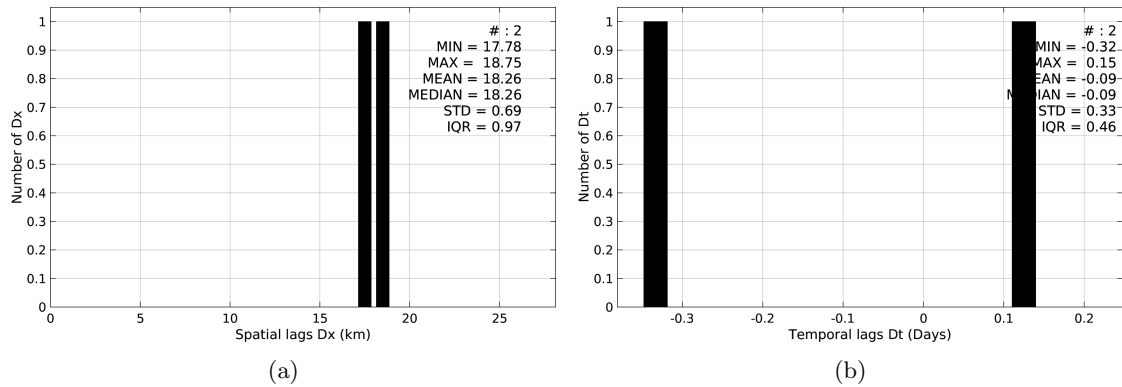
Figure 4: Histograms of the spatial (a) and temporal (b) lags between the time of the Surface drifters measurements and the date of the corresponding SMAP-L3-JPL-V4-8DAY-RUNNING-60KM SSS product.
