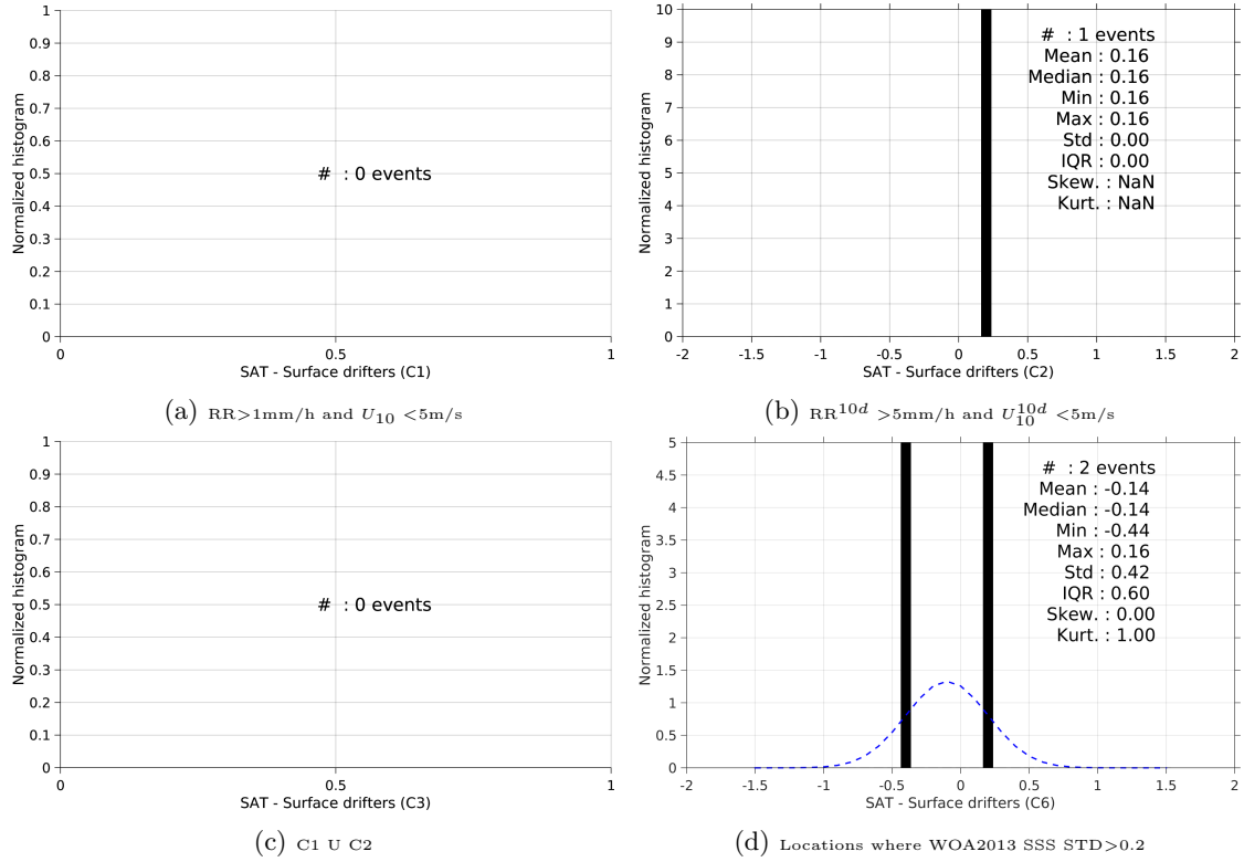
Figure 12: Normalized histogram of \Delta\text{SSS} (SMAP-L3-JPL-V4-8DAY-RUNNING-60KM - Surface drifters) for 6 different subdatasets corresponding to: RR > 1\text{mm/h} and U_{10} < 5\text{m/s} (a), RR^{10d} > 5\text{mm/h} and U_{10}^{10d} < 5\text{m/s} (b), C1 U C2 (c), Locations where WOA2013 SSS STD > 0.2 (d).
