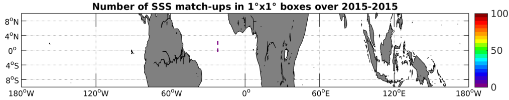
Figure 3: Number of SSS match-ups between Surface drifters SSS and the SMAP-L3-JPL-V4-8DAY-RUNNING-60KM SSS product for the Equatorial Ocean 10N-10S Pi-MEP region over 1^\circ \times 1^\circ boxes and for the full satellite product period.
