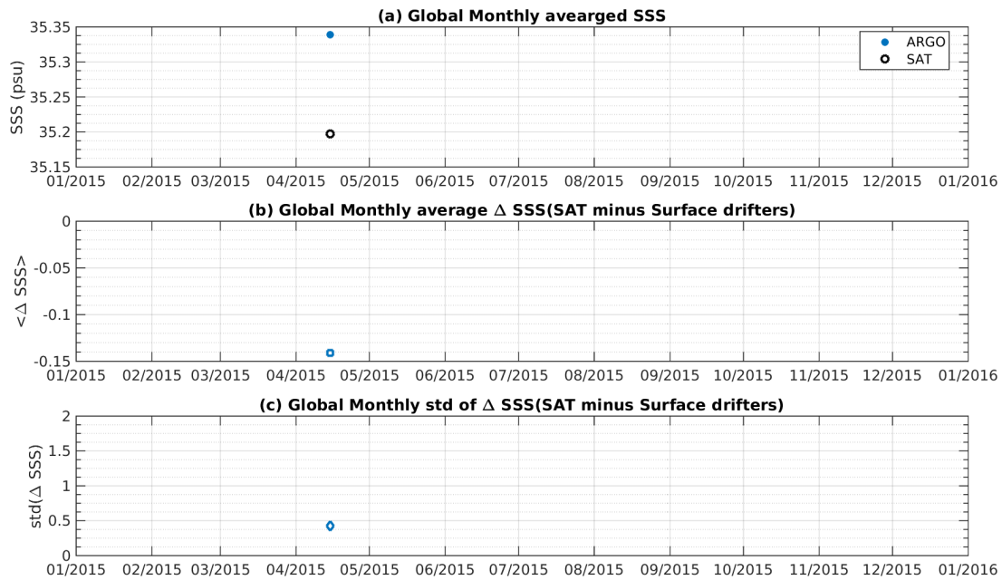
Figure 6: Time series of the monthly averaged mean SSS (top), mean \Delta SSS (Satellite - Surface drifters) and STD of \Delta SSS (Satellite - Surface drifters) over the Equatorial Ocean 10N-10S Pi-MEP region considering all match-ups collected by the Pi-MEP platform.
