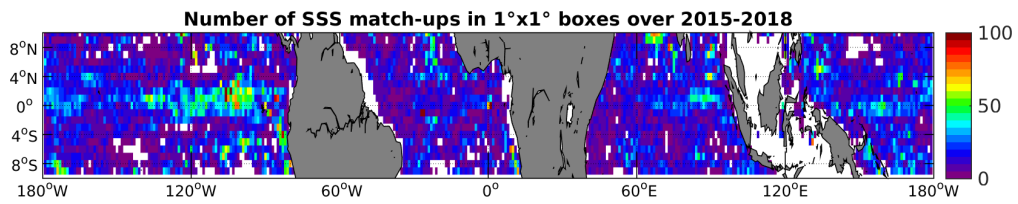
Figure 4: Number of SSS match-ups between Argo SSS and the SMAP-L3-JPL-V4-8DAY-RUNNING-60KM SSS product for the Equatorial Ocean 10N-10S Pi-MEP region over 1^\circ \times 1^\circ boxes and for the full satellite product period.
