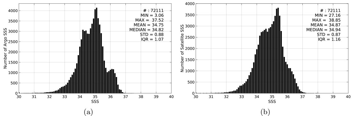
Figure 2: Histograms of SSS from Argo (a) and SMAP-L3-JPL-V4-8DAY-RUNNING-60KM (b) considering all match-up pairs per bins of 0.1 over the Equatorial Ocean 10N-10S Pi-MEP region and for the full satellite product period.
