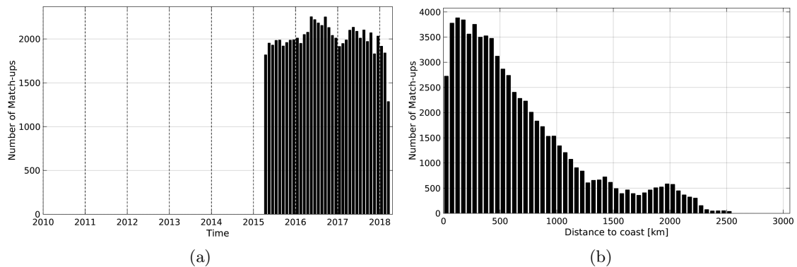
Figure 1: Number of match-ups between Argo and SMAP-L3-JPL-V4-8DAY-RUNNING-60KM SSS as a function of time (a) and as function of the distance to coast (b) over the Equatorial Ocean 10N-10S Pi-MEP region and for the full satellite product period.
