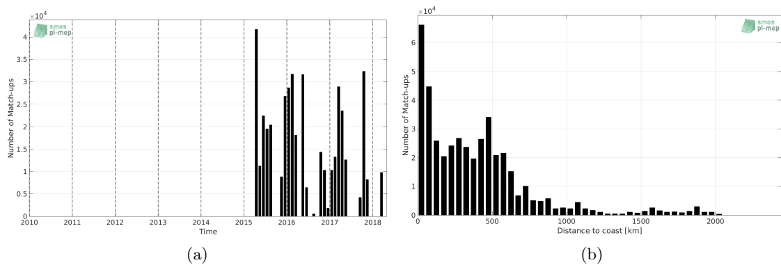
Figure 1: Number of match-ups between TSG-SAMOS and SMAP-L3-JPL-V4-MONTHLY-60KM SSS as a function of time (a) and as function of the distance to coast (b) over the Equatorial Ocean 10N-10S Pi-MEP region and for the full satellite product period.
