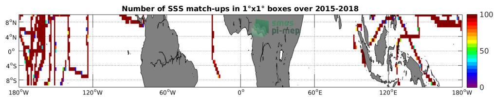
Figure 4: Number of SSS match-ups between TSG-SAMOS SSS and the SMAP-L3-JPL-V4-MONTHLY-60KM SSS product for the Equatorial Ocean 10N-10S Pi-MEP region over 1^\circ \times 1^\circ boxes and for the full satellite product period.
