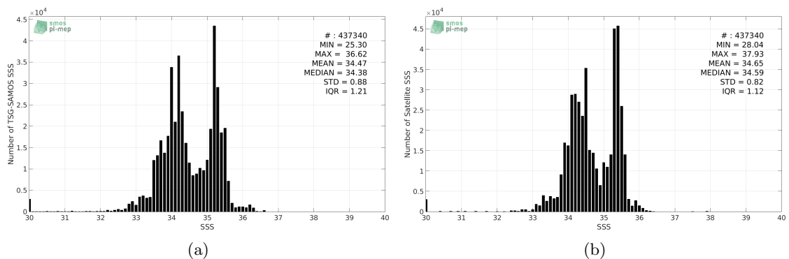
Figure 2: Histograms of SSS from TSG-SAMOS (a) and SMAP-L3-JPL-V4-MONTHLY-60KM (b) considering all match-up pairs per bins of 0.1 over the Equatorial Ocean 10N-10S Pi-MEP region and for the full satellite product period.
