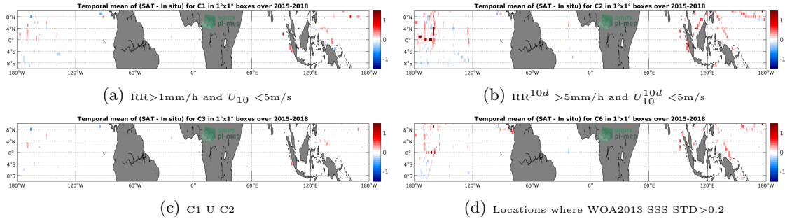
Figure 12: Temporal mean gridded over spatial boxes of size 1^\circ \times 1^\circ of \Delta SSS (SMAP-L3-JPL-V4-MONTHLY-60KM - TSG-SAMOS) for 4 different subdatasets corresponding to: RR > 1\text{mm/h} and U_{10} < 5\text{m/s} (a), RR^{10d} > 5\text{mm/h} and U_{10}^{10d} < 5\text{m/s} (b), C1 U C2 (c), Locations where WOA2013 SSS STD > 0.2 (d).
