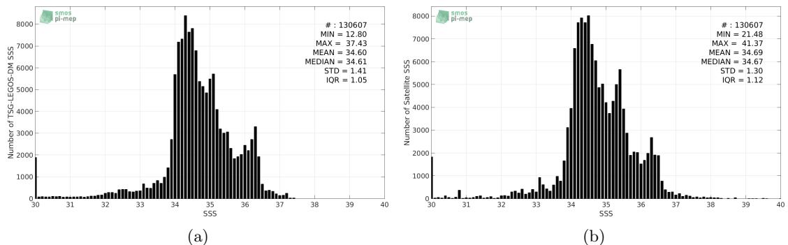
Figure 2: Histograms of SSS from TSG-LEGOS-DM (a) and SMAP-L3-JPL-V4-MONTHLY-60KM (b) considering all match-up pairs per bins of 0.1 over the Equatorial Ocean 10N-10S Pi-MEP region and for the full satellite product period.
