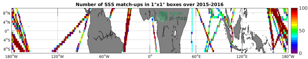
Figure 4: Number of SSS match-ups between TSG-LEGOS-DM SSS and the SMAP-L3-JPL-V4-MONTHLY-60KM SSS product for the Equatorial Ocean 10N-10S Pi-MEP region over 1^\circ \times 1^\circ boxes and for the full satellite product period.
