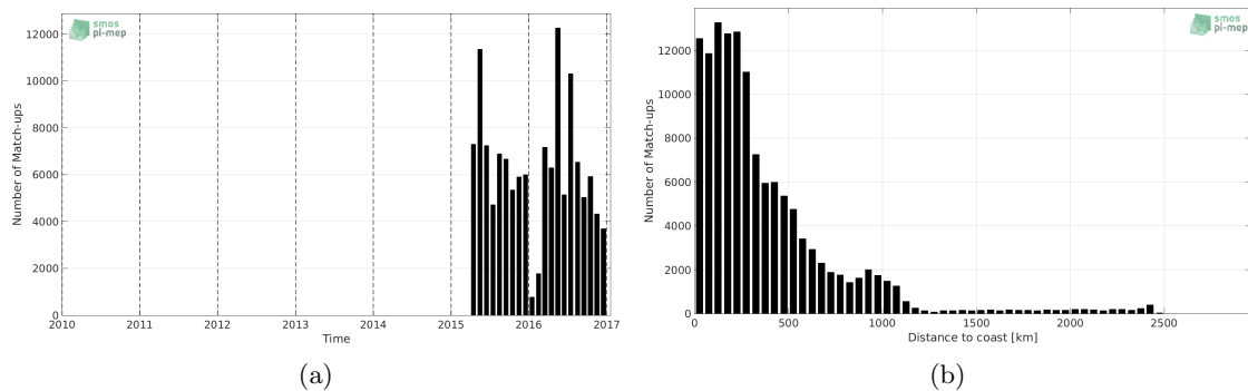
Figure 1: Number of match-ups between TSG-LEGOS-DM and SMAP-L3-JPL-V4-MONTHLY-60KM SSS as a function of time (a) and as function of the distance to coast (b) over the Equatorial Ocean 10N-10S Pi-MEP region and for the full satellite product period.
