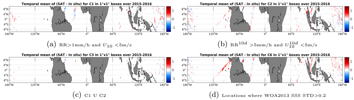
Figure 12: Temporal mean gridded over spatial boxes of size 1^\circ \times 1^\circ of \Delta SSS (SMAP-L3-JPL-V4-MONTHLY-60KM - TSG-LEGOS-DM) for 4 different subdatasets corresponding to: RR > 1\text{mm/h} and U_{10} < 5\text{m/s} (a), RR^{10d} > 5\text{mm/h} and U_{10}^{10d} < 5\text{m/s} (b), C1 U C2 (c), Locations where WOA2013 SSS STD > 0.2 (d).
