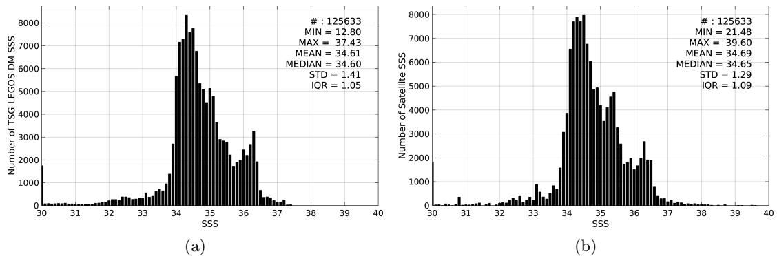
Figure 2: Histograms of SSS from TSG-LEGOS-DM (a) and SMAP-L3-JPL-V4-MONTHLY-60KM (b) considering all match-up pairs per bins of 0.1 over the Equatorial Ocean 10N-10S Pi-MEP region and for the full satellite product period.
