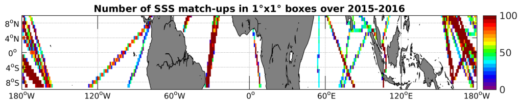
Figure 4: Number of SSS match-ups between TSG-LEGOS-DM SSS and the SMAP-L3-JPL-V4-MONTHLY-60KM SSS product for the Equatorial Ocean 10N-10S Pi-MEP region over 1^\circ \times 1^\circ boxes and for the full satellite product period.
