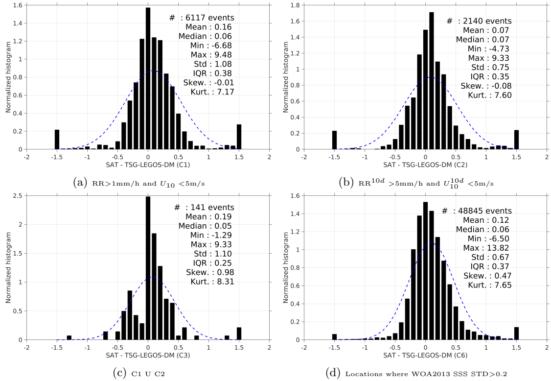
Figure 13: Normalized histogram of \Delta SSS (SMAP-L3-JPL-V4-MONTHLY-60KM - TSG-LEGOS-DM) for 6 different subdatasets corresponding to: RR > 1\text{mm/h} and U_{10} < 5\text{m/s} (a), RR^{10d} > 5\text{mm/h} and U_{10}^{10d} < 5\text{m/s} (b), C1 \cup C2 (c), Locations where WOA2013 SSS STD > 0.2 (d).
