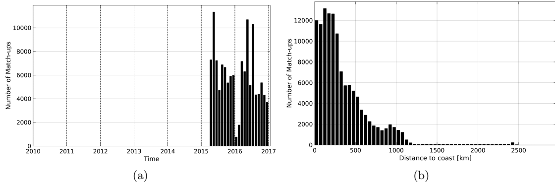
Figure 1: Number of match-ups between TSG-LEGOS-DM and SMAP-L3-JPL-V4-MONTHLY-60KM SSS as a function of time (a) and as function of the distance to coast (b) over the Equatorial Ocean 10N-10S Pi-MEP region and for the full satellite product period.
