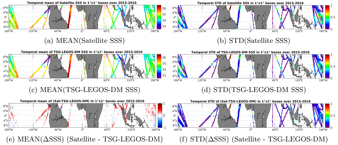
Figure 6: Temporal mean (left) and STD (right) of SSS from SMAP-L3-JPL-V4-MONTHLY-60KM (top), TSG-LEGOS-DM (middle), and of \Delta SSS (Satellite - TSG-LEGOS-DM). Only match-up pairs are used to generate these maps.
