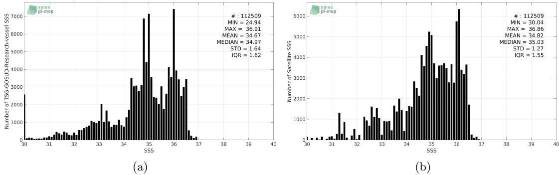
Figure 2: Histograms of SSS from TSG-GOSUD-Research-vessel (a) and SMAP-L3-JPL-V4-MONTHLY-60KM (b) considering all match-up pairs per bins of 0.1 over the Equatorial Ocean 10N-10S Pi-MEP region and for the full satellite product period.
