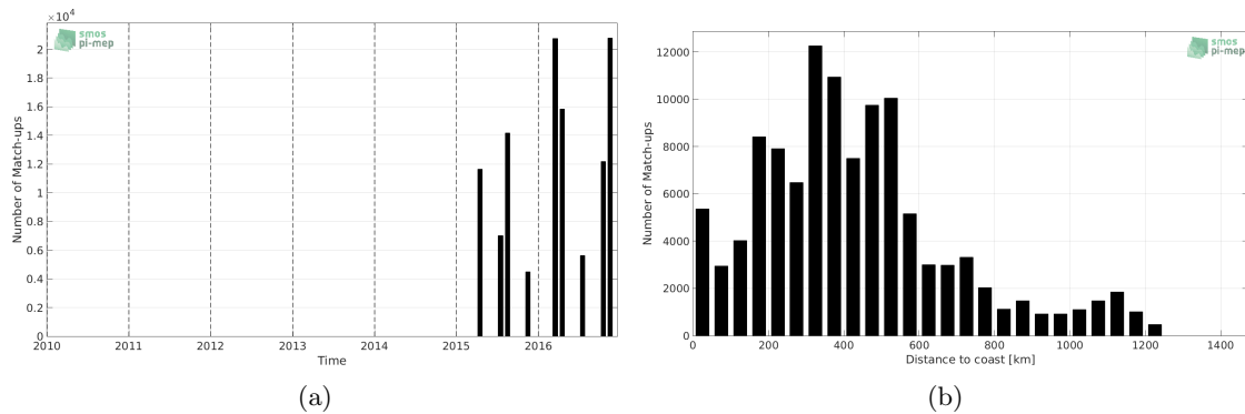
Figure 1: Number of match-ups between TSG-GOSUD-Research-vessel and SMAP-L3-JPL-V4-MONTHLY-60KM SSS as a function of time (a) and as function of the distance to coast (b) over the Equatorial Ocean 10N-10S Pi-MEP region and for the full satellite product period.
