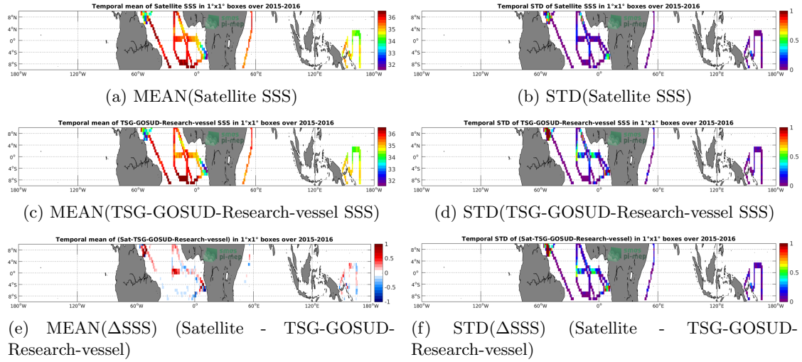
Figure 6: Temporal mean (left) and STD (right) of SSS from SMAP-L3-JPL-V4-MONTHLY-60KM (top), TSG-GOSUD-Research-vessel (middle), and of \Delta SSS (Satellite - TSG-GOSUD-Research-vessel). Only match-up pairs are used to generate these maps.
