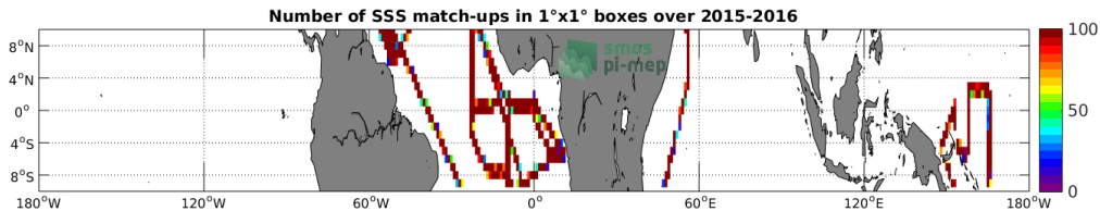
Figure 4: Number of SSS match-ups between TSG-GOSUD-Research-vessel SSS and the SMAP-L3-JPL-V4-MONTHLY-60KM SSS product for the Equatorial Ocean 10N-10S Pi-MEP region over 1°x1° boxes and for the full satellite product period.
