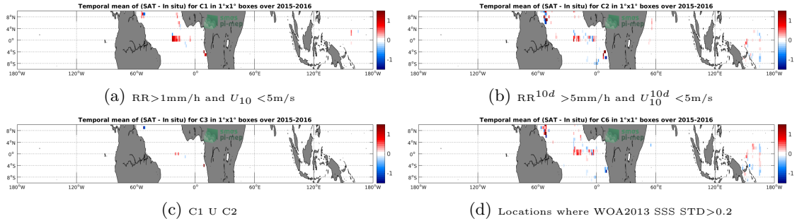
Figure 12: Temporal mean gridded over spatial boxes of size 1^\circ \times 1^\circ of \Delta SSS (SMAP-L3-JPL-V4-MONTHLY-60KM - TSG-GOSUD-Research-vessel) for 4 different subdatasets corresponding to: RR > 1\text{mm/h} and U_{10} < 5\text{m/s} (a), RR^{10d} > 5\text{mm/h} and U_{10}^{10d} < 5\text{m/s} (b), C1 U C2 (c), Locations where WOA2013 SSS STD > 0.2 (d).
