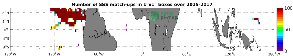
Figure 3: Number of SSS match-ups between Surface drifters SSS and the SMAP-L3-JPL-V4-MONTHLY-60KM SSS product for the Equatorial Ocean 10N-10S Pi-MEP region over 1°x1° boxes and for the full satellite product period.
