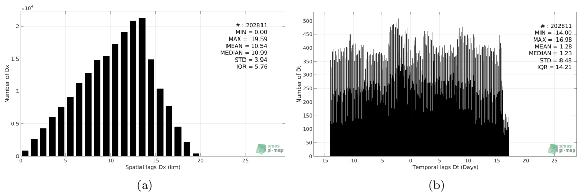
Figure 4: Histograms of the spatial (a) and temporal (b) lags between the time of the Surface drifters measurements and the date of the corresponding SMAP-L3-JPL-V4-MONTHLY-60KM SSS product.
