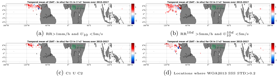
Figure 11: Temporal mean gridded over spatial boxes of size 1^\circ \times 1^\circ of \Delta SSS (SMAP-L3-JPL-V4-MONTHLY-60KM - Surface drifters) for 4 different subdatasets corresponding to: RR > 1\text{mm/h} and U_{10} < 5\text{m/s} (a), RR^{10d} > 5\text{mm/h} and U_{10}^{10d} < 5\text{m/s} (b), C1 U C2 (c), Locations where WOA2013 SSS STD > 0.2 (d).
