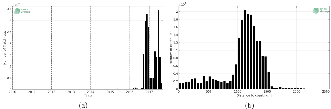
Figure 1: Number of match-ups between Surface drifters and SMAP-L3-JPL-V4-MONTHLY-60KM SSS as a function of time (a) and as function of the distance to coast (b) over the Equatorial Ocean 10N-10S Pi-MEP region and for the full satellite product period.
