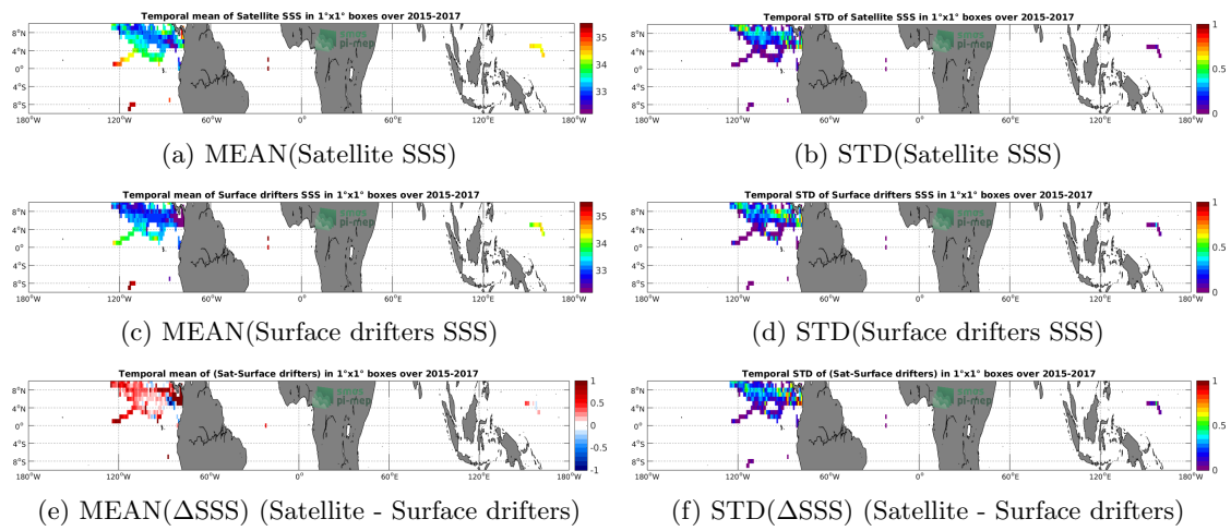
Figure 5: Temporal mean (left) and STD (right) of SSS from SMAP-L3-JPL-V4-MONTHLY-60KM (top), Surface drifters (middle), and of \Delta SSS (Satellite - Surface drifters). Only match-up pairs are used to generate these maps.
