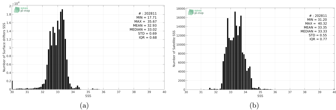
Figure 2: Histograms of SSS from Surface drifters (a) and SMAP-L3-JPL-V4-MONTHLY-60KM (b) considering all match-up pairs per bins of 0.1 over the Equatorial Ocean 10N-10S Pi-MEP region and for the full satellite product period.
