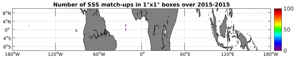
Figure 3: Number of SSS match-ups between Surface drifters SSS and the SMAP-L3-JPL-V4-MONTHLY-60KM SSS product for the Equatorial Ocean 10N-10S Pi-MEP region over 1^\circ \times 1^\circ boxes and for the full satellite product period.
