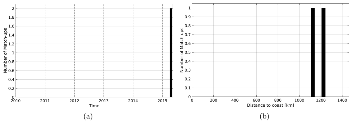
Figure 1: Number of match-ups between Surface drifters and SMAP-L3-JPL-V4-MONTHLY-60KM SSS as a function of time (a) and as function of the distance to coast (b) over the Equatorial Ocean 10N-10S Pi-MEP region and for the full satellite product period.
