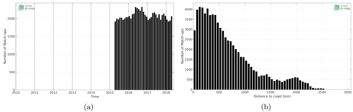
Figure 1: Number of match-ups between Argo and SMAP-L3-JPL-V4-MONTHLY-60KM SSS as a function of time (a) and as function of the distance to coast (b) over the Equatorial Ocean 10N-10S Pi-MEP region and for the full satellite product period.
