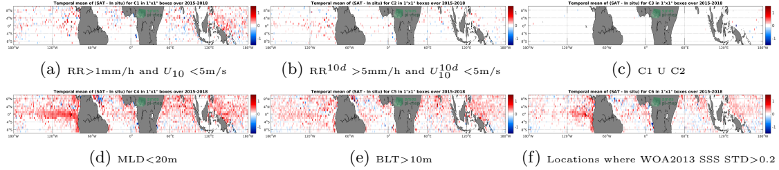
Figure 12: Temporal mean gridded over spatial boxes of size 1^\circ \times 1^\circ of \Delta SSS (SMAP-L3-JPL-V4-MONTHLY-60KM - Argo) for 6 different subdatasets corresponding to:RR>1mm/h and U_{10} < 5\text{m/s} (a), RR^{10d} > 5\text{mm/h} and U_{10}^{10d} < 5\text{m/s} (b), C1 U C2 (c),MLD<20m (d),BLT>10m (e),Locations where WOA2013 SSS STD>0.2 (f).
