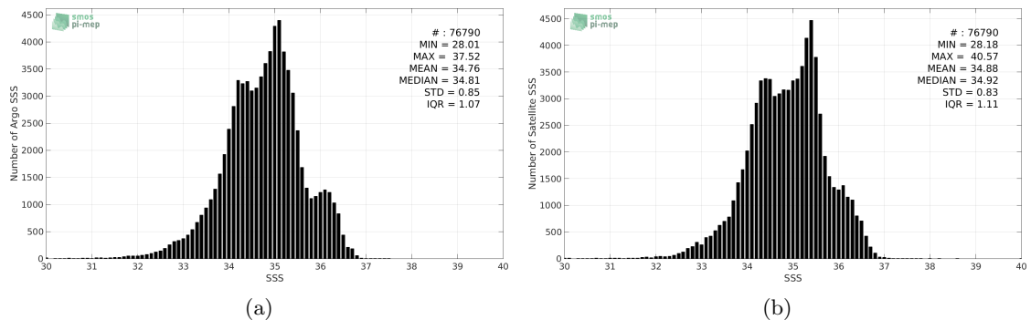
Figure 2: Histograms of SSS from Argo (a) and SMAP-L3-JPL-V4-MONTHLY-60KM (b) considering all match-up pairs per bins of 0.1 over the Equatorial Ocean 10N-10S Pi-MEP region and for the full satellite product period.
