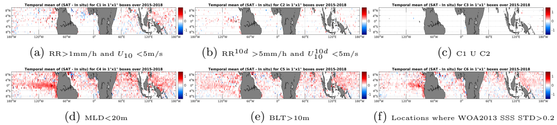
Figure 12: Temporal mean gridded over spatial boxes of size 1^\circ \times 1^\circ of \Delta\text{SSS} (SMAP-L3-JPL-V4-MONTHLY-60KM - Argo) for 6 different subdatasets corresponding to: RR>1mm/h and U_{10} < 5\text{m/s} (a), \text{RR}^{10d} > 5\text{mm/h} and U_{10}^{10d} < 5\text{m/s} (b), C1 U C2 (c),MLD<20m (d),BLT>10m (e),Locations where WOA2013 SSS STD>0.2 (f).
