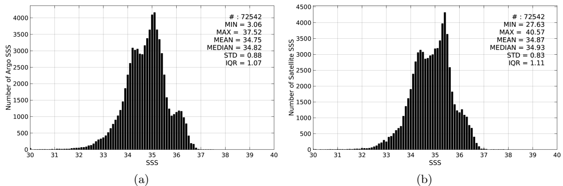
Figure 2: Histograms of SSS from Argo (a) and SMAP-L3-JPL-V4-MONTHLY-60KM (b) considering all match-up pairs per bins of 0.1 over the Equatorial Ocean 10N-10S Pi-MEP region and for the full satellite product period.
