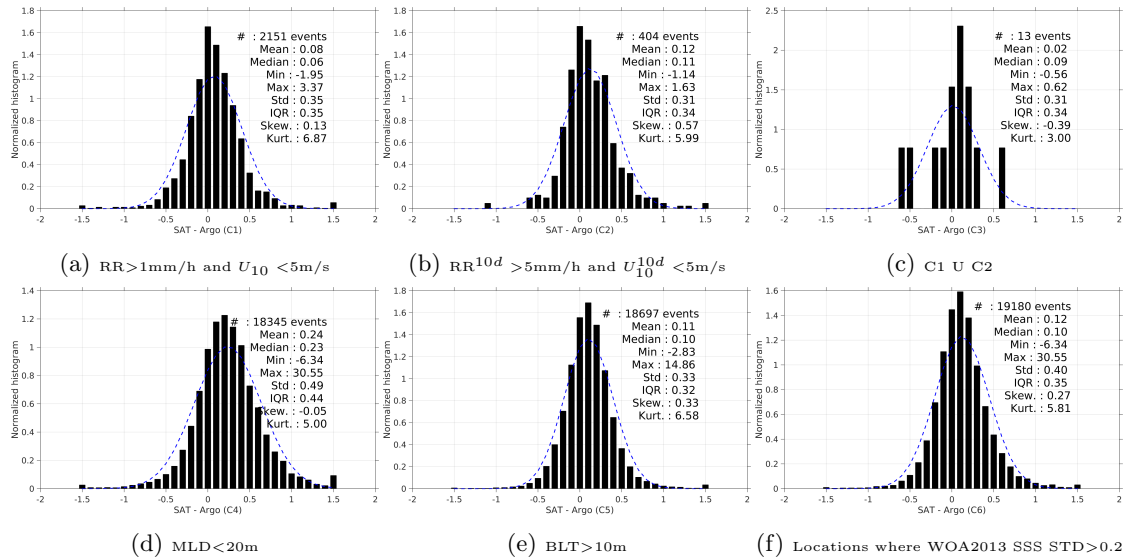
Figure 13: Normalized histogram of \Delta\text{SSS} (SMAP-L3-JPL-V4-MONTHLY-60KM - Argo) for 6 different subdatasets corresponding to: RR>1mm/h and U_{10} < 5\text{m/s} (a), \text{RR}^{10d} > 5\text{mm/h} and U_{10}^{10d} < 5\text{m/s} (b), C1 U C2 (c),MLD<20m (d),BLT>10m (e),Locations where WOA2013 SSS STD>0.2 (f).
