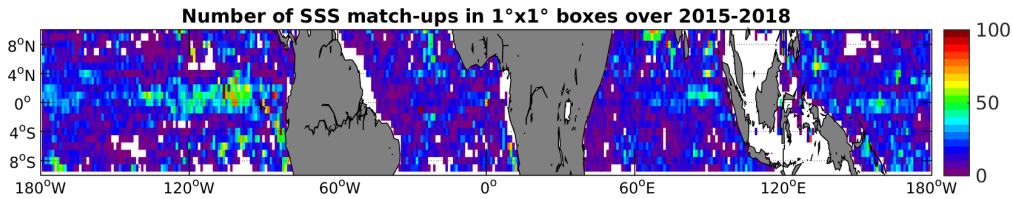
Figure 4: Number of SSS match-ups between Argo SSS and the SMAP-L3-JPL-V4-MONTHLY-60KM SSS product for the Equatorial Ocean 10N-10S Pi-MEP region over 1°x1° boxes and for the full satellite product period.
