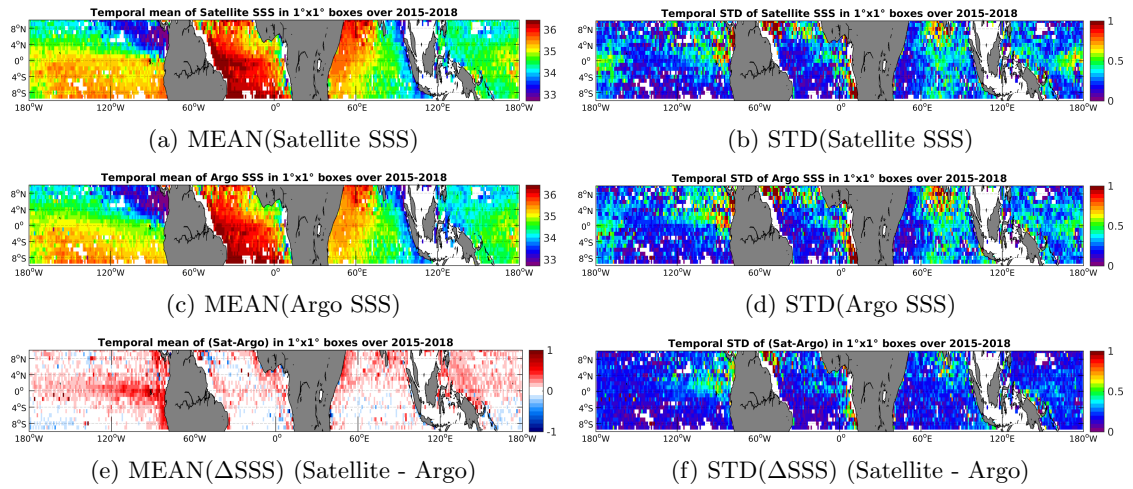
Figure 6: Temporal mean (left) and STD (right) of SSS from SMAP-L3-JPL-V4-MONTHLY-60KM (top), Argo (middle), and of \Delta SSS (Satellite - Argo). Only match-up pairs are used to generate these maps.
