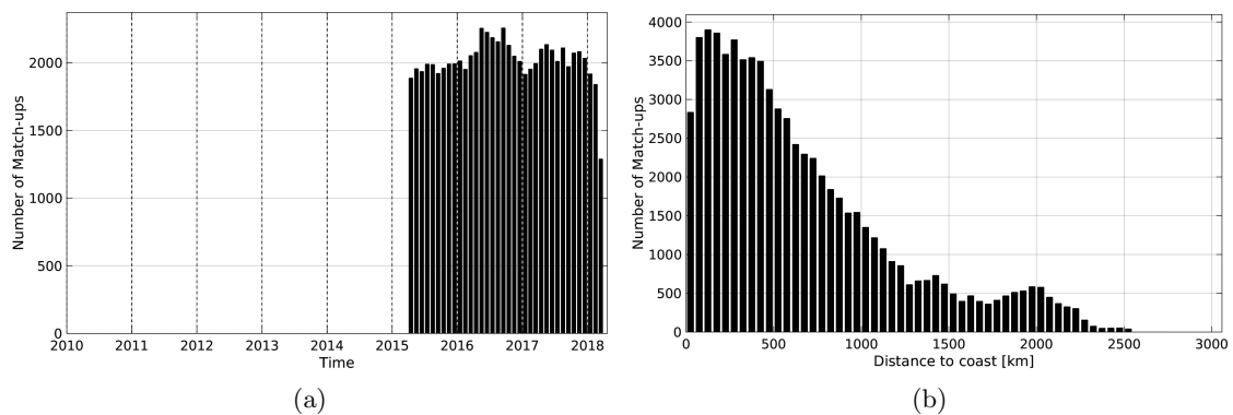
Figure 1: Number of match-ups between Argo and SMAP-L3-JPL-V4-MONTHLY-60KM SSS as a function of time (a) and as function of the distance to coast (b) over the Equatorial Ocean 10N-10S Pi-MEP region and for the full satellite product period.
