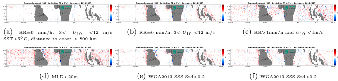
Figure 12: Temporal mean gridded over spatial boxes of size 1^\circ \times 1^\circ of \Delta SSS (SMAP SSS L2-AVERAGED v5 (RSS) - Argo) for 6 different subdatasets corresponding to:RR=0 mm/h, 3 < U_{10} < 12 m/s, SST >5^\circ\text{C} , distance to coast > 800 km (a), RR=0 mm/h, 3 < U_{10} < 12 m/s (b), RR >1 mm/h and U_{10} < 4 m/s (c),MLD <20 m (d),WOA2013 SSS Std <0.2 (e),WOA2013 SSS Std >0.2 (f).
