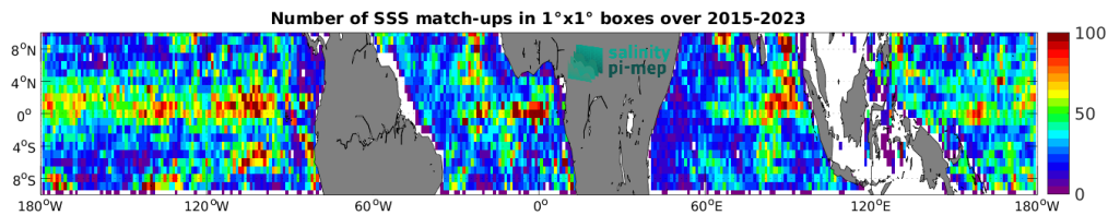
Figure 4: Number of SSS match-ups between Argo SSS and the SMAP SSS L2-AVERAGED v5 (RSS) SSS product for the Equatorial Ocean 10N-10S Pi-MEP region over 1^\circ \times 1^\circ boxes and for the full satellite product period.
