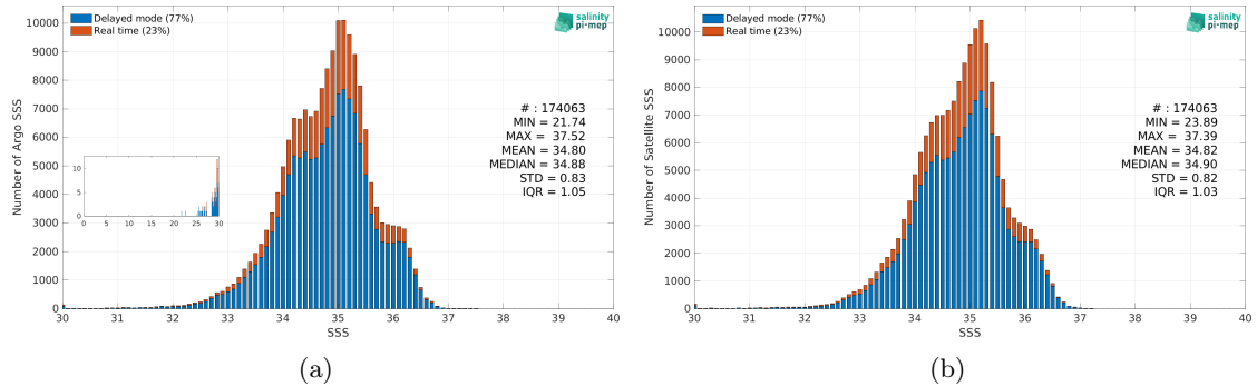
Figure 2: Histograms of SSS from Argo (a) and SMAP SSS L2-AVERAGED v5 (RSS) (b) considering all match-up pairs per bins of 0.1 over the Equatorial Ocean 10N-10S Pi-MEP region and for the full satellite product period.
