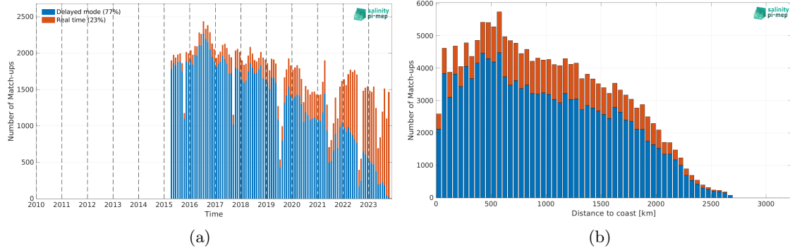
Figure 1: Number of match-ups between Argo and SMAP SSS L2-AVERAGED v5 (RSS) SSS as a function of time (a) and as function of the distance to coast (b) over the Equatorial Ocean 10N-10S Pi-MEP region and for the full satellite product period.
