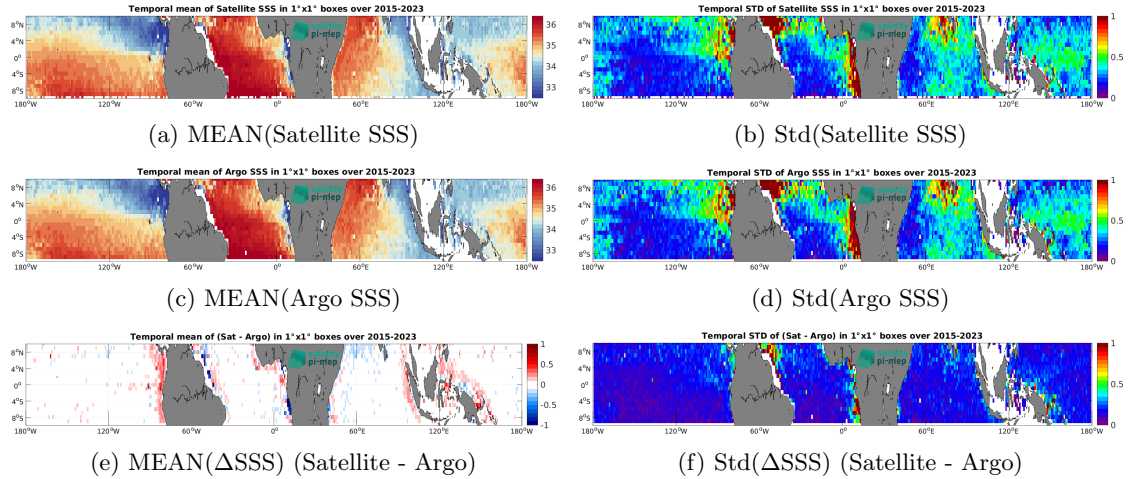
Figure 6: Temporal mean (left) and Std (right) of SSS from SMAP SSS L2-AVERAGED v5 (RSS) (top), Argo (middle), and of \Delta SSS (Satellite - Argo). Only match-up pairs are used to generate these maps.
