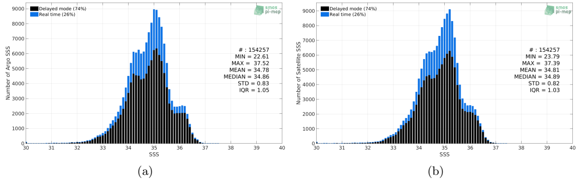
Figure 2: Histograms of SSS from Argo (a) and SMAP SSS L2-AVERAGED v5 (RSS) (b) considering all match-up pairs per bins of 0.1 over the Equatorial Ocean 10N-10S Pi-MEP region and for the full satellite product period.
