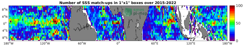
Figure 4: Number of SSS match-ups between Argo SSS and the SMAP SSS L2-AVERAGED v5.0 (JPL) SSS product for the Equatorial Ocean 10N-10S Pi-MEP region over 1^\circ \times 1^\circ boxes and for the full satellite product period.
