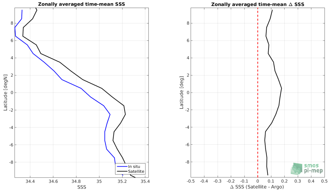
Figure 8: Left panel: Zonal mean SSS from SMAP SSS L2-AVERAGED v5.0 (JPL) satellite product (black) and from Argo (blue). Right panel: Zonal mean of \Delta SSS (Satellite - Argo) for all the collected Pi-MEP match-up pairs estimated over the full satellite product period.
