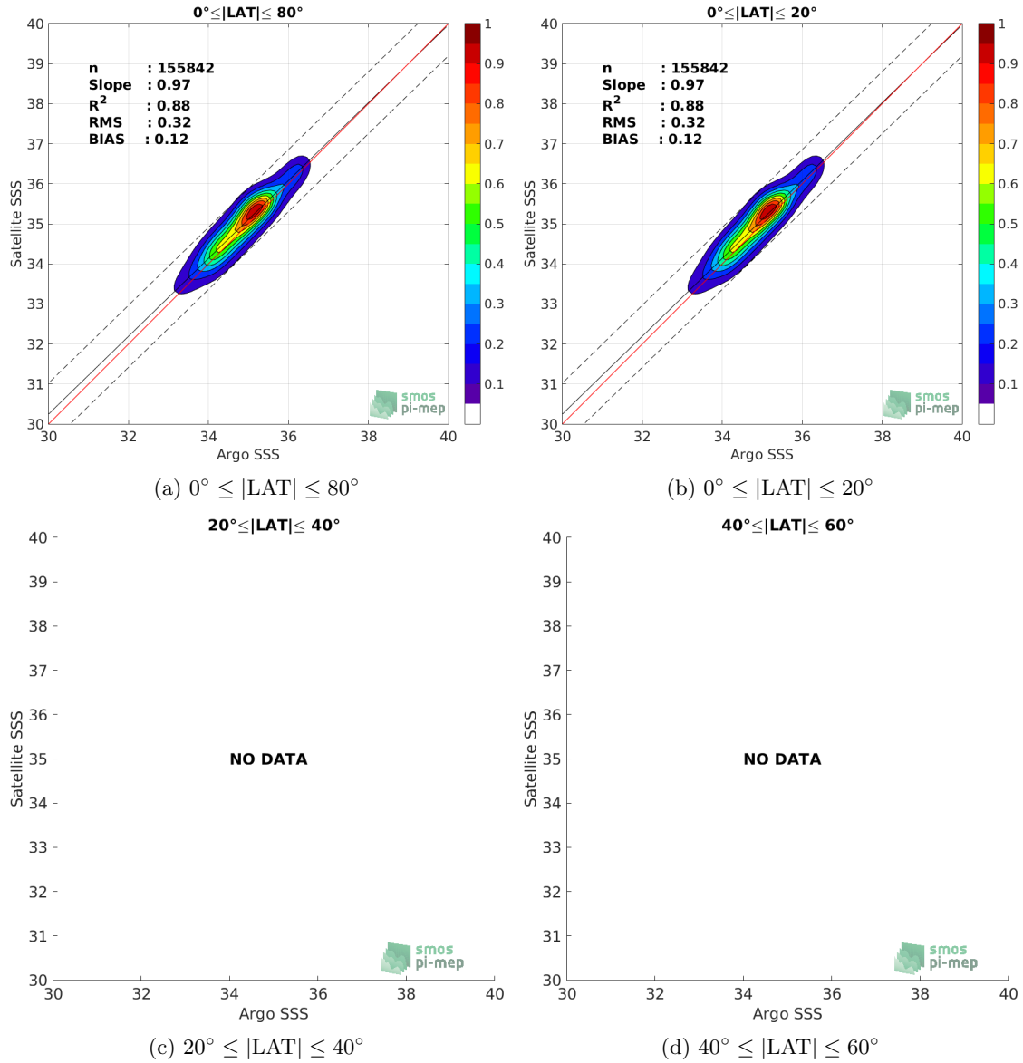
Figure 9: Contour maps of the concentration of SMAP SSS L2-AVERAGED v5.0 (JPL) SSS (y-axis) versus Argo SSS (x-axis) at match-up pairs for different latitude bands. For each plot, the red line shows x=y . The black thin and dashed lines indicate a linear fit through the data cloud and the \pm 95\% confidence levels, respectively. The number match-up pairs n , the slope and R^2 coefficient of the linear fit, the root mean square (RMS) and the mean bias between satellite and in situ data are indicated for each latitude band in each plots.
