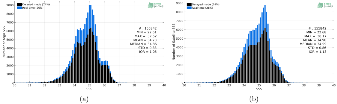
Figure 2: Histograms of SSS from Argo (a) and SMAP SSS L2-AVERAGED v5.0 (JPL) (b) considering all match-up pairs per bins of 0.1 over the Equatorial Ocean 10N-10S Pi-MEP region and for the full satellite product period.
