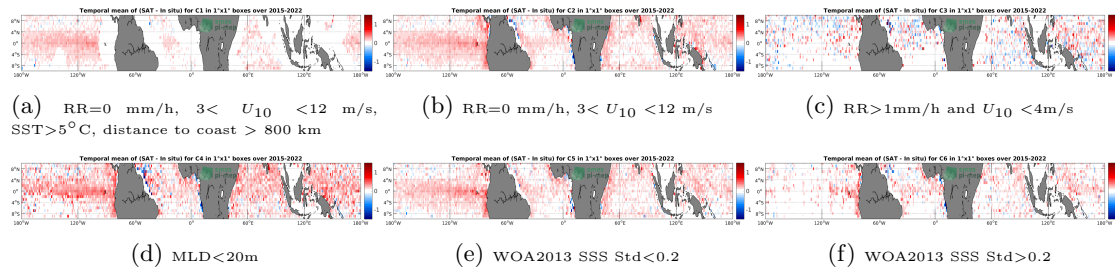
Figure 12: Temporal mean gridded over spatial boxes of size 1^\circ \times 1^\circ of \Delta SSS (SMAP SSS L2-AVERAGED v5.0 (JPL) - Argo) for 6 different subdatasets corresponding to:RR=0 mm/h, 3 < U_{10} < 12 m/s, SST >5^\circ C, distance to coast > 800 km (a), RR=0 mm/h, 3 < U_{10} < 12 m/s (b), RR >1 mm/h and U_{10} < 4 m/s (c),MLD <20 m (d),WOA2013 SSS Std <0.2 (e),WOA2013 SSS Std >0.2 (f).
