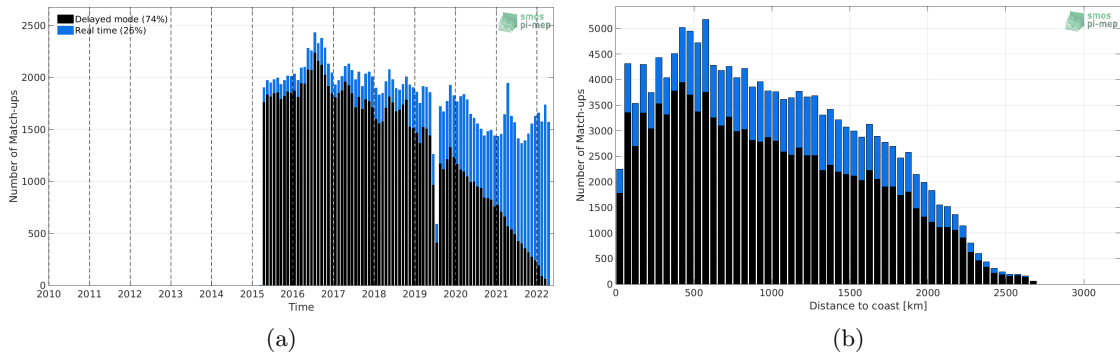
Figure 1: Number of match-ups between Argo and SMAP SSS L2-AVERAGED v5.0 (JPL) SSS as a function of time (a) and as function of the distance to coast (b) over the Equatorial Ocean 10N-10S Pi-MEP region and for the full satellite product period.
