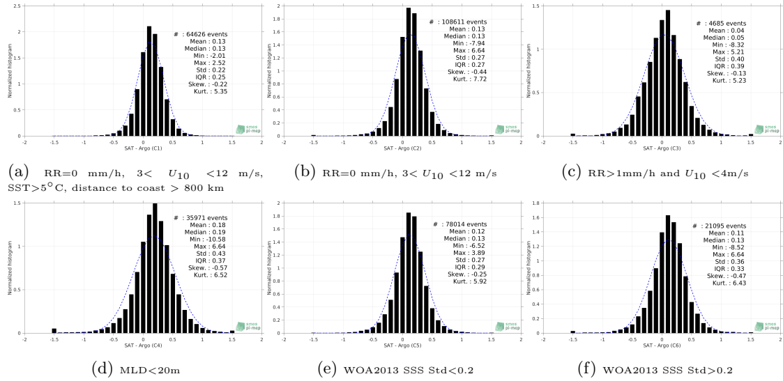
Figure 13: Normalized histogram of \Delta SSS (SMAP SSS L2-AVERAGED v5.0 (JPL) - Argo) for 6 different subdatasets corresponding to: RR=0 mm/h, 3 < U_{10} < 12 m/s, SST>5°C, distance to coast > 800 km (a), RR=0 mm/h, 3 < U_{10} < 12 m/s (b), RR>1mm/h and U_{10} < 4 m/s (c), MLD<20m (d), WOA2013 SSS Std<0.2 (e), WOA2013 SSS Std>0.2 (f).
