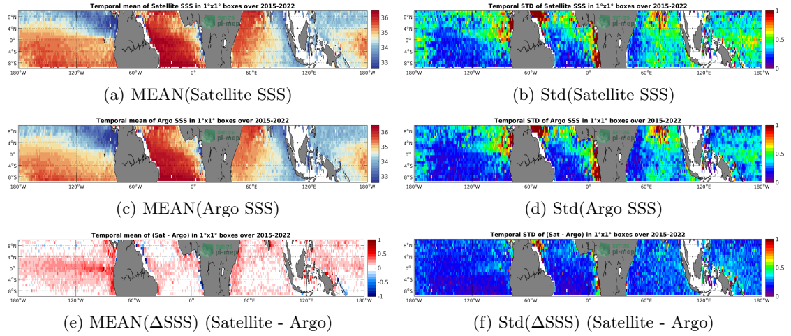
Figure 6: Temporal mean (left) and Std (right) of SSS from SMAP SSS L2-AVERAGED v5.0 (JPL) (top), Argo (middle), and of \Delta SSS (Satellite - Argo). Only match-up pairs are used to generate these maps.
