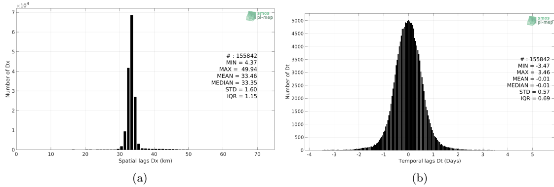
Figure 5: Histograms of the spatial (a) and temporal (b) lags between the location/time of the Argo measurement and the date of the corresponding SMAP SSS L2-AVERAGED v5.0 (JPL) SSS pixel.
