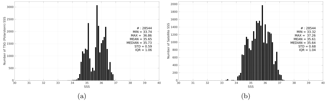
Figure 3: Histograms of SSS from TSG (Polarstern) (a) and SMAP SSS L2 v6 (RSS) (b) considering all match-up pairs per bins of 0.1 over the Equatorial Ocean 10N-10S Pi-MEP region and for the full satellite product period.
