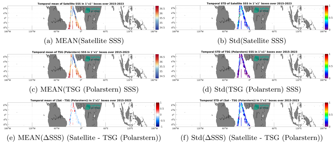
Figure 7: Temporal mean (left) and Std (right) of SSS from SMAP SSS L2 v6 (RSS) (top), TSG (Polarstern) (middle), and of \Delta SSS (Satellite - TSG (Polarstern)). Only match-up pairs are used to generate these maps.
