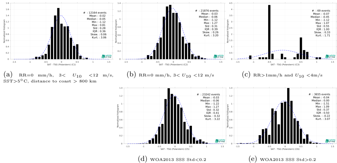
Figure 15: Normalized histogram of \Delta SSS (SMAP SSS L2 v6 (RSS) - TSG (Polarstern)) for 5 different subdatasets corresponding to: RR=0 mm/h, 3 < U_{10} < 12 m/s, SST>5°C, distance to coast > 800 km (a), RR=0 mm/h, 3 < U_{10} < 12 m/s (b), RR>1mm/h and U_{10} < 4 m/s (c), WOA2013 SSS Std<0.2 (d), WOA2013 SSS Std>0.2 (e).
