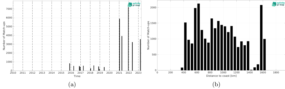
Figure 2: Number of match-ups between TSG (Polarstern) and SMAP SSS L2 v6 (RSS) SSS as a function of time (a) and as function of the distance to coast (b) over the Equatorial Ocean 10N-10S Pi-MEP region and for the full satellite product period.
