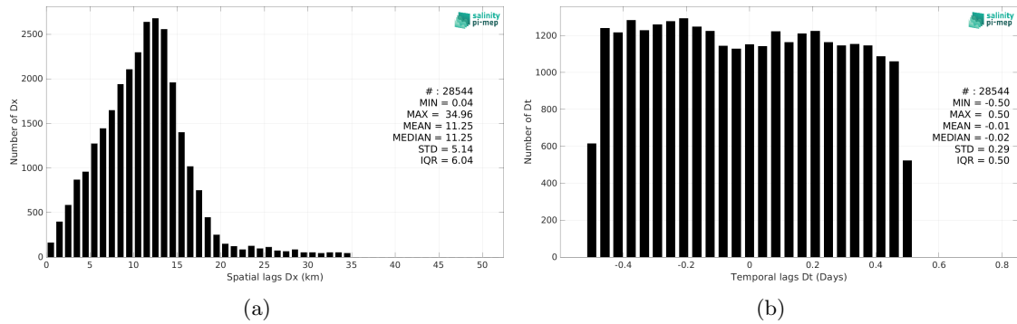
Figure 6: Histograms of the spatial (a) and temporal (b) lags between the location/time of the TSG (Polarstern) measurement and the date of the corresponding SMAP SSS L2 v6 (RSS) SSS pixel.
