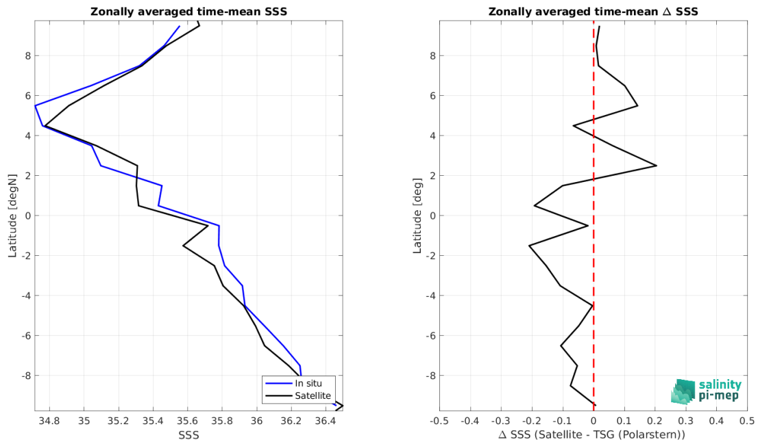
Figure 9: Left panel: Zonal mean SSS from SMAP SSS L2 v6 (RSS) satellite product (black) and from TSG (Polarstern) (blue). Right panel: Zonal mean of \Delta SSS (Satellite - TSG (Polarstern)) for all the collected Pi-MEP match-up pairs estimated over the full satellite product period.
