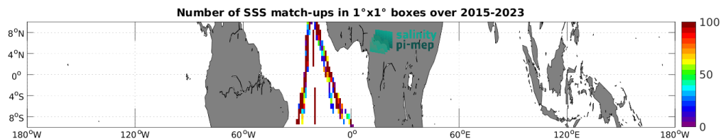
Figure 5: Number of SSS match-ups between TSG (Polarstern) SSS and the SMAP SSS L2 v6 (RSS) SSS product for the Equatorial Ocean 10N-10S Pi-MEP region over 1^\circ \times 1^\circ boxes and for the full satellite product period.
