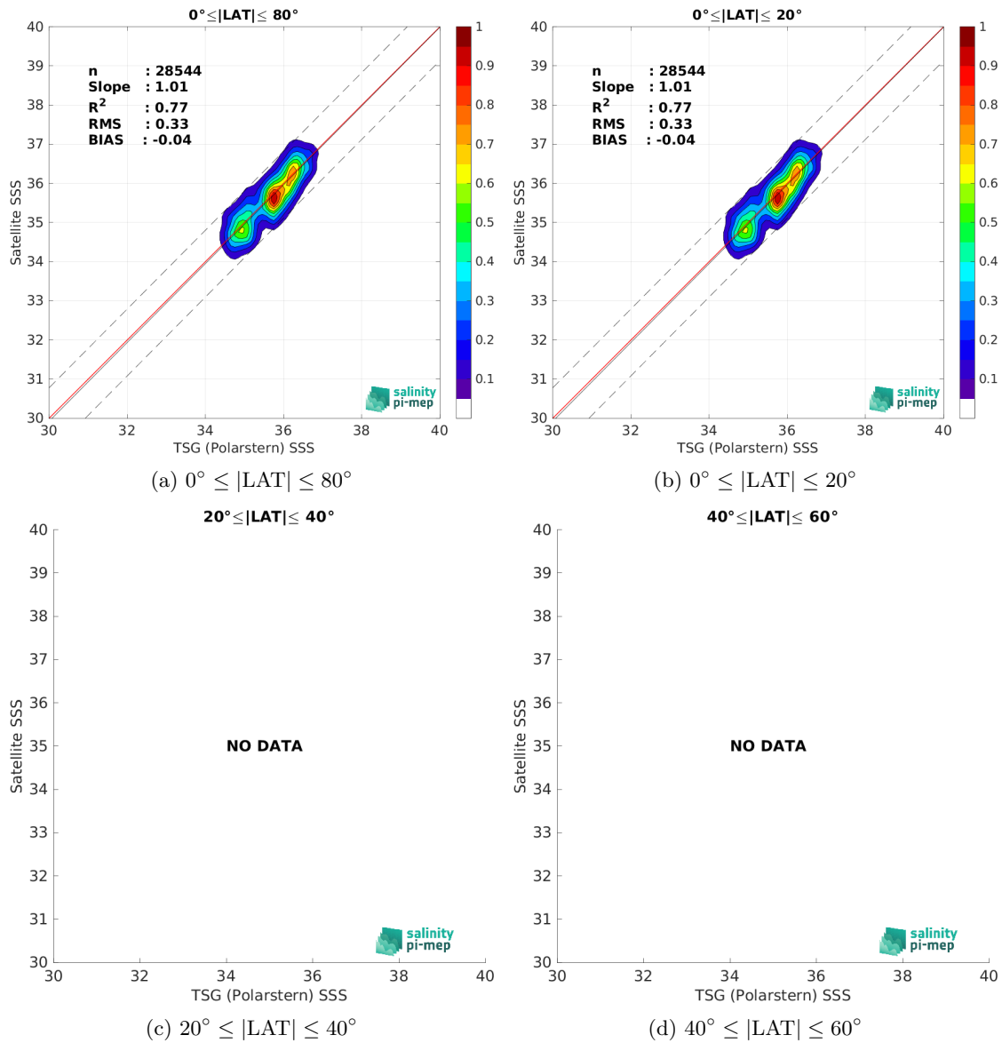
Figure 10: Contour maps of the concentration of SMAP SSS L2 v6 (RSS) SSS (y-axis) versus TSG (Polarstern) SSS (x-axis) at match-up pairs for different latitude bands. For each plot, the red line shows x=y . The black thin and dashed lines indicate a linear fit through the data cloud and the \pm 95\% confidence levels, respectively. The number match-up pairs n , the slope and R^2 coefficient of the linear fit, the root mean square (RMS) and the mean bias between satellite and in situ data are indicated for each latitude band in each plots.
