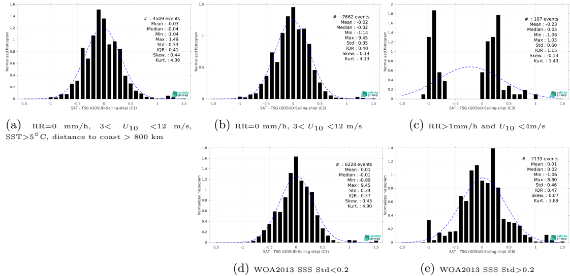
Figure 15: Normalized histogram of \Delta\text{SSS} (SMAP SSS L2 v6 (RSS) - TSG (GOSUD-Sailing-ship)) for 5 different subdatasets corresponding to: RR=0 mm/h, 3 < U_{10} < 12 m/s, SST>5°C, distance to coast > 800 km (a), RR=0 mm/h, 3 < U_{10} < 12 m/s (b), RR>1mm/h and U_{10} < 4 m/s (c), WOA2013 SSS Std<0.2 (d), WOA2013 SSS Std>0.2 (e).
