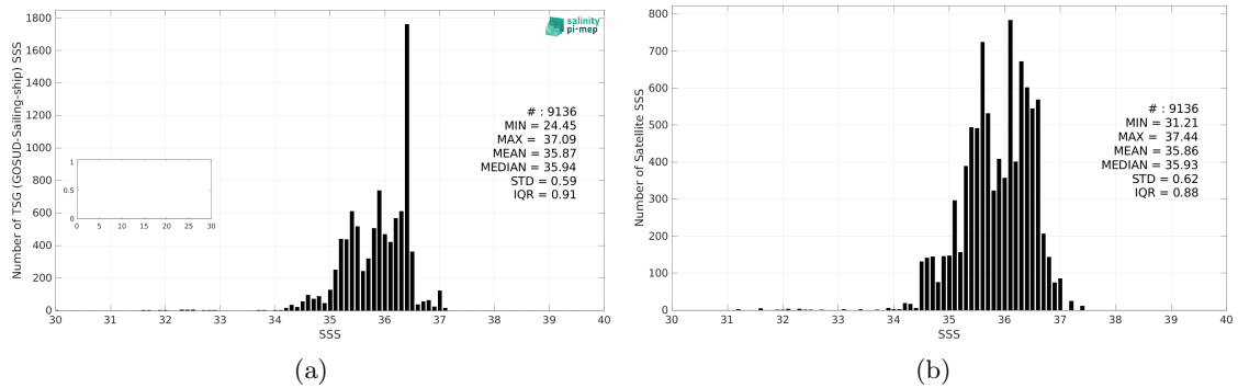
Figure 3: Histograms of SSS from TSG (GOSUD-Sailing-ship) (a) and SMAP SSS L2 v6 (RSS) (b) considering all match-up pairs per bins of 0.1 over the Equatorial Ocean 10N-10S Pi-MEP region and for the full satellite product period.
