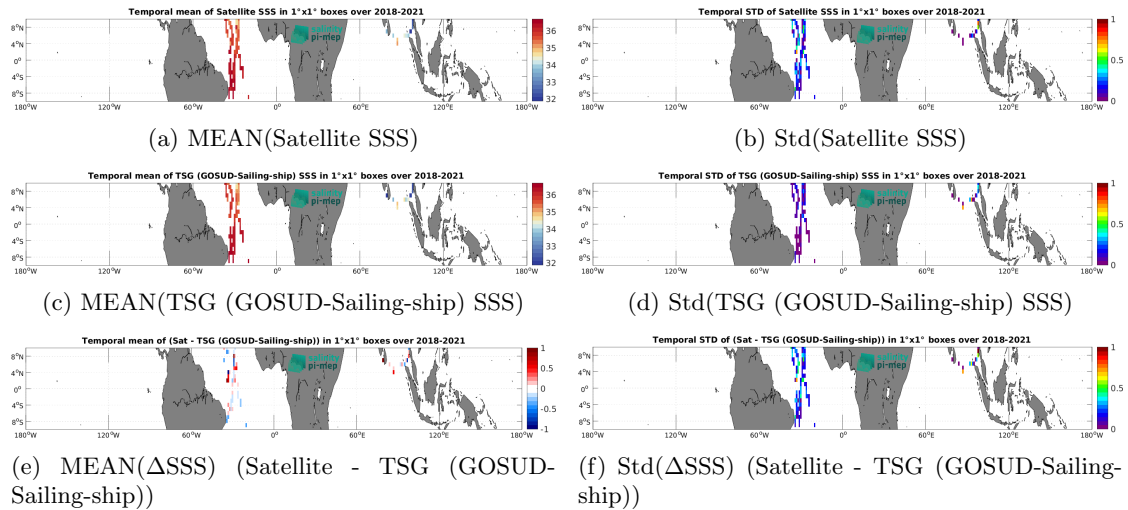
Figure 7: Temporal mean (left) and Std (right) of SSS from SMAP SSS L2 v6 (RSS) (top), TSG (GOSUD-Sailing-ship) (middle), and of \Delta SSS (Satellite - TSG (GOSUD-Sailing-ship)). Only match-up pairs are used to generate these maps.
