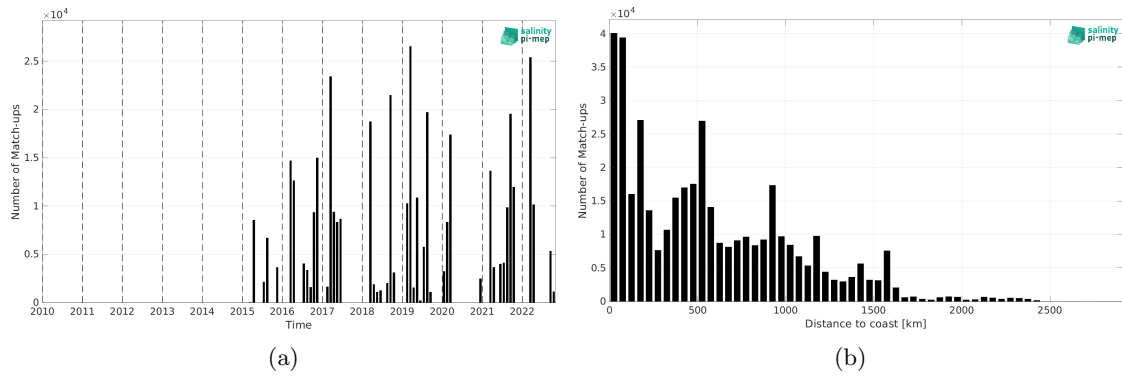
Figure 2: Number of match-ups between TSG (GOSUD-Research-vessel) and SMAP SSS L2 v6 (RSS) SSS as a function of time (a) and as function of the distance to coast (b) over the Equatorial Ocean 10N-10S Pi-MEP region and for the full satellite product period.
