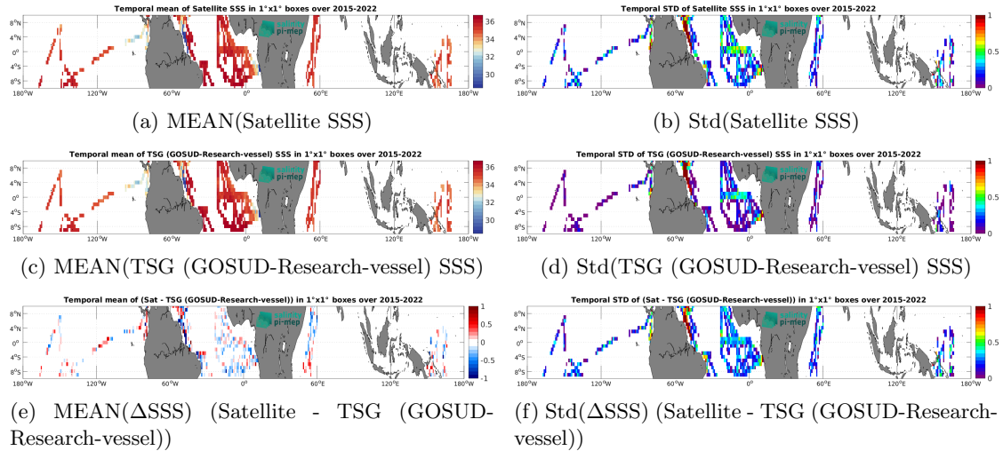
Figure 7: Temporal mean (left) and Std (right) of SSS from SMAP SSS L2 v6 (RSS) (top), TSG (GOSUD-Research-vessel) (middle), and of \Delta SSS (Satellite - TSG (GOSUD-Research-vessel)). Only match-up pairs are used to generate these maps.
