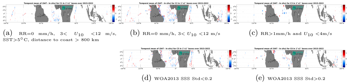
Figure 14: Temporal mean gridded over spatial boxes of size 1^\circ \times 1^\circ of \Delta SSS (SMAP SSS L2 v6 (RSS) - TSG (GOSUD-Research-vessel)) for 5 different subdatasets corresponding to:RR=0 mm/h, 3 < U_{10} < 12 m/s, SST>5°C, distance to coast > 800 km (a), RR=0 mm/h, 3 < U_{10} < 12 m/s (b), RR>1mm/h and U_{10} < 4 m/s (c), WOA2013 SSS Std<0.2 (d), WOA2013 SSS Std>0.2 (e).
