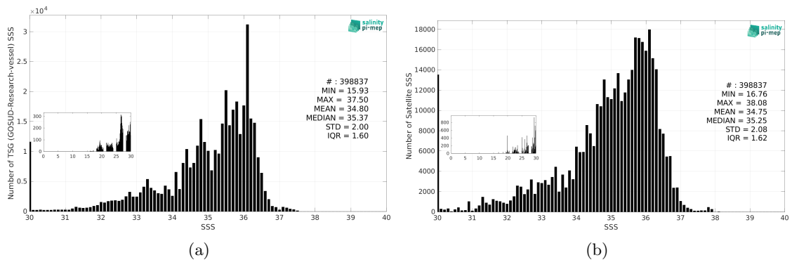
Figure 3: Histograms of SSS from TSG (GOSUD-Research-vessel) (a) and SMAP SSS L2 v6 (RSS) (b) considering all match-up pairs per bins of 0.1 over the Equatorial Ocean 10N-10S Pi-MEP region and for the full satellite product period.
