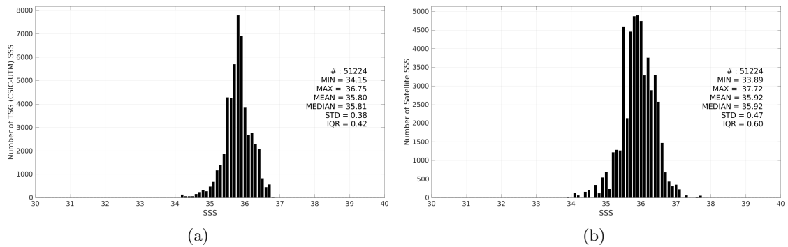
Figure 3: Histograms of SSS from TSG (CSIC-UTM) (a) and SMAP SSS L2 v6 (RSS) (b) considering all match-up pairs per bins of 0.1 over the Equatorial Ocean 10N-10S Pi-MEP region and for the full satellite product period.
