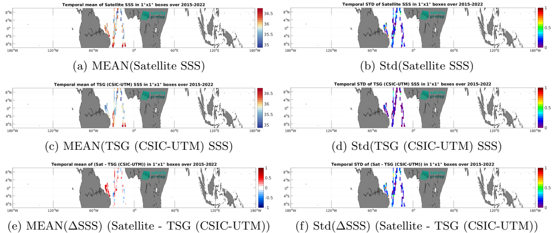
Figure 7: Temporal mean (left) and Std (right) of SSS from SMAP SSS L2 v6 (RSS) (top), TSG (CSIC-UTM) (middle), and of \Delta SSS (Satellite - TSG (CSIC-UTM)). Only match-up pairs are used to generate these maps.
