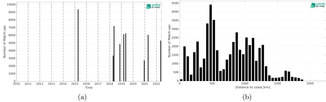
Figure 2: Number of match-ups between TSG (CSIC-UTM) and SMAP SSS L2 v6 (RSS) SSS as a function of time (a) and as function of the distance to coast (b) over the Equatorial Ocean 10N-10S Pi-MEP region and for the full satellite product period.
