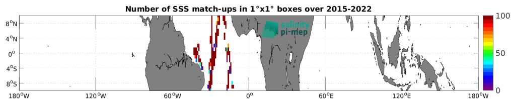
Figure 5: Number of SSS match-ups between TSG (CSIC-UTM) SSS and the SMAP SSS L2 v6 (RSS) SSS product for the Equatorial Ocean 10N-10S Pi-MEP region over 1^\circ \times 1^\circ boxes and for the full satellite product period.
