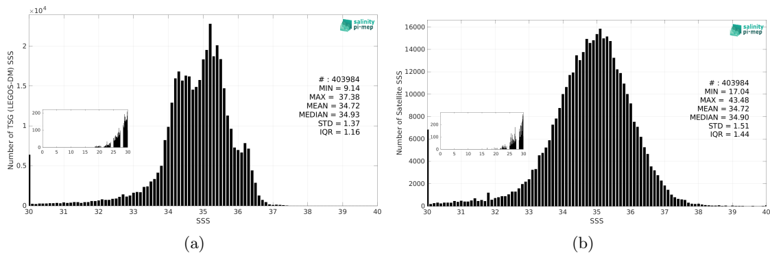
Figure 3: Histograms of SSS from TSG (LEGOS-DM) (a) and SMAP SSS L2 v6 - 40 km (RSS) (b) considering all match-up pairs per bins of 0.1 over the Equatorial Ocean 10N-10S Pi-MEP region and for the full satellite product period.
