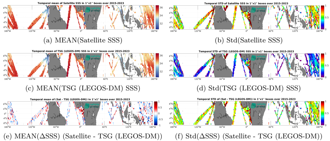
Figure 7: Temporal mean (left) and Std (right) of SSS from SMAP SSS L2 v6 - 40 km (RSS) (top), TSG (LEGOS-DM) (middle), and of \Delta SSS (Satellite - TSG (LEGOS-DM)). Only match-up pairs are used to generate these maps.
