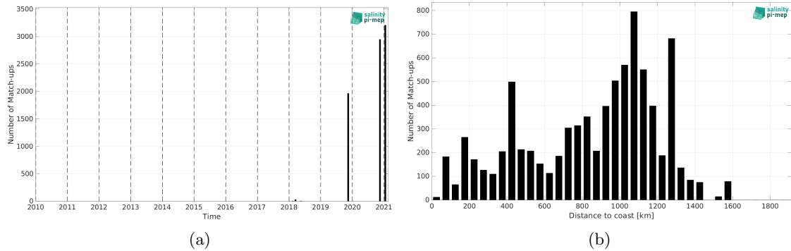
Figure 2: Number of match-ups between TSG (GOSUD-Sailing-ship) and SMAP SSS L2 v6 - 40 km (RSS) SSS as a function of time (a) and as function of the distance to coast (b) over the Equatorial Ocean 10N-10S Pi-MEP region and for the full satellite product period.
