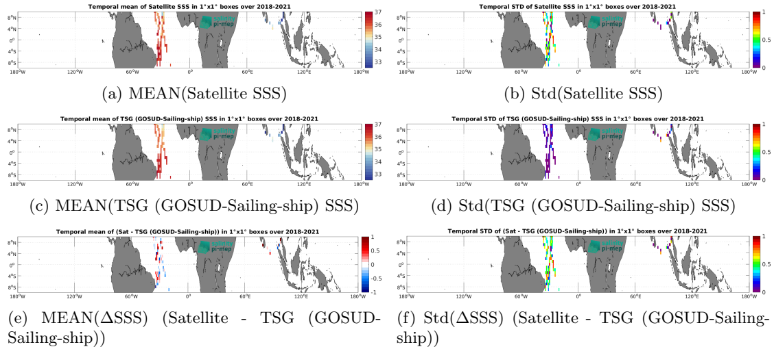
Figure 7: Temporal mean (left) and Std (right) of SSS from SMAP SSS L2 v6 - 40 km (RSS) (top), TSG (GOSUD-Sailing-ship) (middle), and of \Delta SSS (Satellite - TSG (GOSUD-Sailing-ship)). Only match-up pairs are used to generate these maps.
