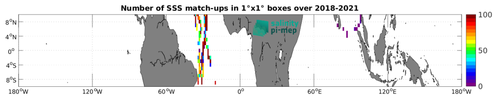
Figure 5: Number of SSS match-ups between TSG (GOSUD-Sailing-ship) SSS and the SMAP SSS L2 v6 - 40 km (RSS) SSS product for the Equatorial Ocean 10N-10S Pi-MEP region over 1^\circ \times 1^\circ boxes and for the full satellite product period.
