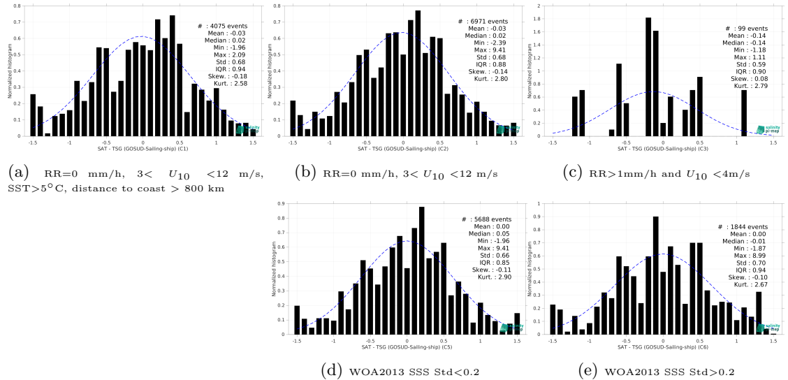
Figure 15: Normalized histogram of \Delta SSS (SMAP SSS L2 v6 - 40 km (RSS) - TSG (GOSUD-Sailing-ship)) for 5 different subdatasets corresponding to: RR=0 mm/h, 3 < U_{10} < 12 m/s, SST>5°C, distance to coast > 800 km (a), RR=0 mm/h, 3 < U_{10} < 12 m/s (b), RR>1mm/h and U_{10} < 4 m/s (c), WOA2013 SSS Std<0.2 (d), WOA2013 SSS Std>0.2 (e).
