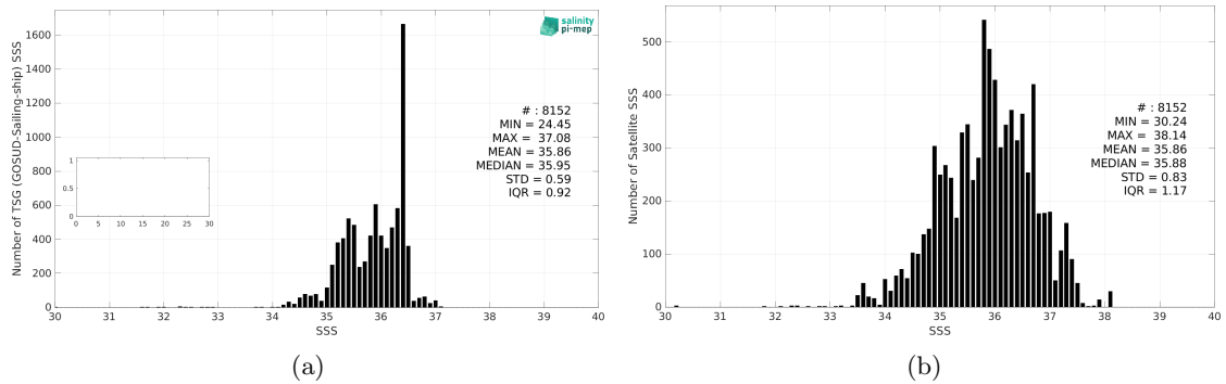
Figure 3: Histograms of SSS from TSG (GOSUD-Sailing-ship) (a) and SMAP SSS L2 v6 - 40 km (RSS) (b) considering all match-up pairs per bins of 0.1 over the Equatorial Ocean 10N-10S Pi-MEP region and for the full satellite product period.
