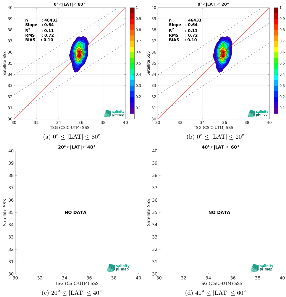
Figure 10: Contour maps of the concentration of SMAP SSS L2 v6 - 40 km (RSS) SSS (y-axis) versus TSG (CSIC-UTM) SSS (x-axis) at match-up pairs for different latitude bands. For each plot, the red line shows x=y . The black thin and dashed lines indicate a linear fit through the data cloud and the \pm 95\% confidence levels, respectively. The number match-up pairs n , the slope and R^2 coefficient of the linear fit, the root mean square (RMS) and the mean bias between satellite and in situ data are indicated for each latitude band in each plots.
