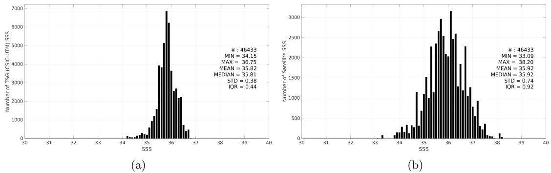
Figure 3: Histograms of SSS from TSG (CSIC-UTM) (a) and SMAP SSS L2 v6 - 40 km (RSS) (b) considering all match-up pairs per bins of 0.1 over the Equatorial Ocean 10N-10S Pi-MEP region and for the full satellite product period.
