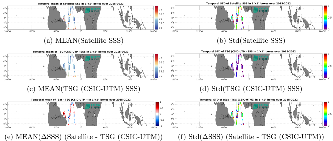
Figure 7: Temporal mean (left) and Std (right) of SSS from SMAP SSS L2 v6 - 40 km (RSS) (top), TSG (CSIC-UTM) (middle), and of \Delta SSS (Satellite - TSG (CSIC-UTM)). Only match-up pairs are used to generate these maps.
