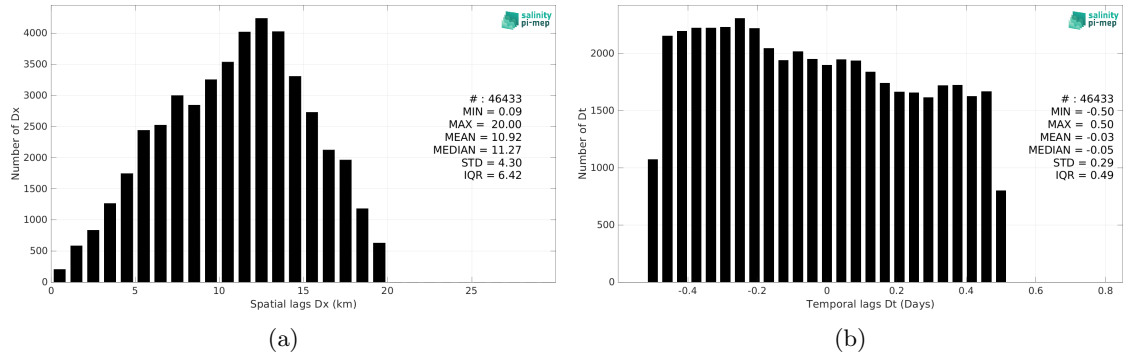
Figure 6: Histograms of the spatial (a) and temporal (b) lags between the location/time of the TSG (CSIC-UTM) measurement and the date of the corresponding SMAP SSS L2 v6 - 40 km (RSS) SSS pixel.
