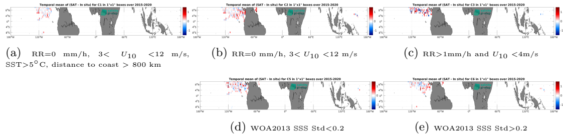
Figure 13: Temporal mean gridded over spatial boxes of size 1^\circ \times 1^\circ of \Delta\text{SSS} (SMAP SSS L2 v6 - 40 km (RSS) - Surface drifters) for 5 different subdatasets corresponding to:RR=0 mm/h, 3 < U_{10} < 12 m/s, SST >5^\circ\text{C} , distance to coast > 800 km (a), RR=0 mm/h, 3 < U_{10} < 12 m/s (b), RR >1 mm/h and U_{10} < 4 m/s (c), WOA2013 SSS Std <0.2 (d), WOA2013 SSS Std >0.2 (e).
