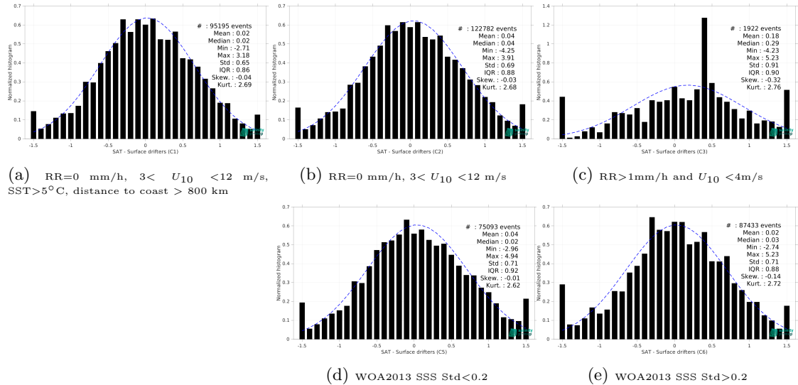
Figure 14: Normalized histogram of \Delta\text{SSS} (SMAP SSS L2 v6 - 40 km (RSS) - Surface drifters) for 5 different subdatasets corresponding to: RR=0 mm/h, 3 < U_{10} < 12 m/s, SST >5^\circ\text{C} , distance to coast > 800 km (a), RR=0 mm/h, 3 < U_{10} < 12 m/s (b), RR >1 mm/h and U_{10} < 4 m/s (c), WOA2013 SSS Std <0.2 (d), WOA2013 SSS Std >0.2 (e).
