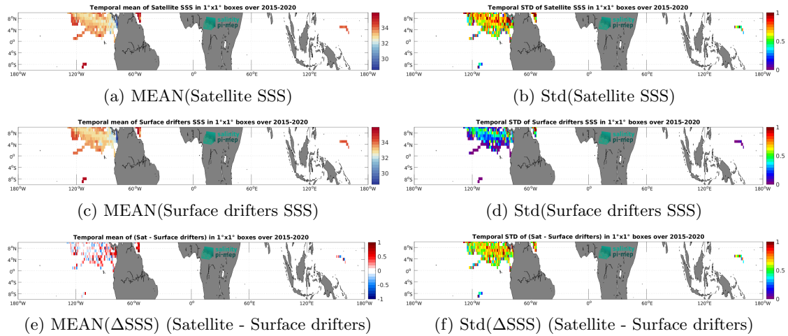
Figure 6: Temporal mean (left) and Std (right) of SSS from SMAP SSS L2 v6 - 40 km (RSS) (top), Surface drifters (middle), and of \Delta SSS (Satellite - Surface drifters). Only match-up pairs are used to generate these maps.
