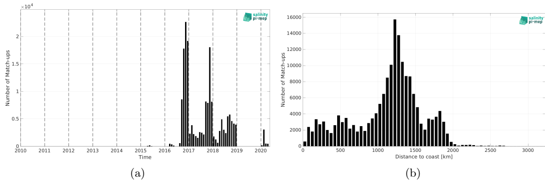
Figure 2: Number of match-ups between Surface drifters and SMAP SSS L2 v6 - 40 km (RSS) SSS as a function of time (a) and as function of the distance to coast (b) over the Equatorial Ocean 10N-10S Pi-MEP region and for the full satellite product period.
