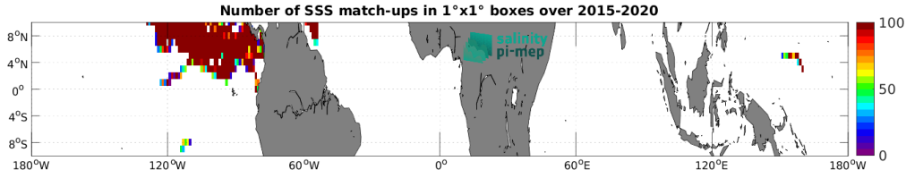
Figure 4: Number of SSS match-ups between Surface drifters SSS and the SMAP SSS L2 v6 - 40 km (RSS) SSS product for the Equatorial Ocean 10N-10S Pi-MEP region over 1^\circ \times 1^\circ boxes and for the full satellite product period.
