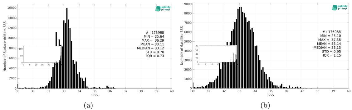
Figure 3: Histograms of SSS from Surface drifters (a) and SMAP SSS L2 v6 - 40 km (RSS) (b) considering all match-up pairs per bins of 0.1 over the Equatorial Ocean 10N-10S Pi-MEP region and for the full satellite product period.
