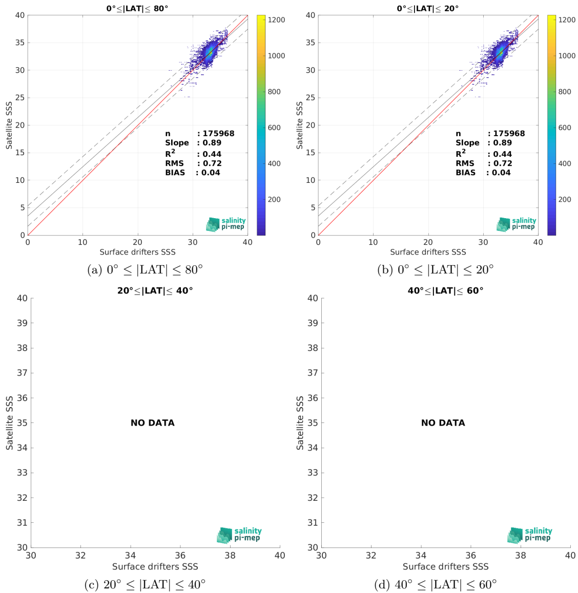
Figure 9: Contour maps of the concentration of SMAP SSS L2 v6 - 40 km (RSS) SSS (y-axis) versus Surface drifters SSS (x-axis) at match-up pairs for different latitude bands. For each plot, the red line shows x=y . The black thin and dashed lines indicate a linear fit through the data cloud and the \pm 95\% confidence levels, respectively. The number match-up pairs n , the slope and R^2 coefficient of the linear fit, the root mean square (RMS) and the mean bias between satellite and in situ data are indicated for each latitude band in each plots.
