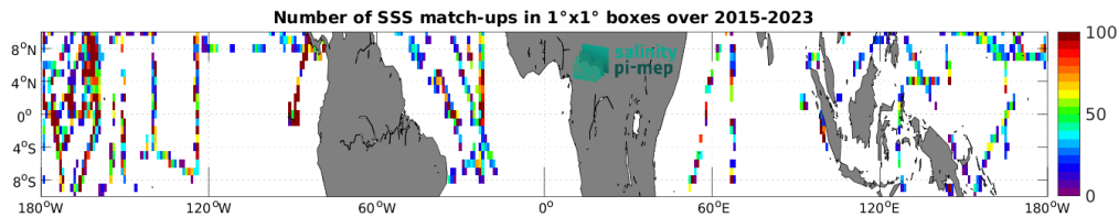
Figure 4: Number of SSS match-ups between TSG (SAMOS) SSS and the SMAP SSS L2 v5 (RSS) SSS product for the Equatorial Ocean 10N-10S Pi-MEP region over 1^\circ \times 1^\circ boxes and for the full satellite product period.
