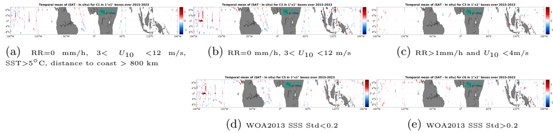
Figure 12: Temporal mean gridded over spatial boxes of size 1^\circ \times 1^\circ of \Delta SSS (SMAP SSS L2 v5 (RSS) - TSG (SAMOS)) for 5 different subdatasets corresponding to:RR=0 mm/h, 3 < U_{10} < 12 m/s, SST>5°C, distance to coast > 800 km (a), RR=0 mm/h, 3 < U_{10} < 12 m/s (b), RR>1mm/h and U_{10} < 4 m/s (c), WOA2013 SSS Std<0.2 (d), WOA2013 SSS Std>0.2 (e).
