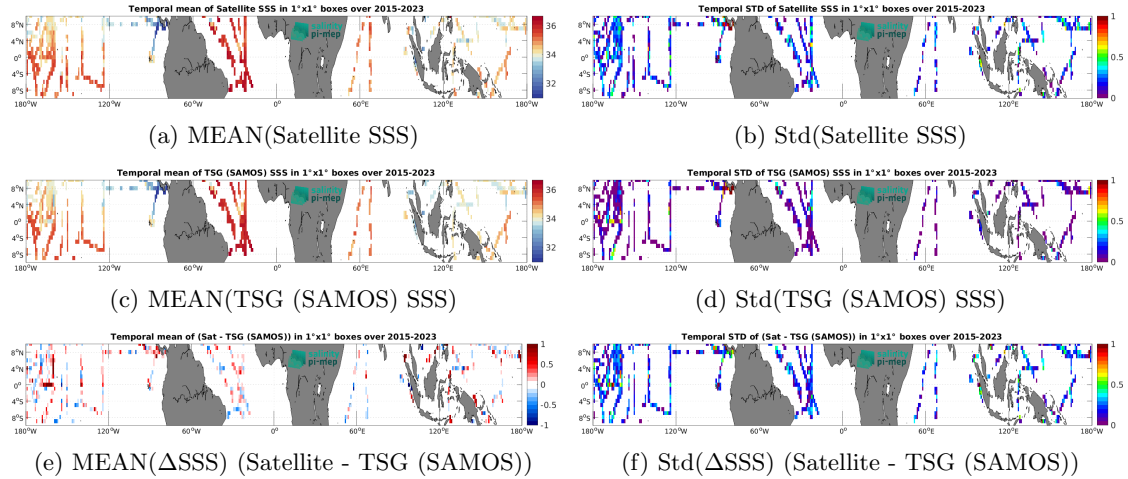
Figure 6: Temporal mean (left) and Std (right) of SSS from SMAP SSS L2 v5 (RSS) (top), TSG (SAMOS) (middle), and of \Delta SSS (Satellite - TSG (SAMOS)). Only match-up pairs are used to generate these maps.
