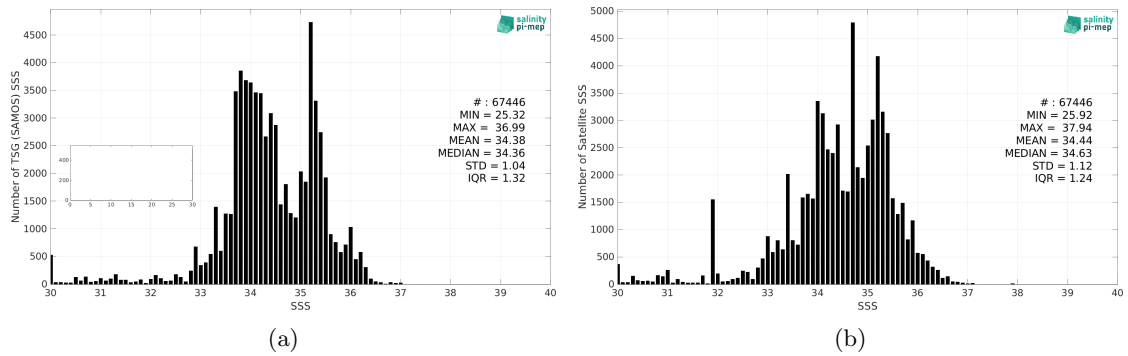
Figure 2: Histograms of SSS from TSG (SAMOS) (a) and SMAP SSS L2 v5 (RSS) (b) considering all match-up pairs per bins of 0.1 over the Equatorial Ocean 10N-10S Pi-MEP region and for the full satellite product period.
