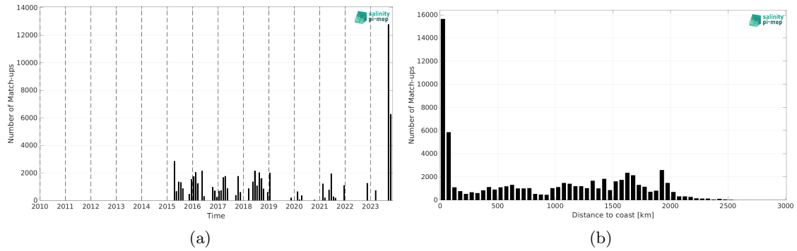
Figure 1: Number of match-ups between TSG (SAMOS) and SMAP SSS L2 v5 (RSS) SSS as a function of time (a) and as function of the distance to coast (b) over the Equatorial Ocean 10N-10S Pi-MEP region and for the full satellite product period.
