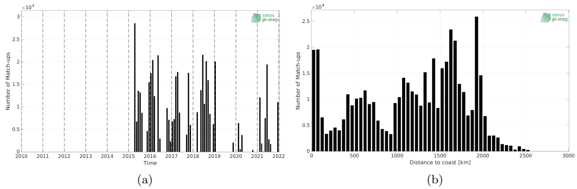
Figure 1: Number of match-ups between TSG (SAMOS) and SMAP SSS L2 v5 (RSS) SSS as a function of time (a) and as function of the distance to coast (b) over the Equatorial Ocean 10N-10S Pi-MEP region and for the full satellite product period.
