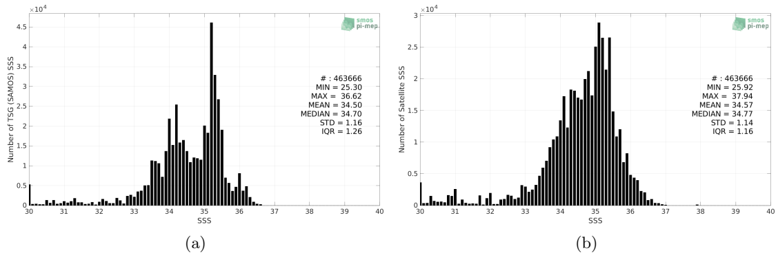
Figure 2: Histograms of SSS from TSG (SAMOS) (a) and SMAP SSS L2 v5 (RSS) (b) considering all match-up pairs per bins of 0.1 over the Equatorial Ocean 10N-10S Pi-MEP region and for the full satellite product period.
