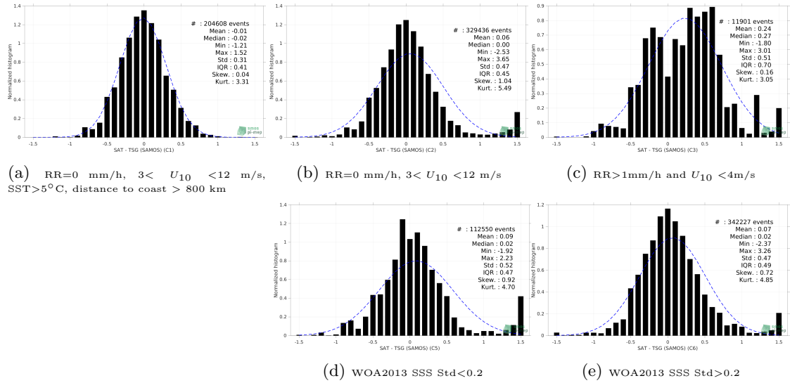
Figure 13: Normalized histogram of \Delta SSS (SMAP SSS L2 v5 (RSS) - TSG (SAMOS)) for 5 different subdatasets corresponding to: RR=0 mm/h, 3 < U_{10} < 12 m/s, SST >5^\circ\text{C} , distance to coast > 800 km (a), RR=0 mm/h, 3 < U_{10} < 12 m/s (b), RR >1 mm/h and U_{10} < 4 m/s (c), WOA2013 SSS Std <0.2 (d), WOA2013 SSS Std >0.2 (e).
