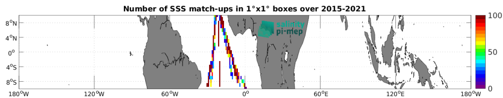
Figure 4: Number of SSS match-ups between TSG (Polarstern) SSS and the SMAP SSS L2 v5 (RSS) SSS product for the Equatorial Ocean 10N-10S Pi-MEP region over 1^\circ \times 1^\circ boxes and for the full satellite product period.
