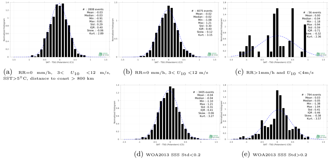
Figure 13: Normalized histogram of \Delta SSS (SMAP SSS L2 v5 (RSS) - TSG (Polarstern)) for 5 different subdatasets corresponding to: RR=0 mm/h, 3 < U_{10} < 12 m/s, SST >5^\circ C, distance to coast > 800 km (a), RR=0 mm/h, 3 < U_{10} < 12 m/s (b), RR >1 mm/h and U_{10} < 4 m/s (c), WOA2013 SSS Std <0.2 (d), WOA2013 SSS Std >0.2 (e).
