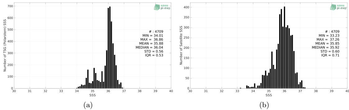
Figure 2: Histograms of SSS from TSG (Polarstern) (a) and SMAP SSS L2 v5 (RSS) (b) considering all match-up pairs per bins of 0.1 over the Equatorial Ocean 10N-10S Pi-MEP region and for the full satellite product period.
