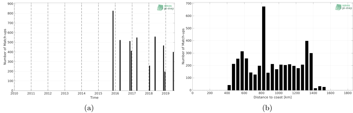
Figure 1: Number of match-ups between TSG (Polarstern) and SMAP SSS L2 v5 (RSS) SSS as a function of time (a) and as function of the distance to coast (b) over the Equatorial Ocean 10N-10S Pi-MEP region and for the full satellite product period.
