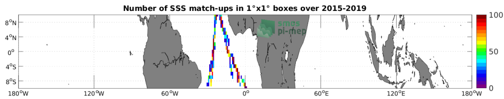
Figure 4: Number of SSS match-ups between TSG (Polarstern) SSS and the SMAP SSS L2 v5 (RSS) SSS product for the Equatorial Ocean 10N-10S Pi-MEP region over 1^\circ \times 1^\circ boxes and for the full satellite product period.
