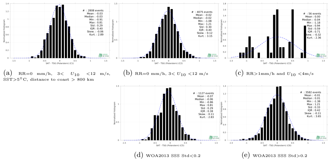
Figure 13: Normalized histogram of \Delta SSS (SMAP SSS L2 v5 (RSS) - TSG (Polarstern)) for 5 different subdatasets corresponding to: RR=0 mm/h, 3 < U_{10} < 12 m/s, SST >5^\circ\text{C} , distance to coast > 800 km (a), RR=0 mm/h, 3 < U_{10} < 12 m/s (b), RR >1 mm/h and U_{10} < 4 m/s (c), WOA2013 SSS Std <0.2 (d), WOA2013 SSS Std >0.2 (e).
