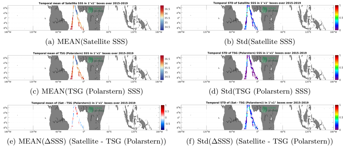
Figure 6: Temporal mean (left) and Std (right) of SSS from SMAP SSS L2 v5 (RSS) (top), TSG (Polarstern) (middle), and of \Delta SSS (Satellite - TSG (Polarstern)). Only match-up pairs are used to generate these maps.
