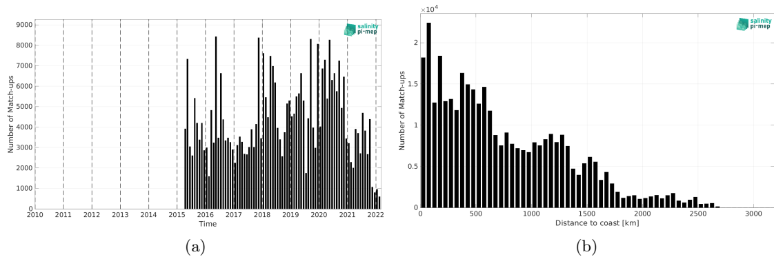
Figure 1: Number of match-ups between TSG (LEGOS-DM) and SMAP SSS L2 v5 (RSS) SSS as a function of time (a) and as function of the distance to coast (b) over the Equatorial Ocean 10N-10S Pi-MEP region and for the full satellite product period.
