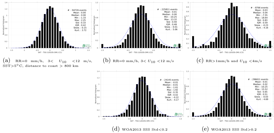
Figure 13: Normalized histogram of \Delta SSS (SMAP SSS L2 v5 (RSS) - TSG (LEGOS-DM)) for 5 different subdatasets corresponding to: RR=0 mm/h, 3 < U_{10} < 12 m/s, SST > 5^\circ C , distance to coast > 800 km (a), RR=0 mm/h, 3 < U_{10} < 12 m/s (b), RR>1mm/h and U_{10} < 4 m/s (c), WOA2013 SSS Std<0.2 (d), WOA2013 SSS Std>0.2 (e).
