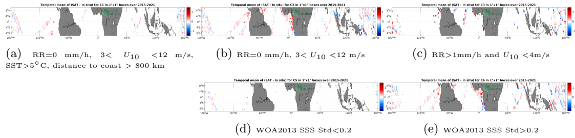
Figure 12: Temporal mean gridded over spatial boxes of size 1^\circ \times 1^\circ of \Delta SSS (SMAP SSS L2 v5 (RSS) - TSG (LEGOS-DM)) for 5 different subdatasets corresponding to: RR=0 mm/h, 3 < U_{10} < 12 m/s, SST > 5^\circ C , distance to coast > 800 km (a), RR=0 mm/h, 3 < U_{10} < 12 m/s (b), RR>1mm/h and U_{10} < 4 m/s (c), WOA2013 SSS Std<0.2 (d), WOA2013 SSS Std>0.2 (e).
