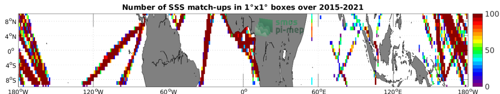
Figure 4: Number of SSS match-ups between TSG (LEGOS-DM) SSS and the SMAP SSS L2 v5 (RSS) SSS product for the Equatorial Ocean 10N-10S Pi-MEP region over 1^\circ \times 1^\circ boxes and for the full satellite product period.
