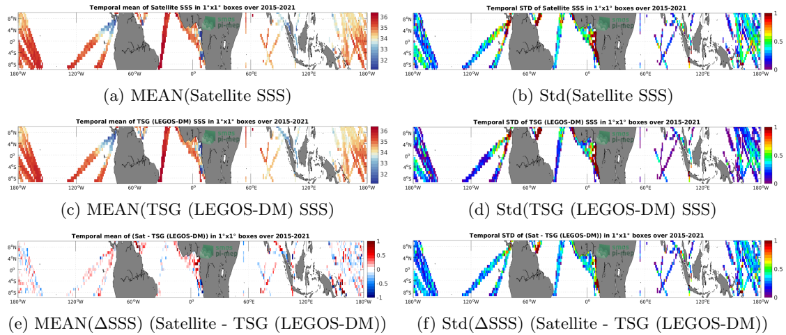
Figure 6: Temporal mean (left) and Std (right) of SSS from SMAP SSS L2 v5 (RSS) (top), TSG (LEGOS-DM) (middle), and of \Delta SSS (Satellite - TSG (LEGOS-DM)). Only match-up pairs are used to generate these maps.
