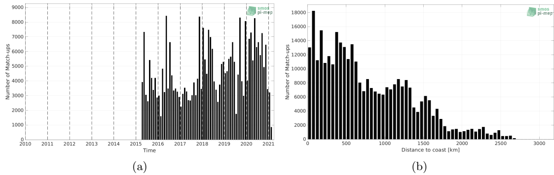
Figure 1: Number of match-ups between TSG (LEGOS-DM) and SMAP SSS L2 v5 (RSS) SSS as a function of time (a) and as function of the distance to coast (b) over the Equatorial Ocean 10N-10S Pi-MEP region and for the full satellite product period.
