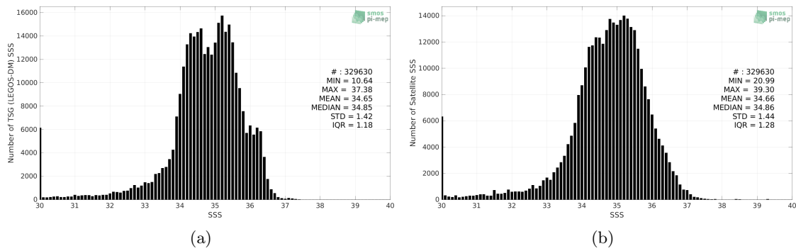
Figure 2: Histograms of SSS from TSG (LEGOS-DM) (a) and SMAP SSS L2 v5 (RSS) (b) considering all match-up pairs per bins of 0.1 over the Equatorial Ocean 10N-10S Pi-MEP region and for the full satellite product period.
