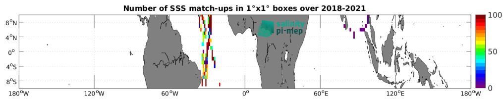
Figure 4: Number of SSS match-ups between TSG (GOSUD-Sailing-ship) SSS and the SMAP SSS L2 v5 (RSS) SSS product for the Equatorial Ocean 10N-10S Pi-MEP region over 1^\circ \times 1^\circ boxes and for the full satellite product period.
