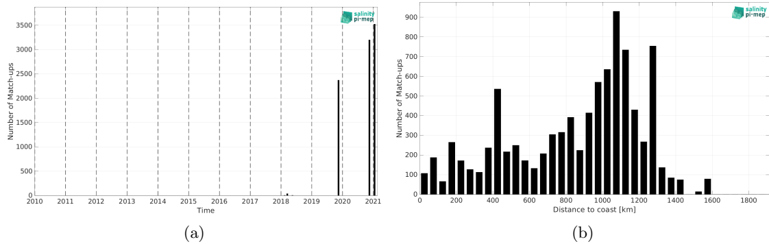
Figure 1: Number of match-ups between TSG (GOSUD-Sailing-ship) and SMAP SSS L2 v5 (RSS) SSS as a function of time (a) and as function of the distance to coast (b) over the Equatorial Ocean 10N-10S Pi-MEP region and for the full satellite product period.
