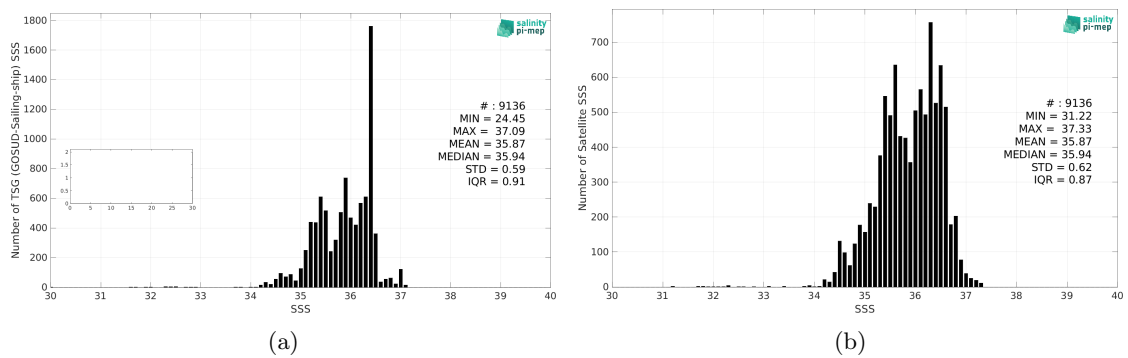
Figure 2: Histograms of SSS from TSG (GOSUD-Sailing-ship) (a) and SMAP SSS L2 v5 (RSS) (b) considering all match-up pairs per bins of 0.1 over the Equatorial Ocean 10N-10S Pi-MEP region and for the full satellite product period.
