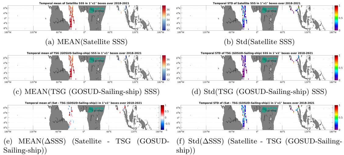
Figure 6: Temporal mean (left) and Std (right) of SSS from SMAP SSS L2 v5 (RSS) (top), TSG (GOSUD-Sailing-ship) (middle), and of \Delta SSS (Satellite - TSG (GOSUD-Sailing-ship)). Only match-up pairs are used to generate these maps.
